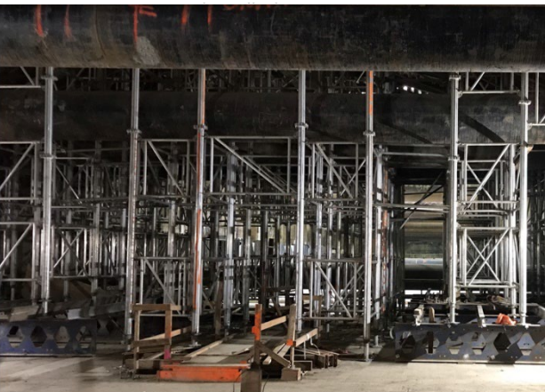
Falsework removal at the WRS Station Box
