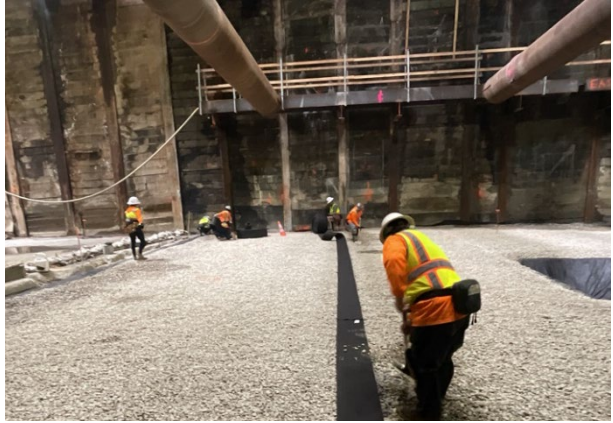
Excavation, Lagging Storm Drain Relocation, and Concrete Slab Preparation Progress at Century City
