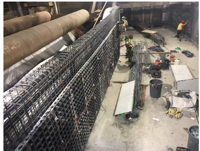
South Beverly Appendage Exterior Walls
