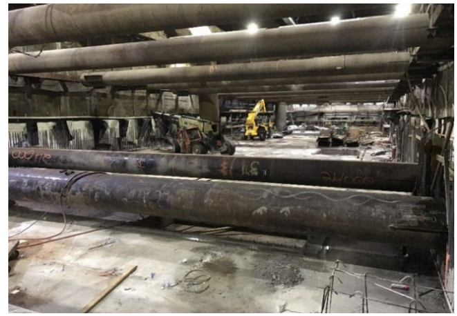
WRS East Concourse Level Strut Removal
