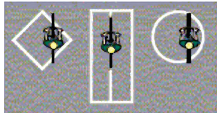
This diagram shows the bike-sensitive portion of different loop detectors
