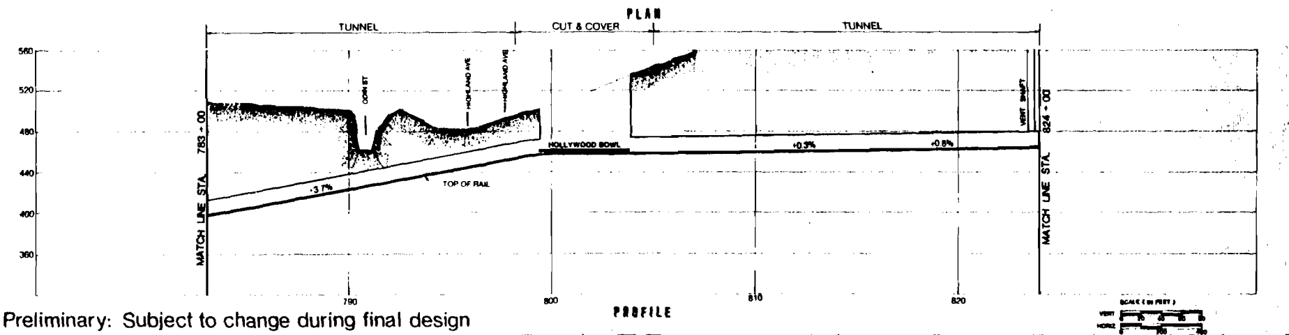
Figure 2-4.15 Alignment for Locally Preferred Alternative
