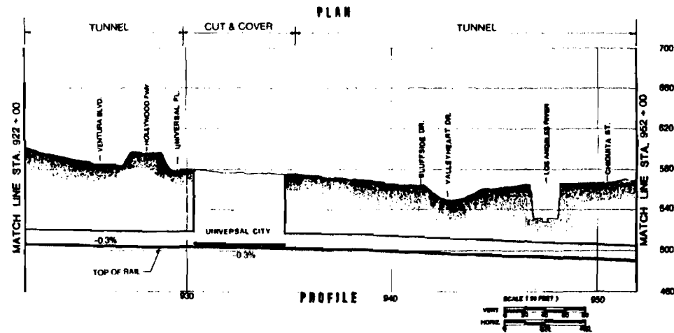
Figure 2-4.18 Alignment for Locally Preferred Alternative
