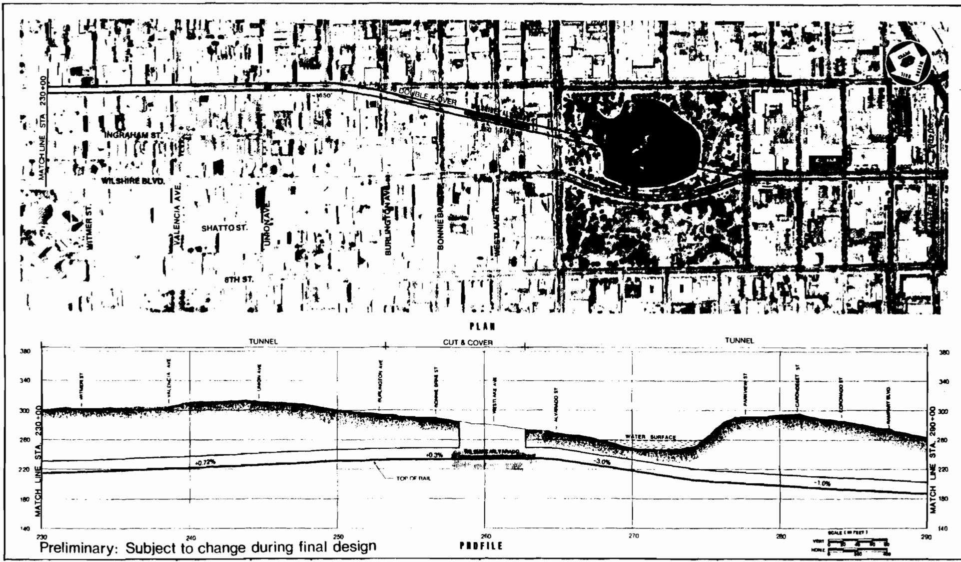
Figure 2-4.4 Alignment for Locally Preferred Alternative
