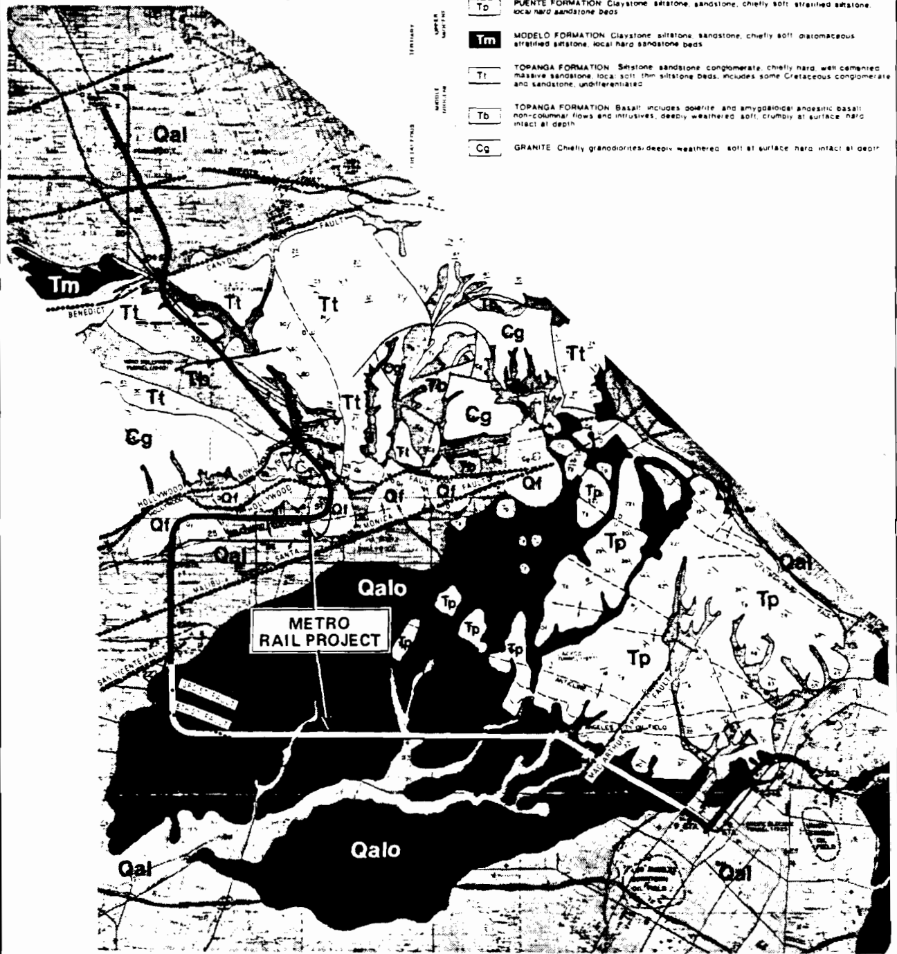
Figure 3-18 Local Geology
