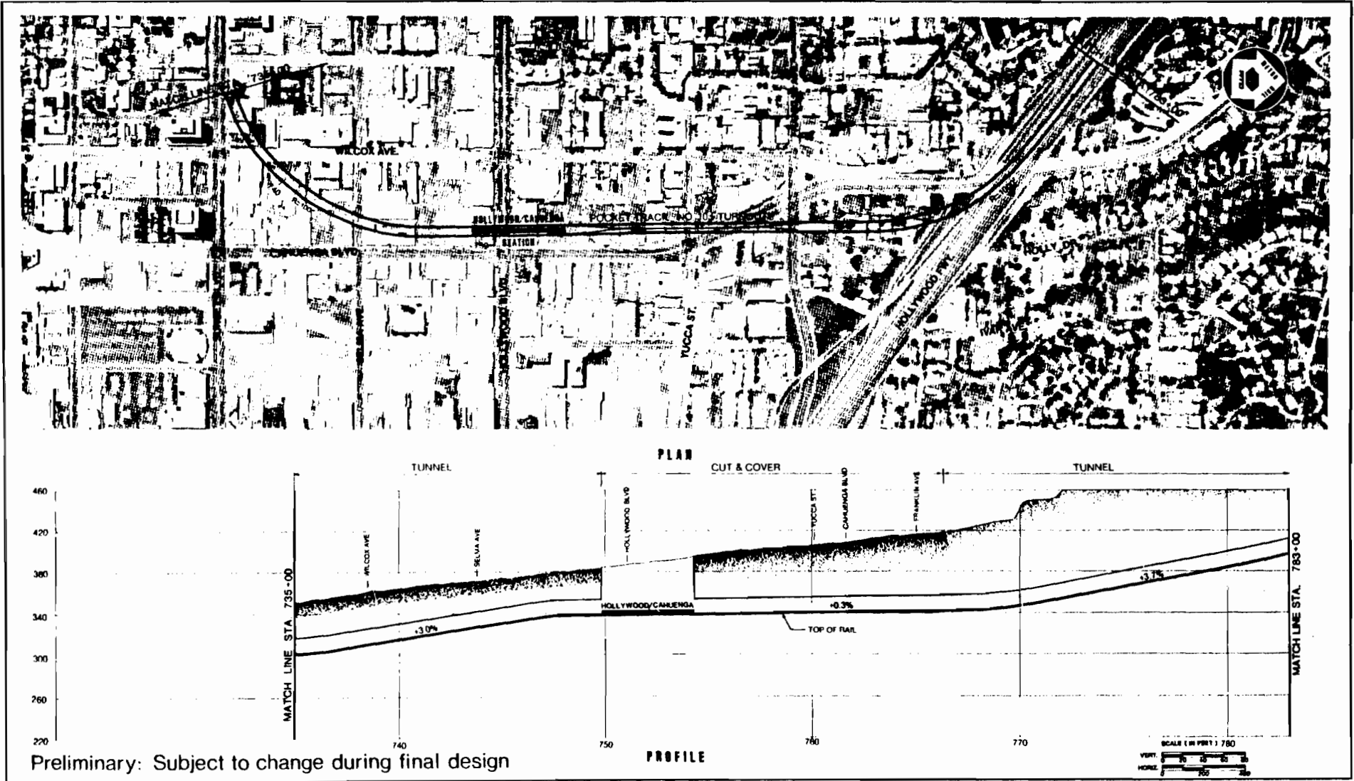
Figure 2-4.14 Alignment for Locally Preferred Alternative
