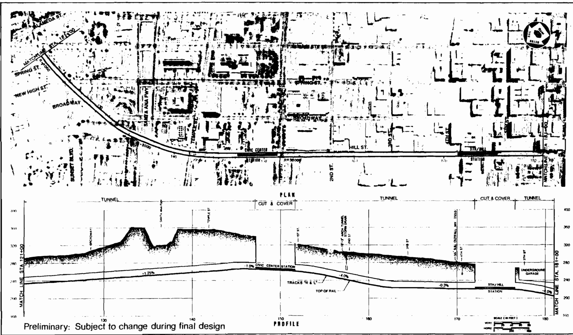
Figure 2-4.2 Alignment for Locally Preferred Alternative
