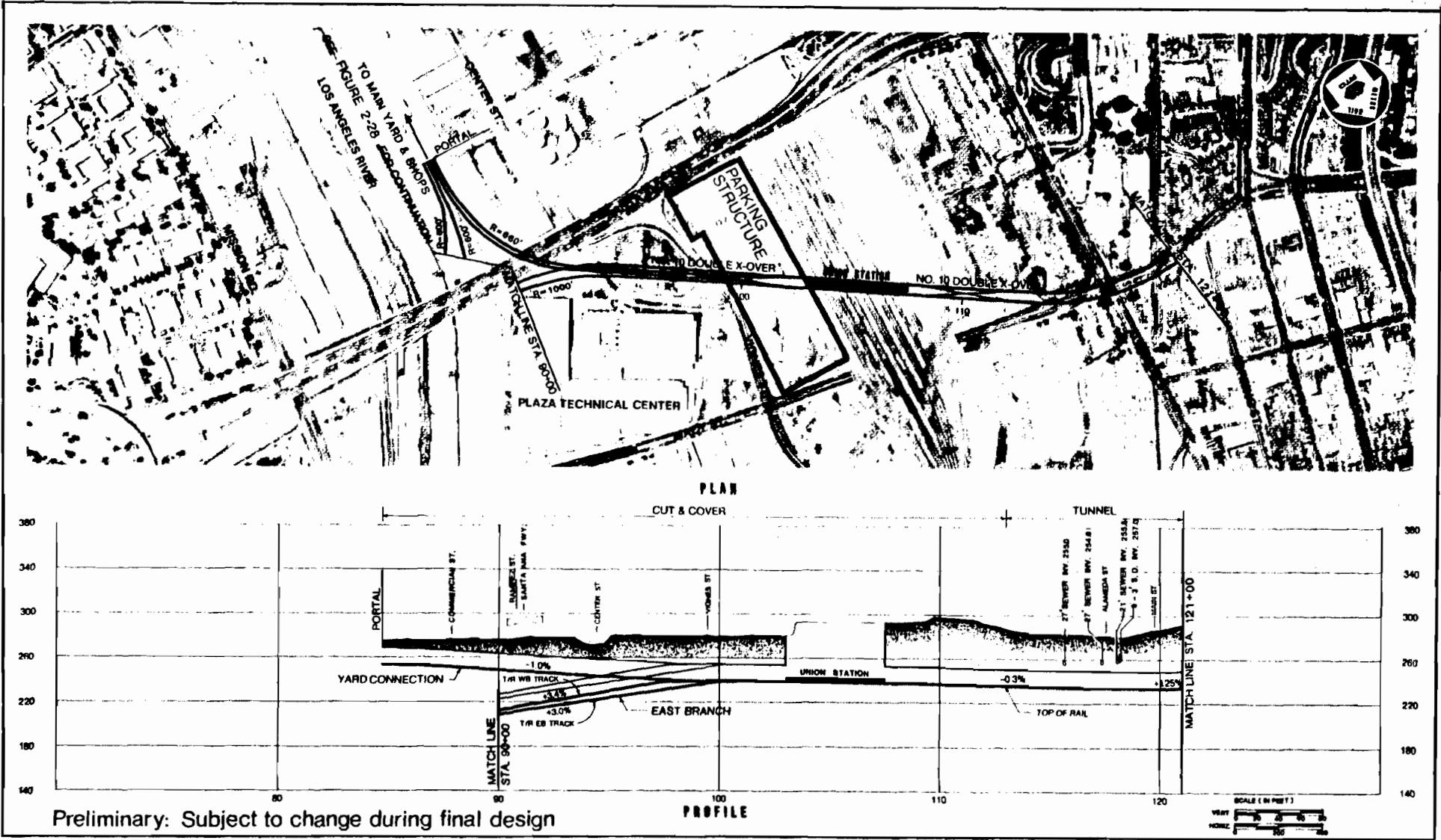
Southern California Rapid Transit District Metro Rail Project PRELIMINARY ENGINEERING PROGRAM Figure 2-4.1 Alignment for Locally Preferred Alternative Source: DMJM/PBQD
