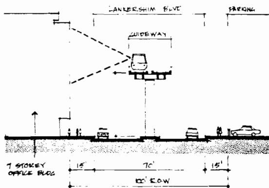
Lankershim Blvd. north of Ventura Freeway. Section looking south. 10 15 30 60 feet
