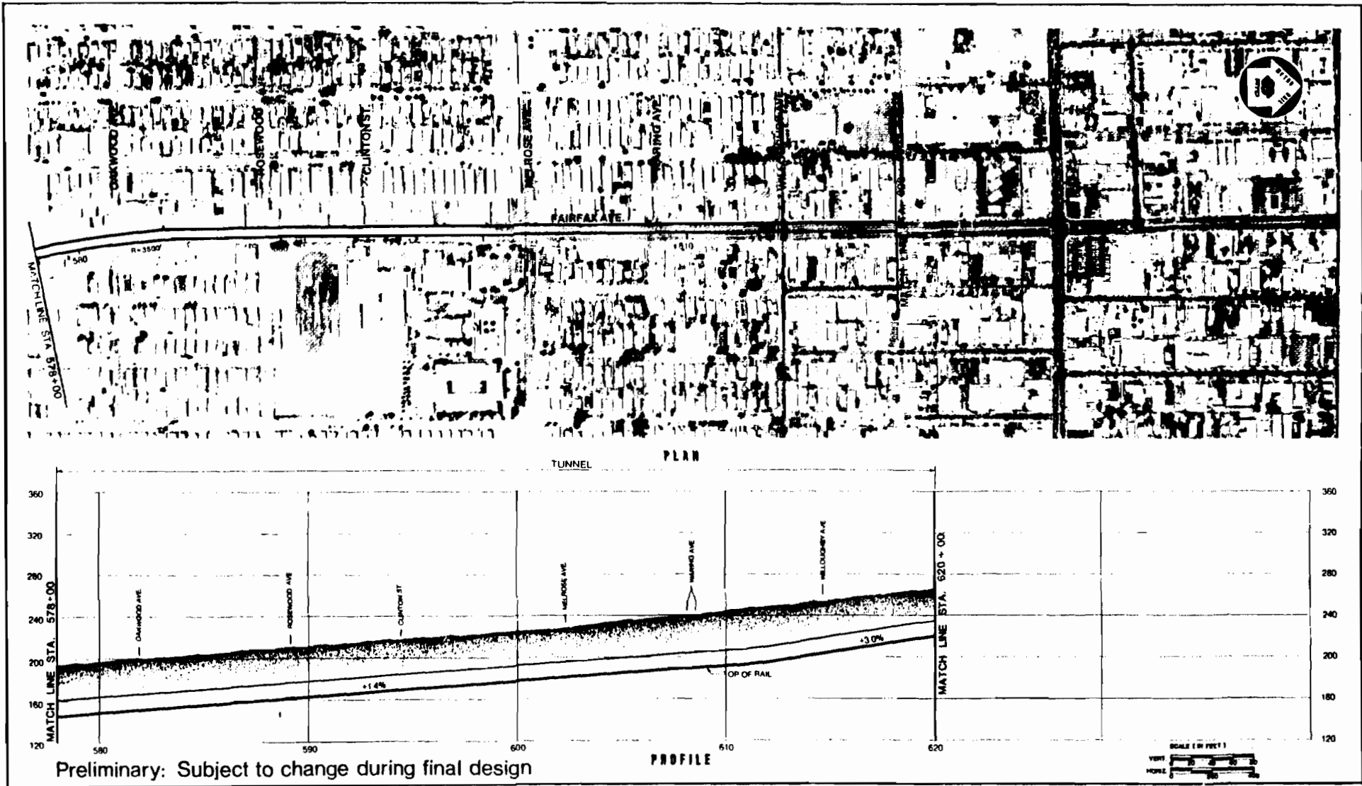
Figure 2-4.10 Alignment for Locally Preferred Alternative
