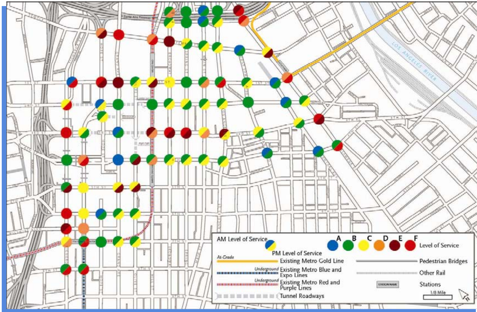
Figure 1-8. Predicted Level of Service in Project Area Without Transit Improvements (2035)
