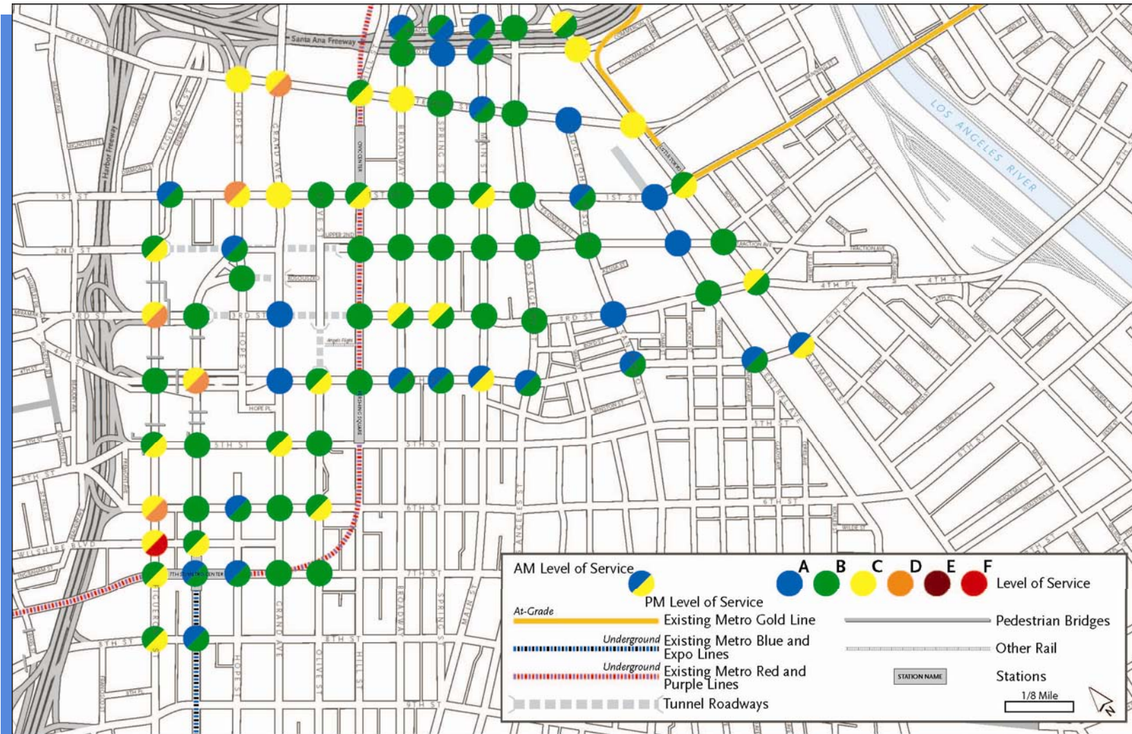
Figure 1-7. Existing Level of Service in Project Area
