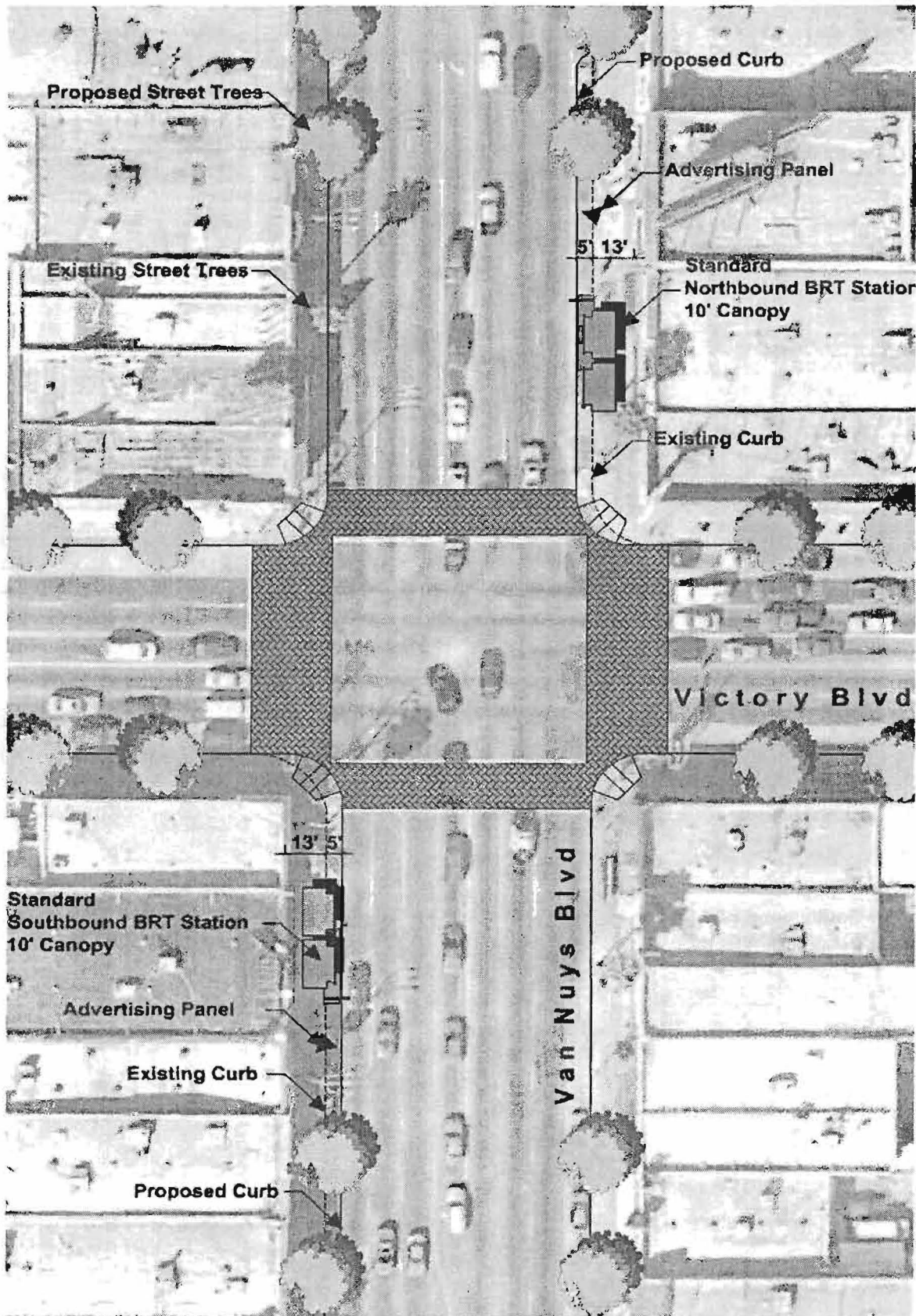
Figure 4-37. Site Plan of On-Street Station along Van Nuys Boulevard at Victory Boulevard source: Gruen Associates
