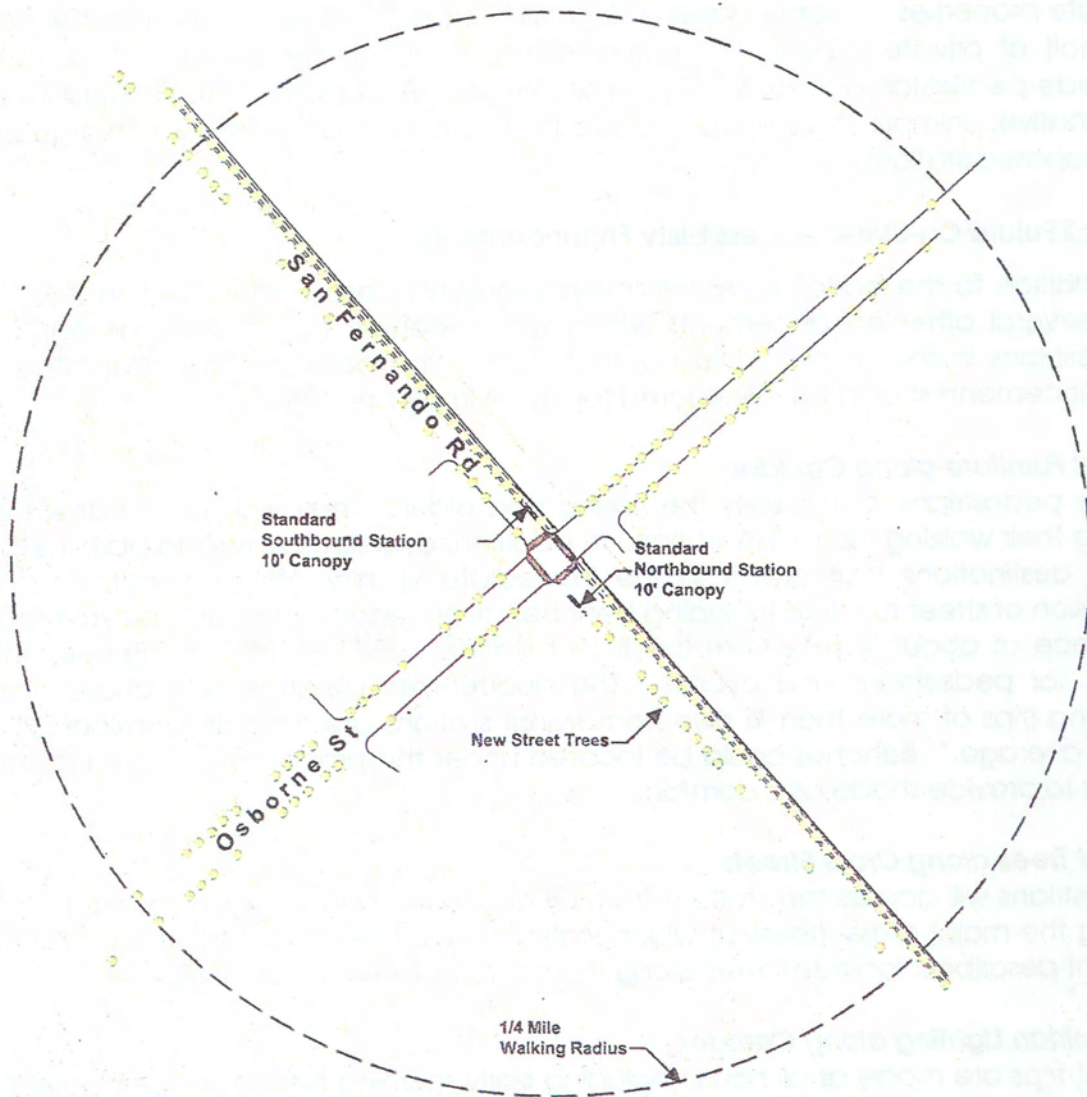
Figure 4-23. Typical Plan of Tree Planting Within 1/4 Mile of Station (San Fernando / Osborne Station)
