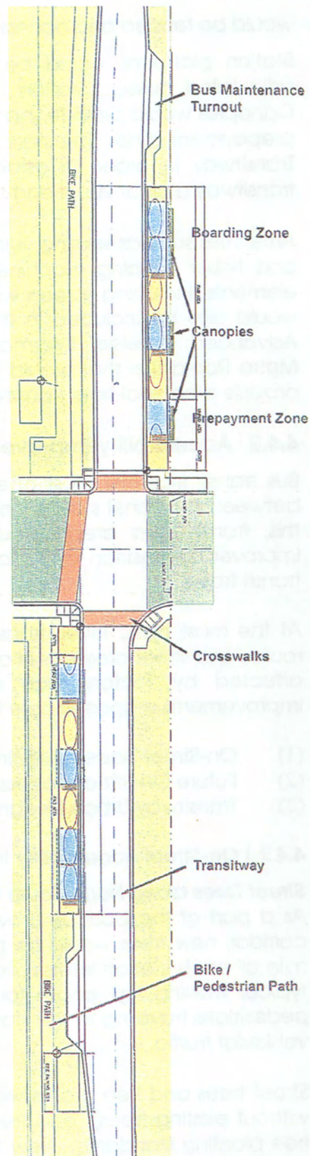
Figure 4-22. Typical Transitway Station
