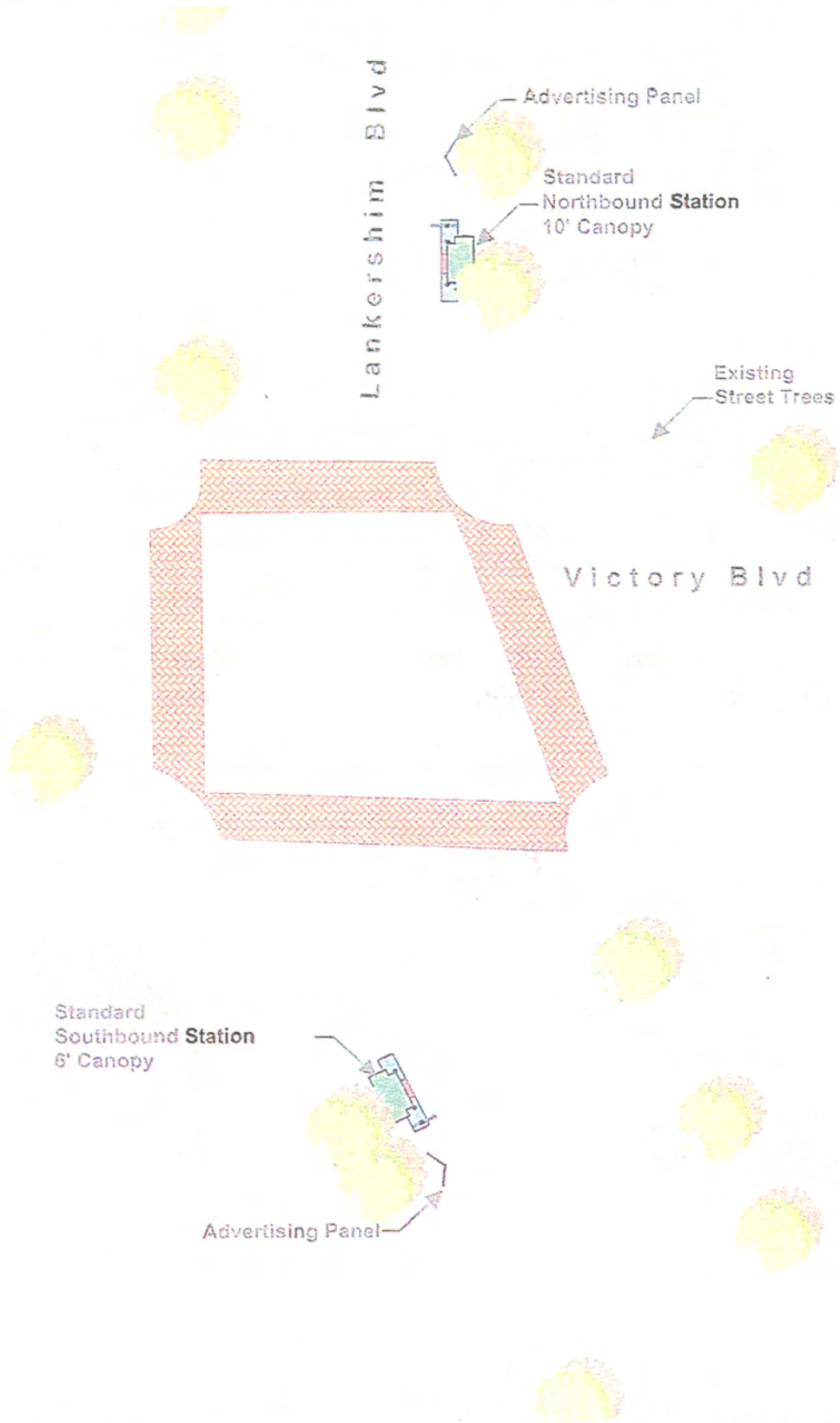
Figure 4-41. Site Plan of On-Street Station along Lankershim Boulevard at Victory Boulevard
