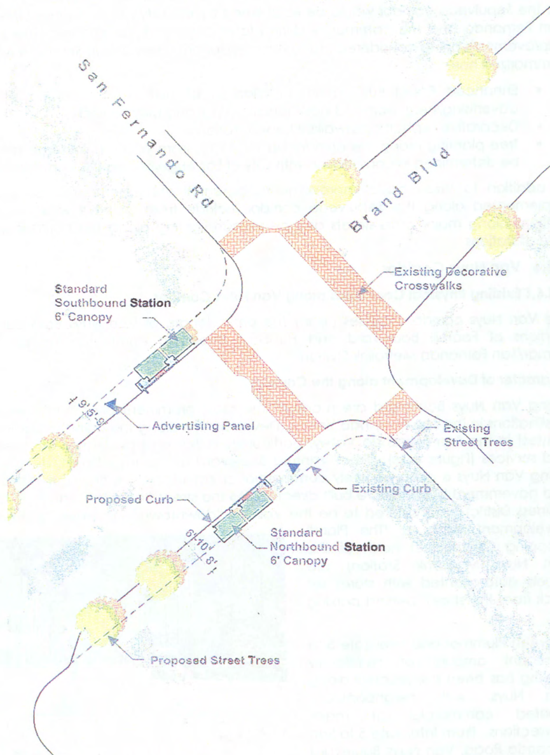
Figure 4-35. Site Plan of On-Street Station along Brand Boulevard and San Fernando Road, Sepulveda Corridor
