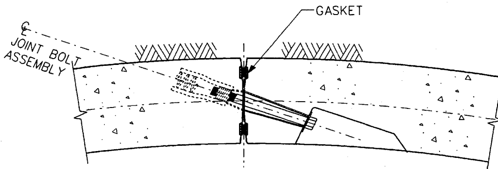
Figure 1 Double Gasket Liner
