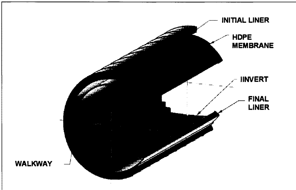
Figure C-5 Tunnel Liners and Membrane Orientation
