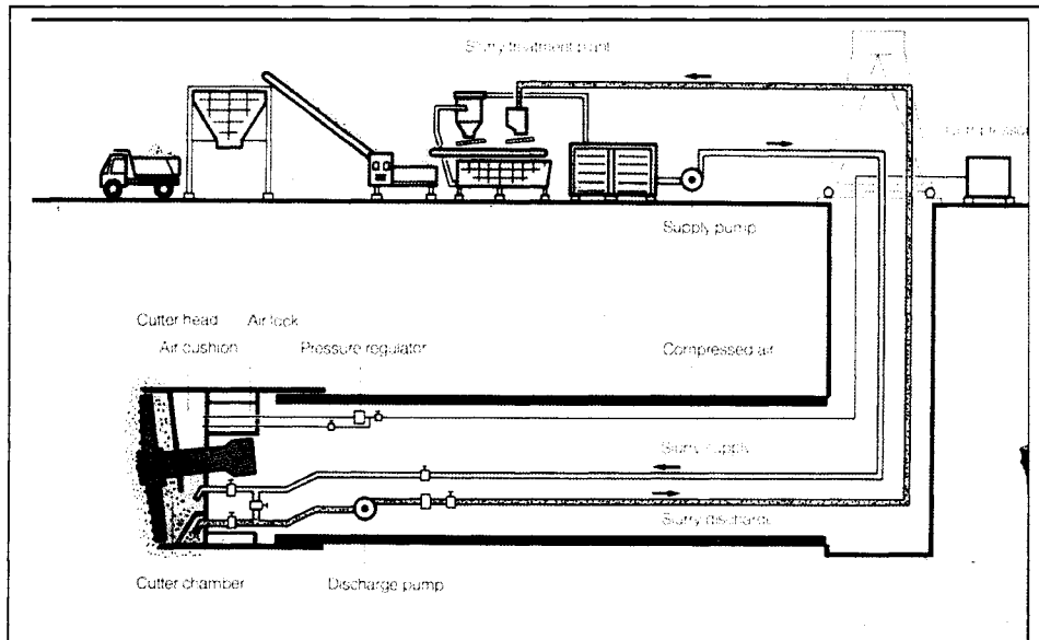
Figure C-2 Slurry Material Conveyance
