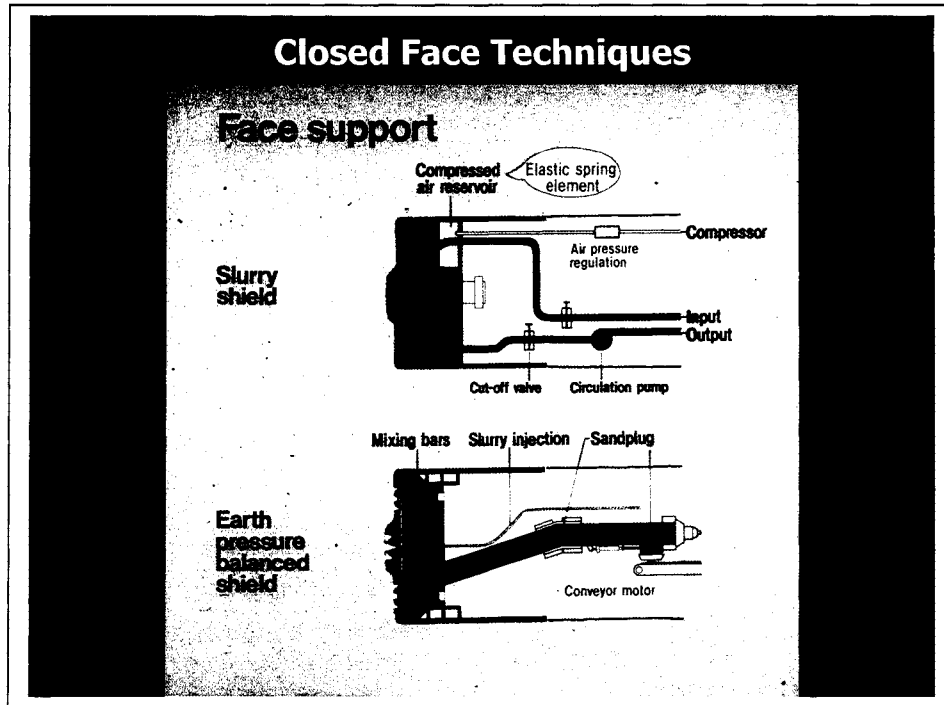
Figure C-1 Slurry and EPB TBM
