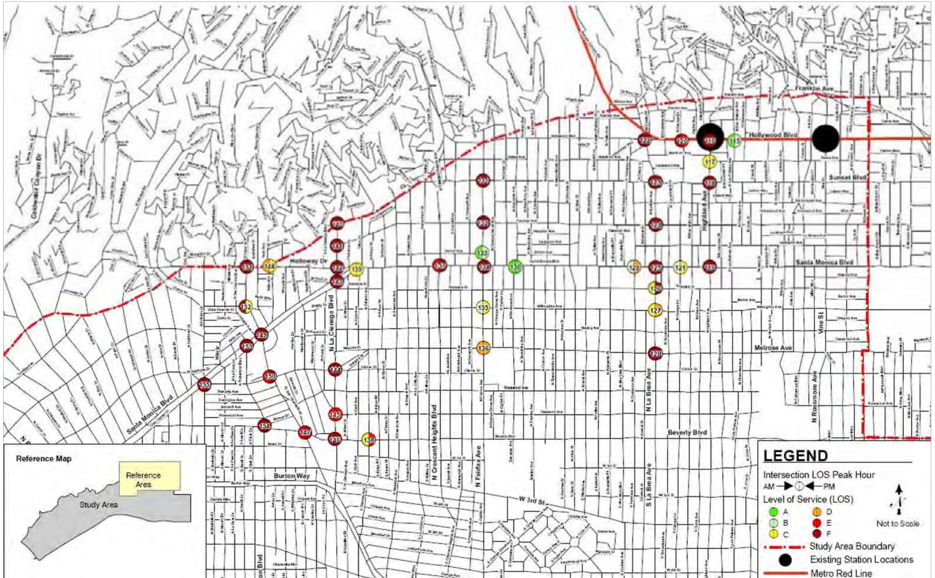
Figure 5-37. Year 2035 Alternative 1 Intersection Levels of Service (continued)
