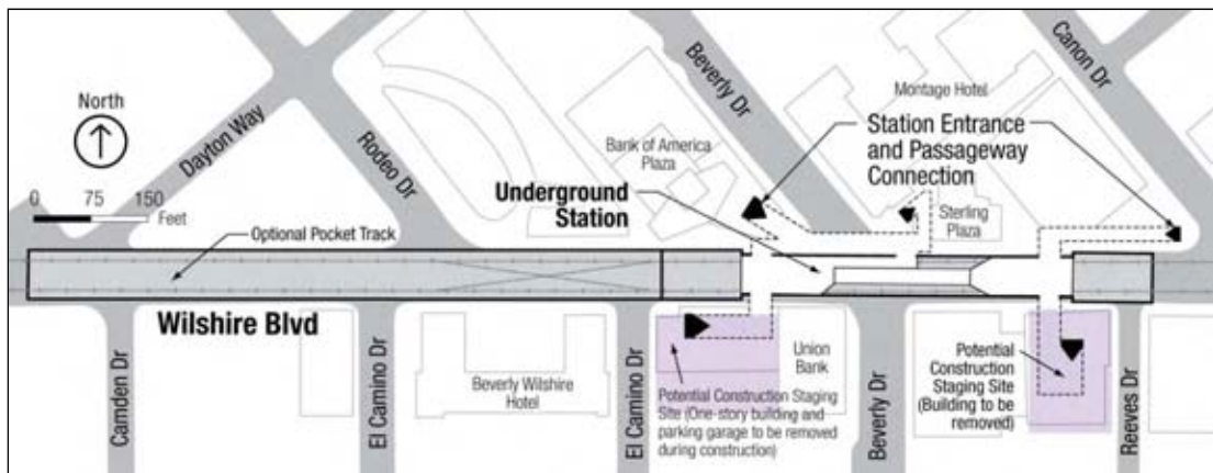
Figure 5-10. Wilshire/Rodeo Station Site Plan
