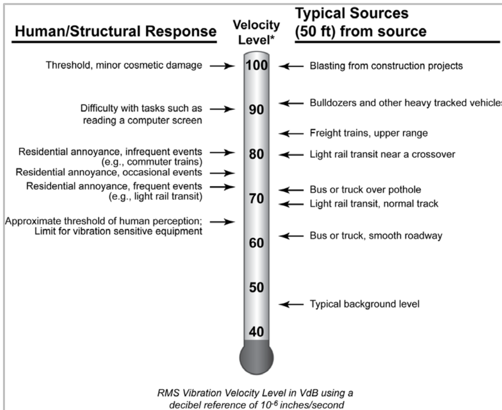
Figure 3.11-2. Typical Groundborne Vibration Levels and Criteria
