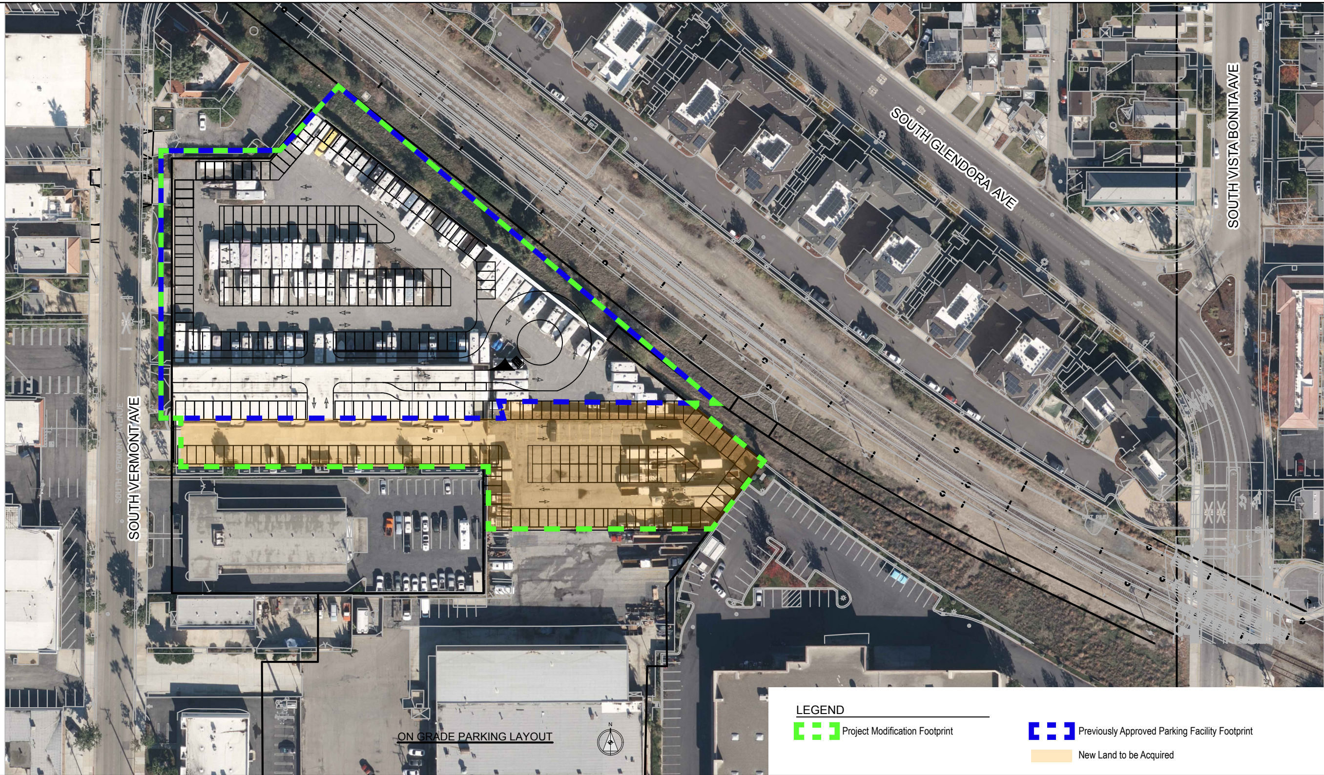
Figure NOP-2 Glendora Station Parking Facility Reconfiguration
