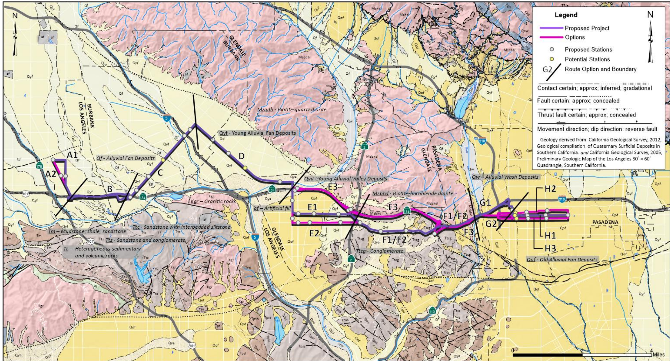
Figure 3 – Regional and Site Geology Map
