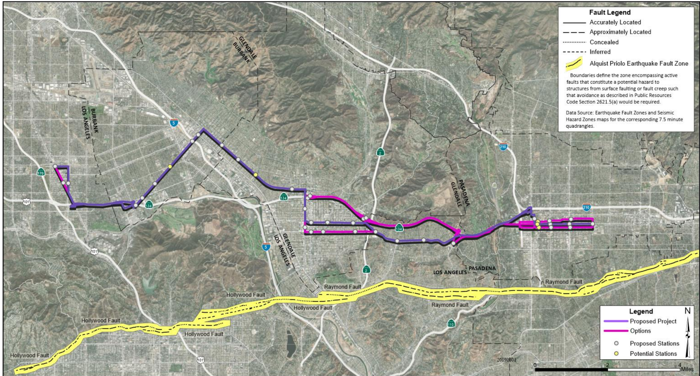
Figure 6 – Alquist-Priolo Earthquake Fault Map
