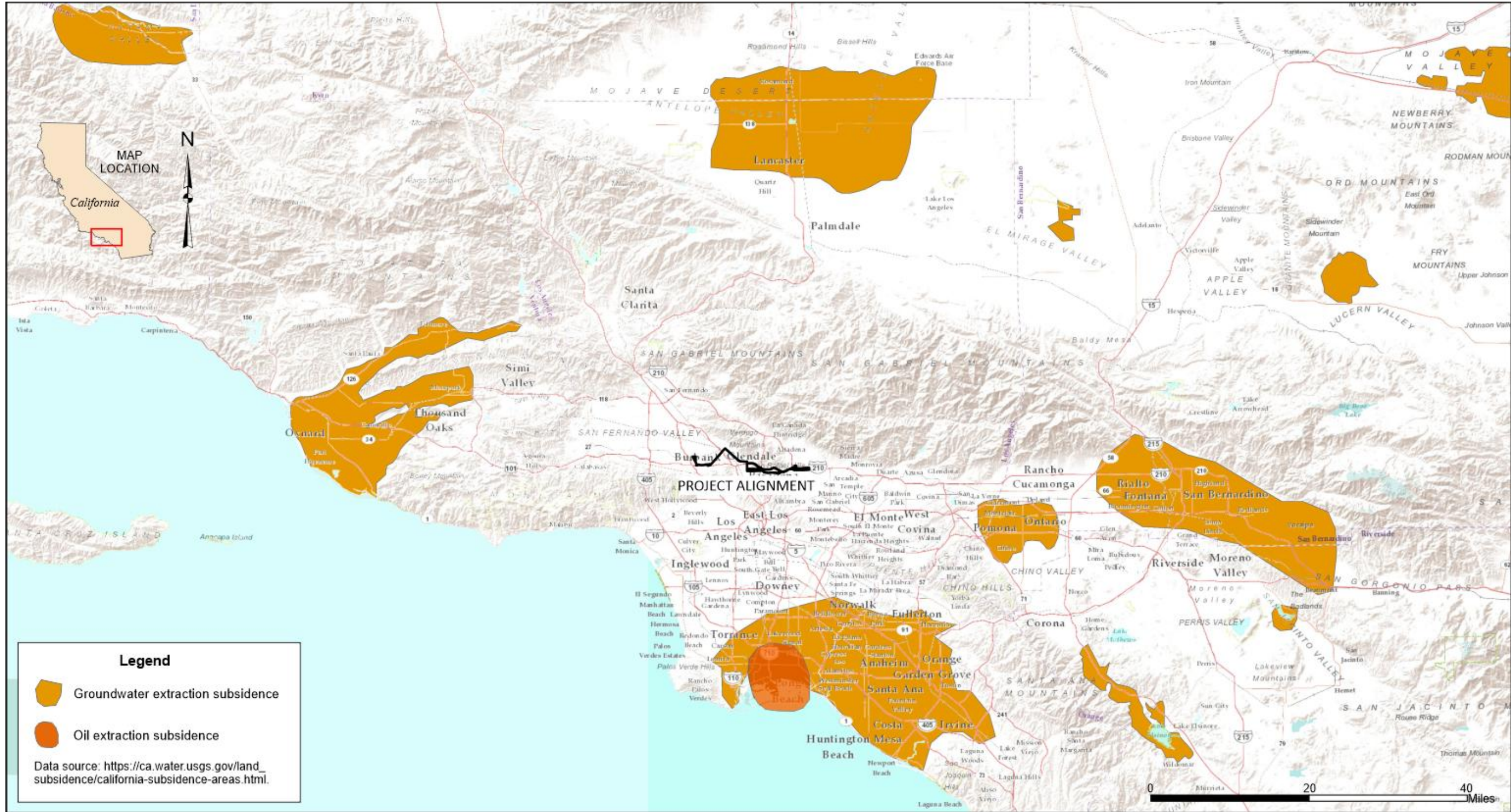
Figure 12 – Land Subsidence Map
