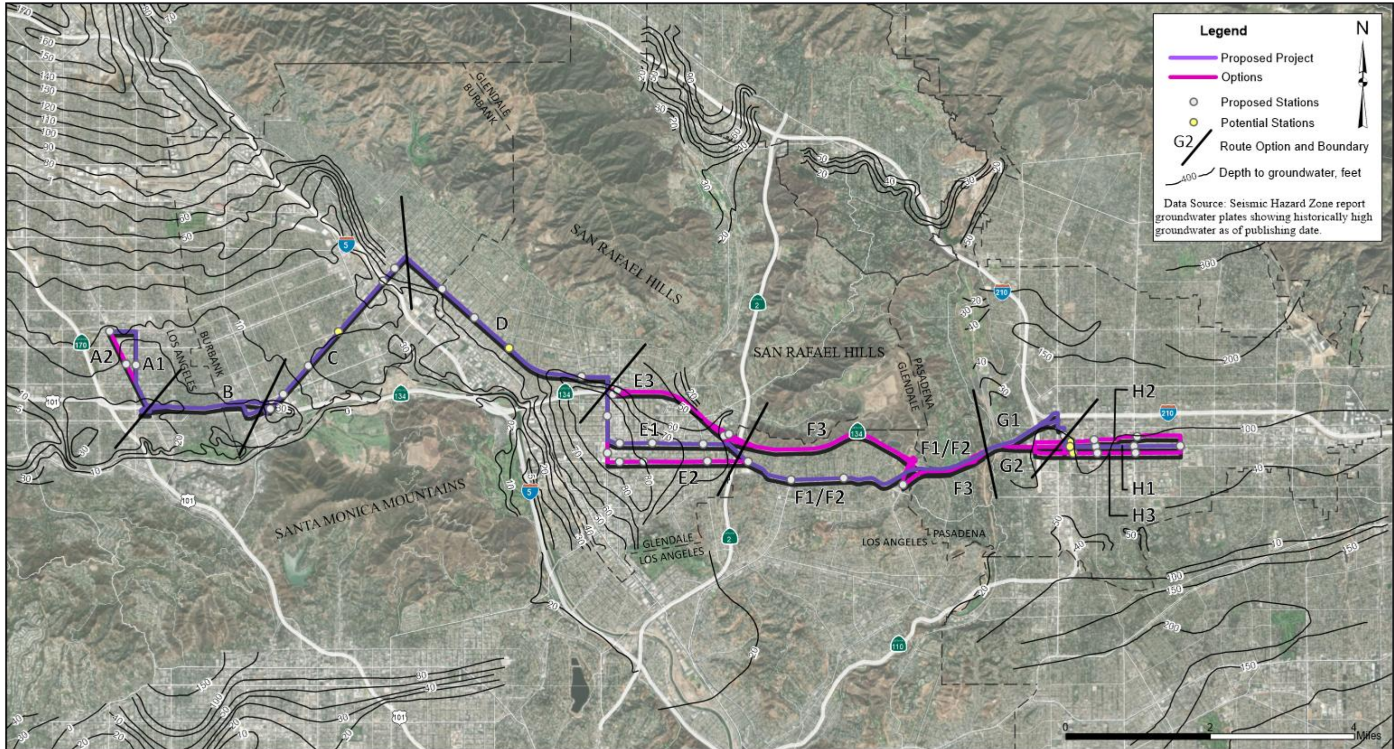
Figure 9 – Historical Groundwater Contours Map
