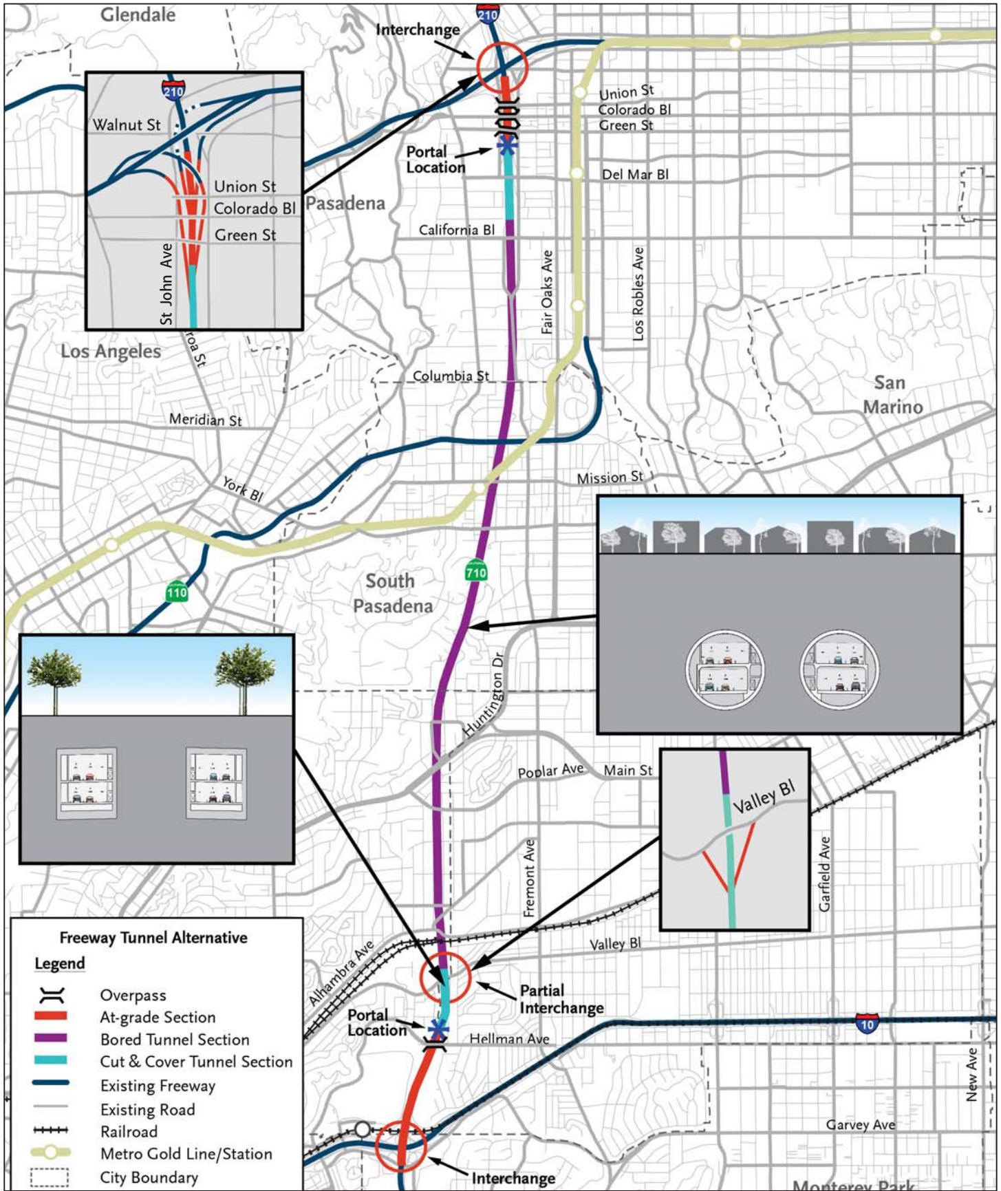
FIGURE 1-6 Freeway Tunnel Alternative Single and Dual Bore Health Risk Assessment SR 710 North Study
