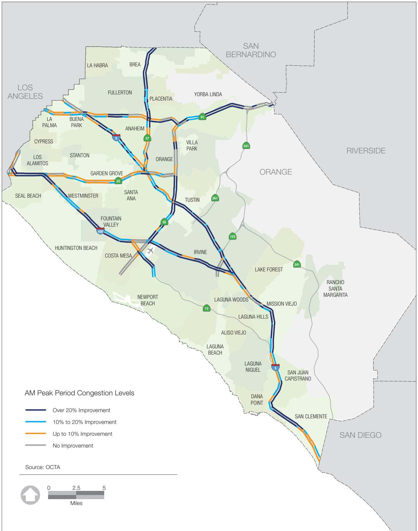
Figure 5-8: Improvement in Level of Service for Year 2035 Preferred Plan
