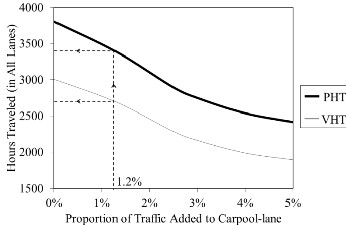
Fig. 7 Predicted total PHT and VHT as functions of the added traffic proportions that are given access to the carpool-lane
