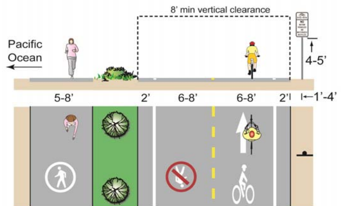
Preferred design, with separation.
