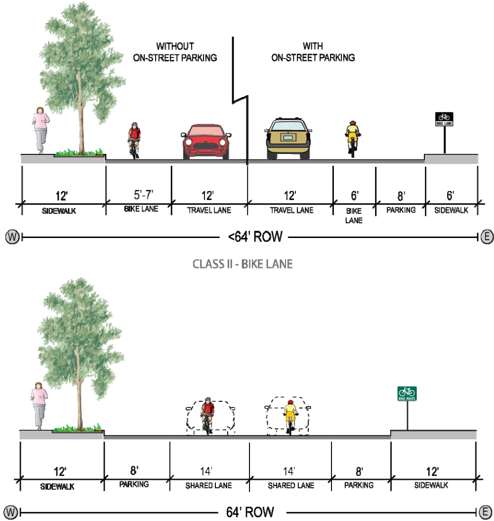
Figure F-8: Local street ROW <math><64'</math>
