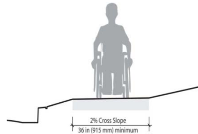
ADA clearance requirement.
