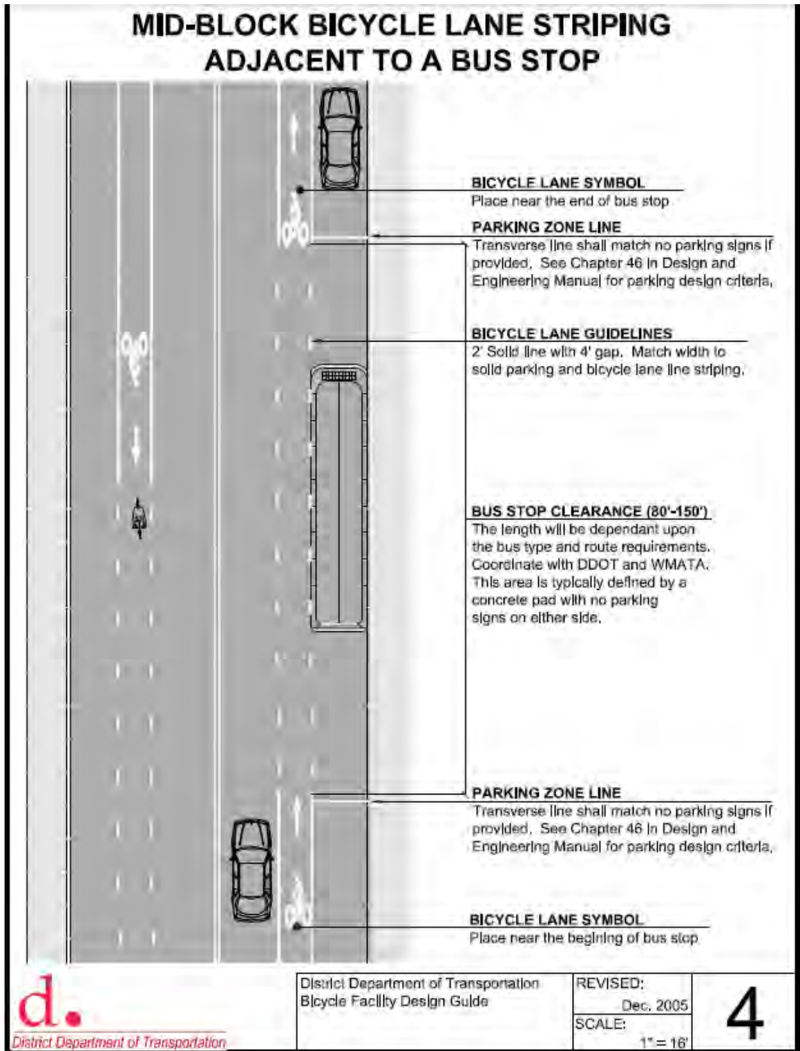
Figure 2.3 - Mid-block bicycle lane striping adjacent to a bus stop
