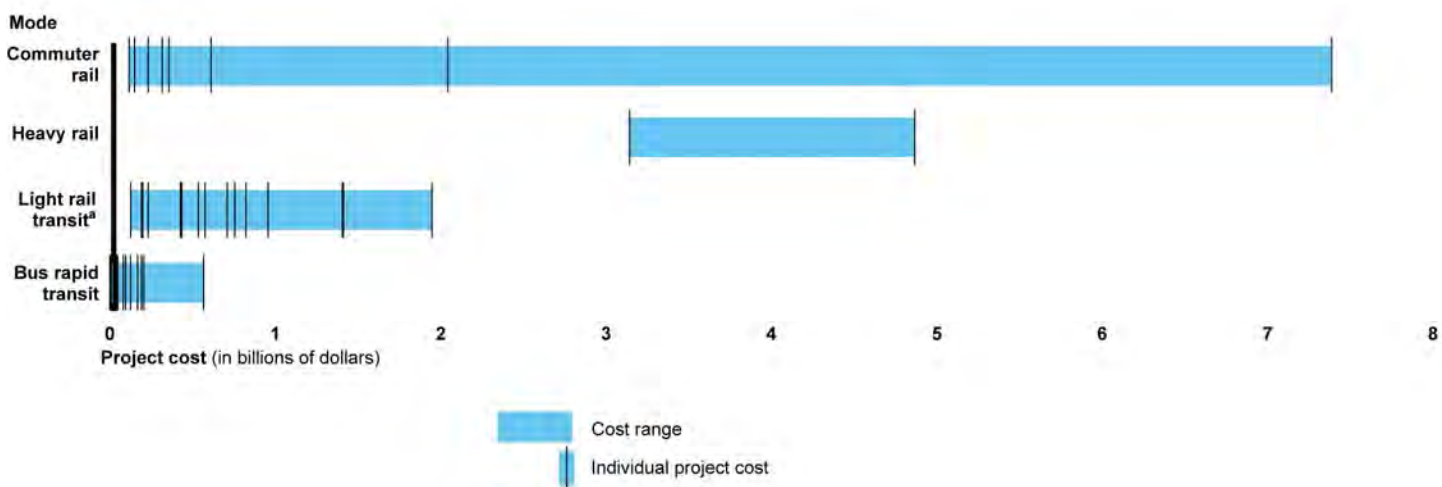
Figure 9: Range and Individual Capital Costs for BRT and Rail Transit Projects Receiving a Grant Agreement from Fiscal Year 2005 through February 2012
