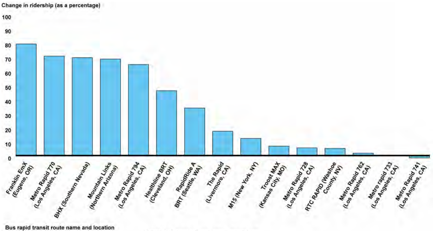
Figure 6: Percentage Change in Ridership for BRT Projects after 1 Year of Operation Compared to Previous Transit Service
