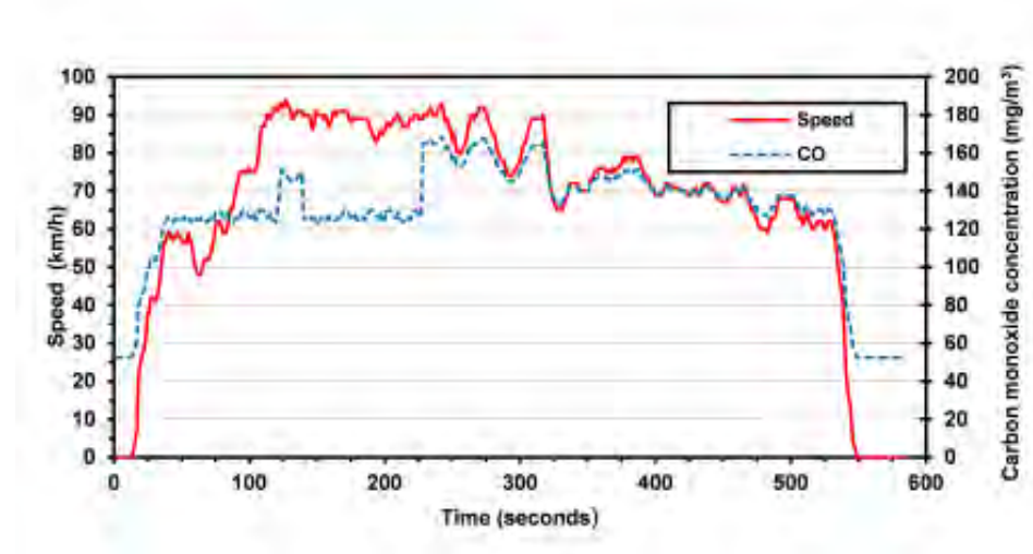
Figure 6.1 Measured variation in CO emissions with vehicle speed
