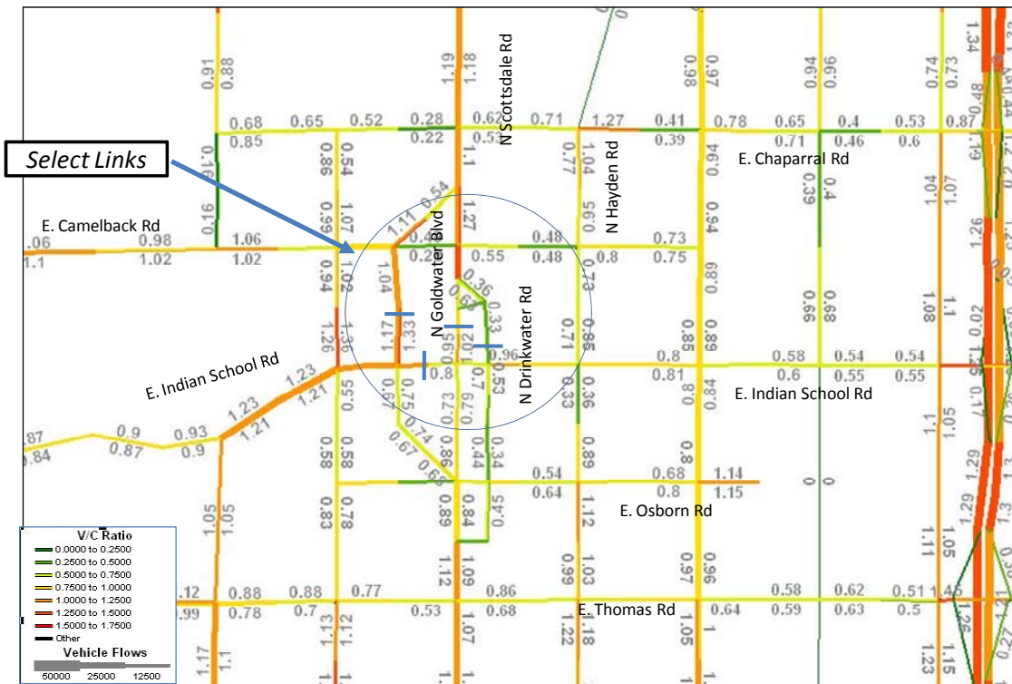
Figure 46A. 2008 Midday V/C Ratios on Scottsdale Road.
