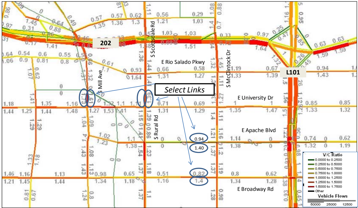
Figure 53A. 2008 PM Peak Period V/C Ratios in Tempe.
