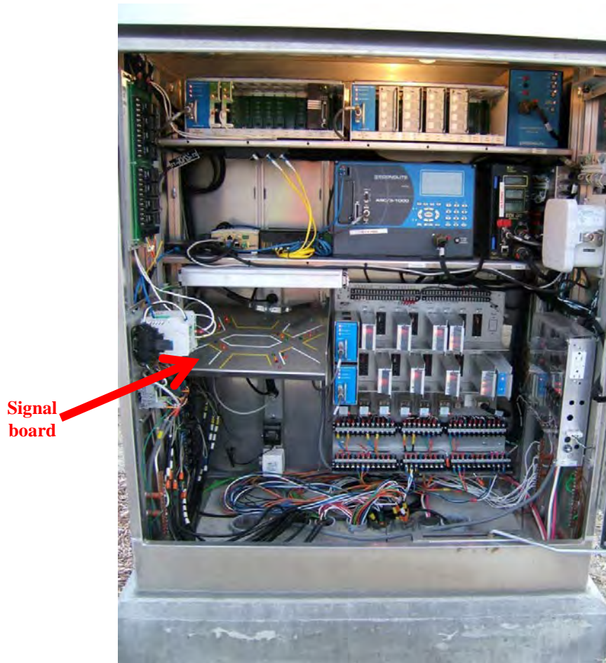
Figure 3-1. Signal Cabinet Pioneer Crossing DDI.
