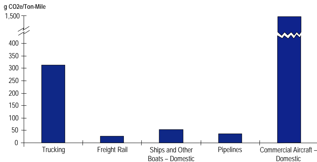
Figure 2.12 GHG Emissions per Freight Ton-Mile by Freight Transportation Mode 2006
