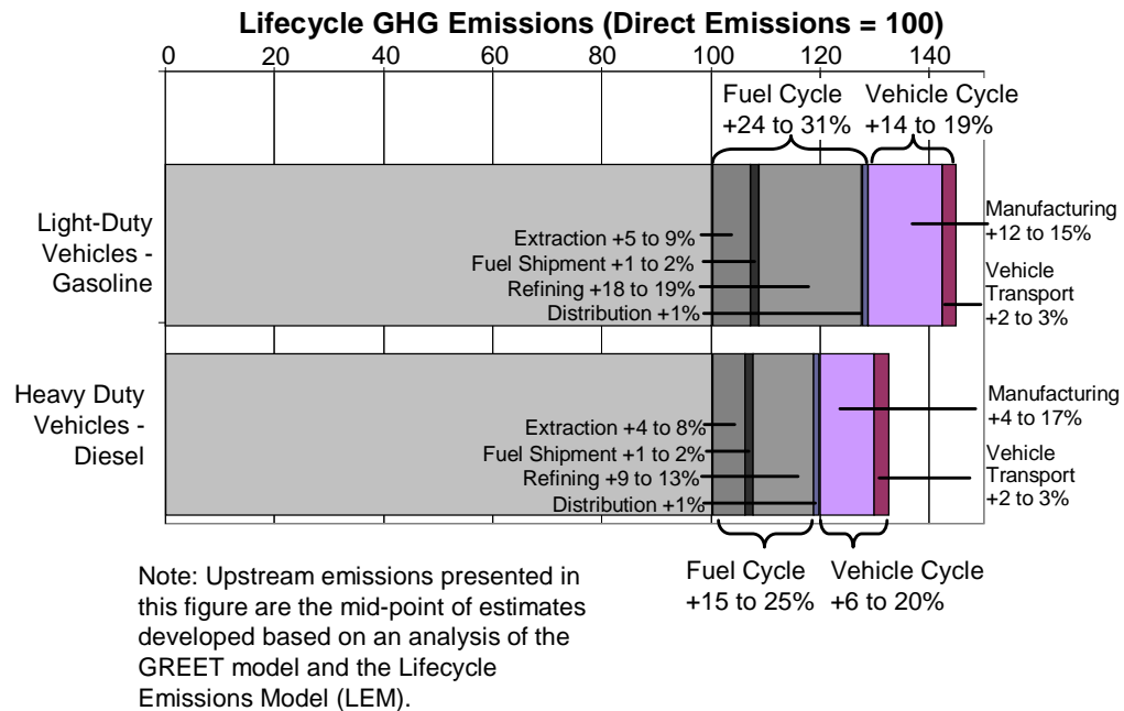
Figure 2.14 Direct GHG Emissions Plus Fuel and Vehicle Cycle GHG Emissions
