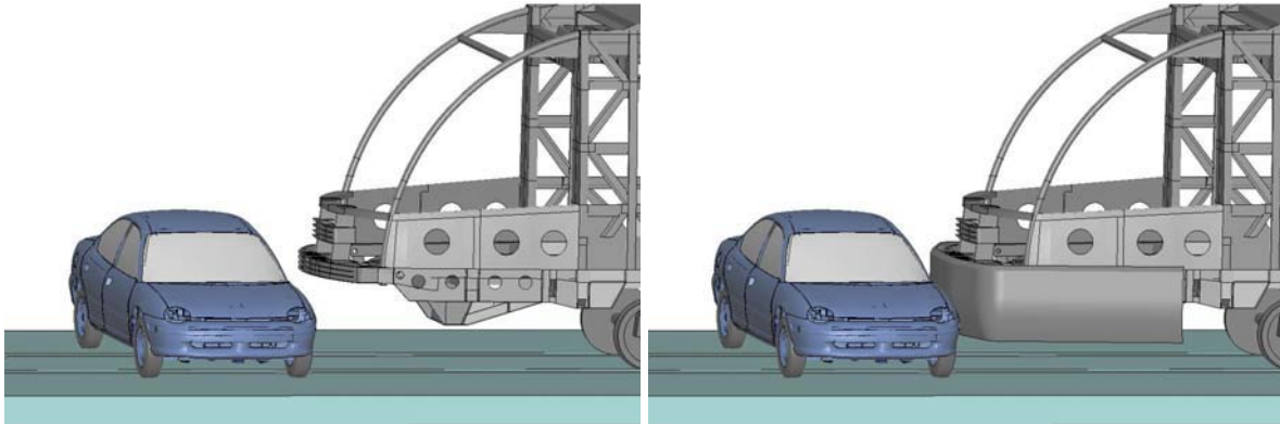
FIGURE 5 Geometric compatibility with and without bumper.
