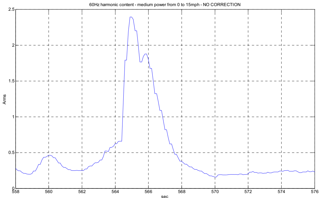
FIGURE 13 60-Hz emission level versus time for base propulsion system configuration.
