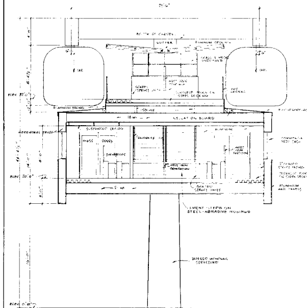
SECTION THRU STATION TYPE 'A' SCALE 1/8" = 1'-0"
