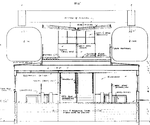
SECTION THRU STATION TYPE 'B' SCALE 1/8" = 1'-0"
