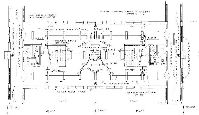
STATION LAYOUT - ZONE C REVERSE LAYOUT FOR ZONE A SCALE: 1/4" = 1'-0"
