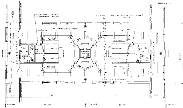
STATION LAYOUT - ZONE B SCALE: 1/4" = 1'-0"
