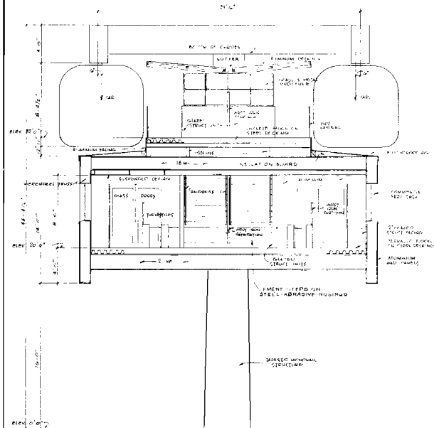
SECTION THROUGH STATION TYPE 'A'
