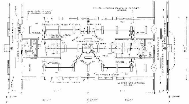
STATION LAYOUT - ZONE C REVERSE LAYOUT FOR ZONE A SCALE 1/4" = 1'-0"
