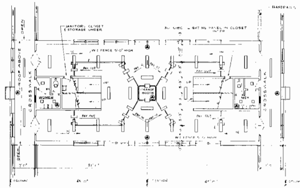
STATION LAYOUT - ZONE B SCALE 1/4" = 1'-0"
