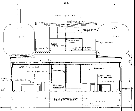
SECTION THROUGH STATION TYPE 'B'
