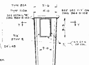
SECTION E-E
