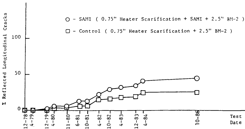
FIGURE K-8 Percent longitudinal cracks vs. time. (K13)
