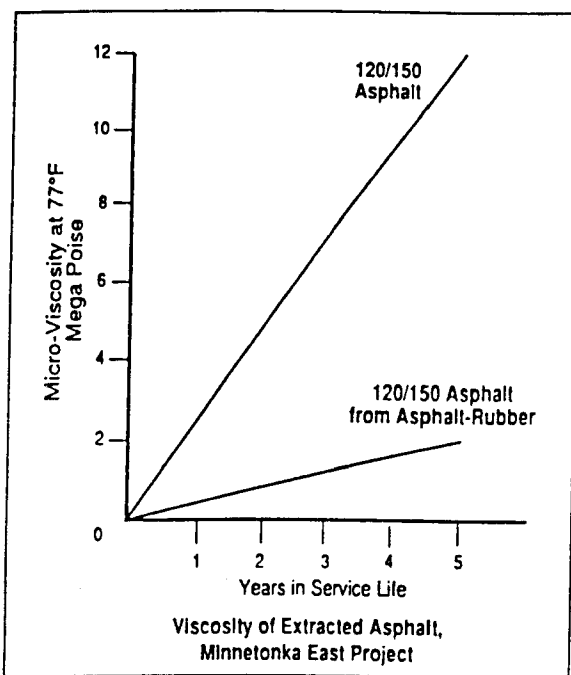
FIGURE 4 Aging resistance (22).
