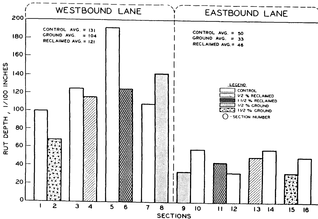
FIGURE O-3 Final rut-depth measurements for test sections and comparable control sections. (O11)
