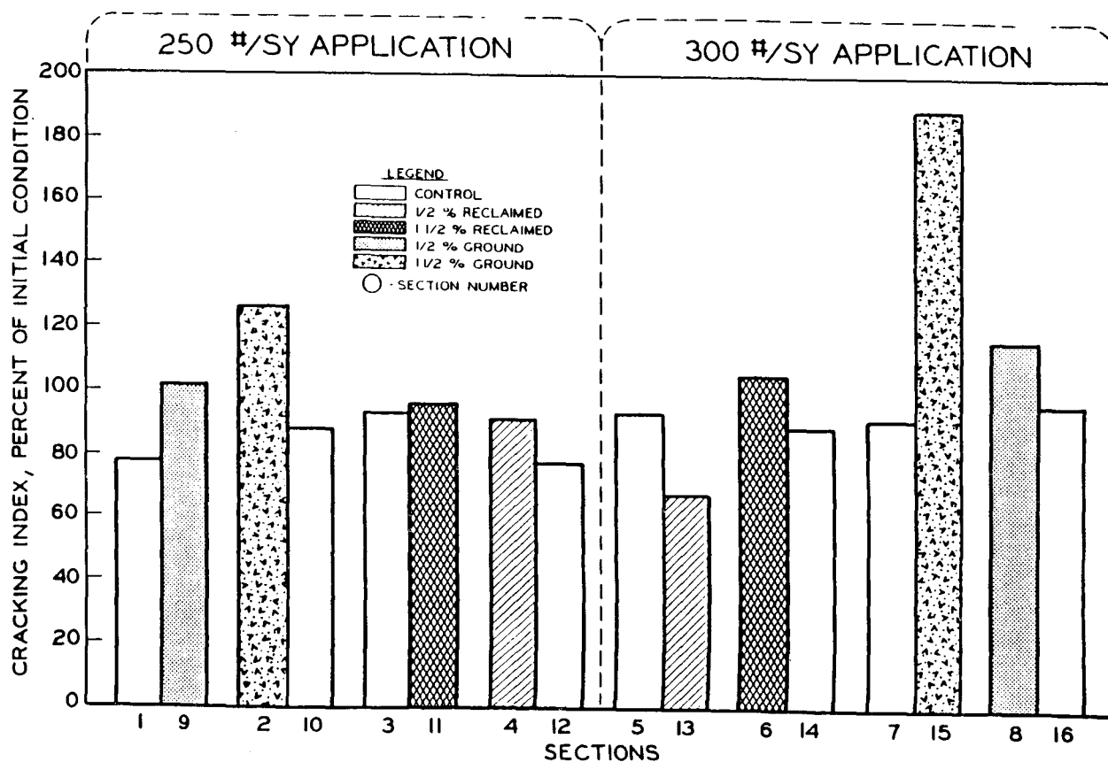
FIGURE O-2 Cracking index ratios for test sections and comparable control sections of conventional mixture. (O11)
