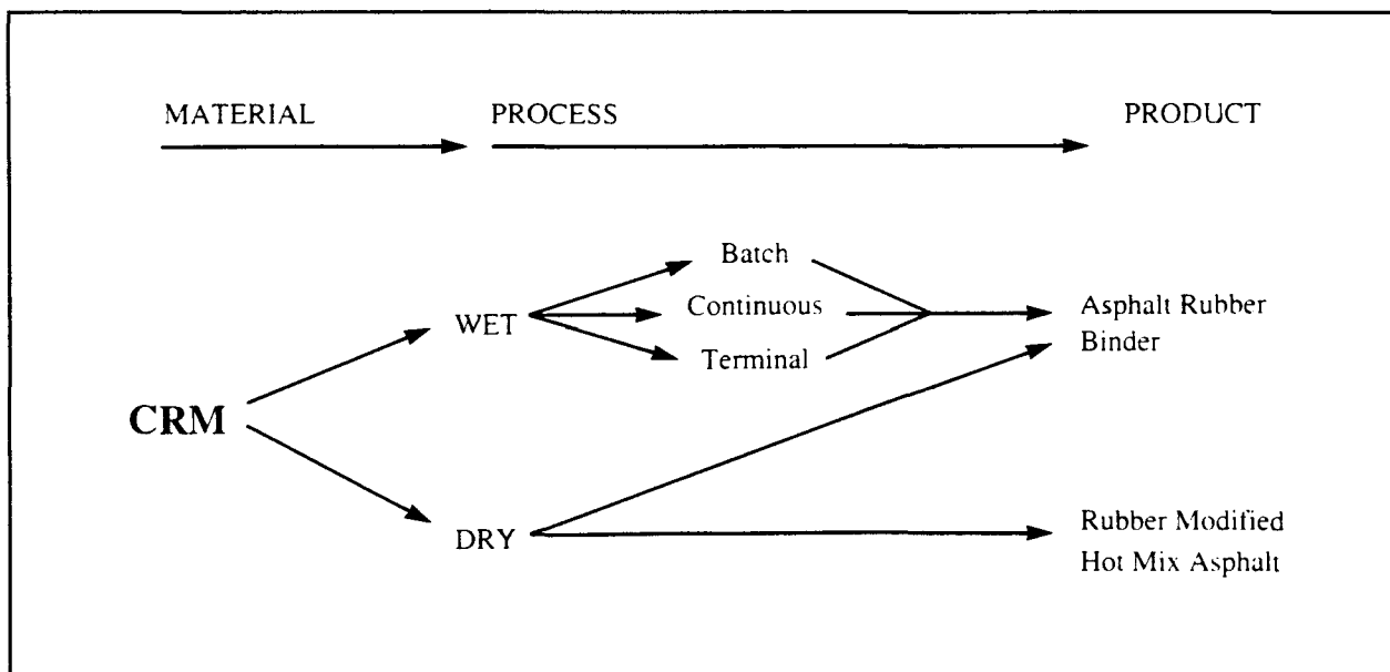
FIGURE 1 The relationship of crumb rubber modified (CRM) terminology and technology (12).
