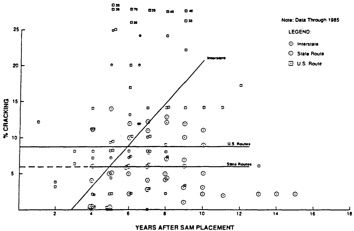
FIGURE H-2 Pavement crack development in SAMs. (H2)
