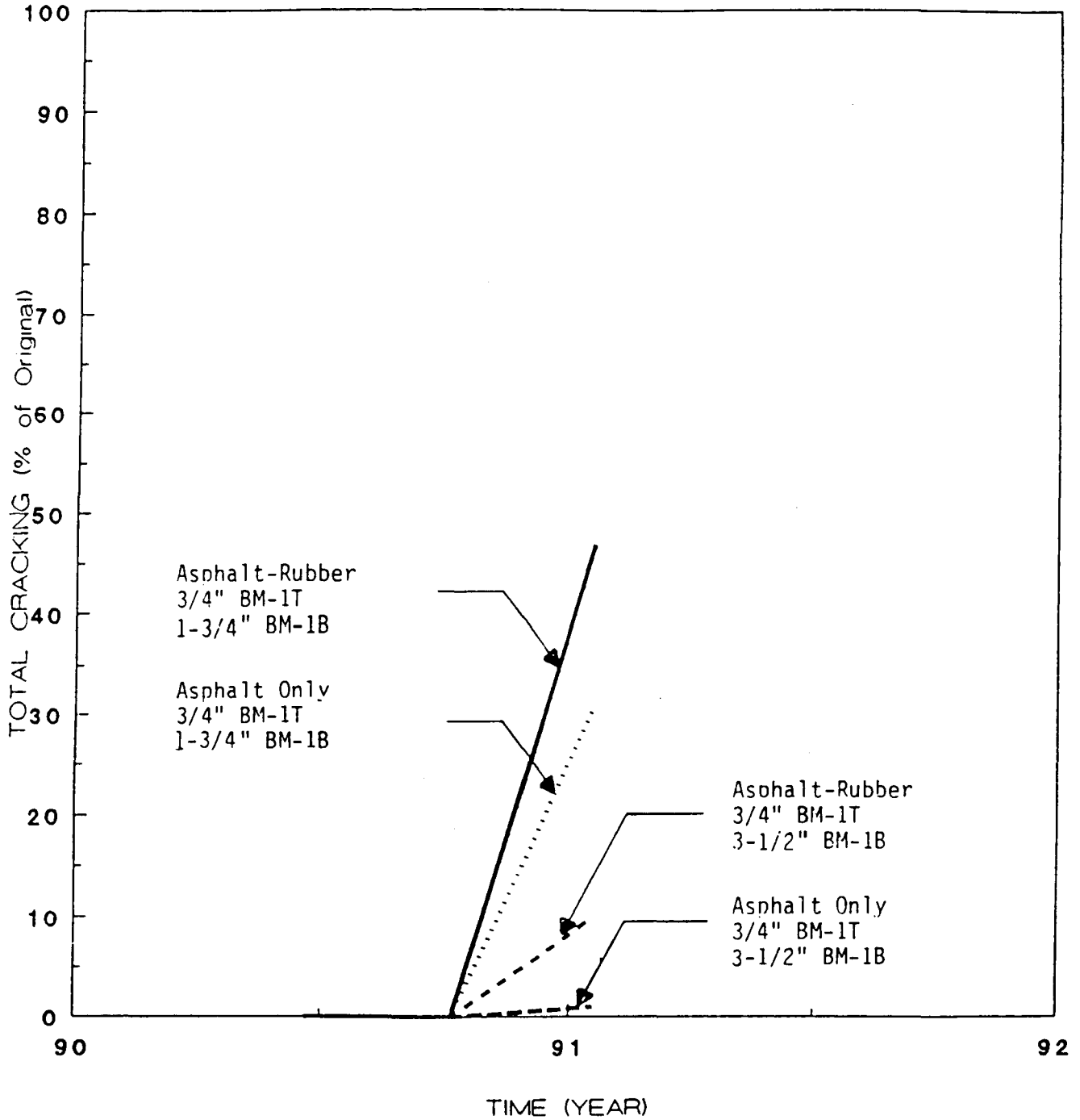
FIGURE O-1 Test and control sections/total cracking, US 75. (O15)
