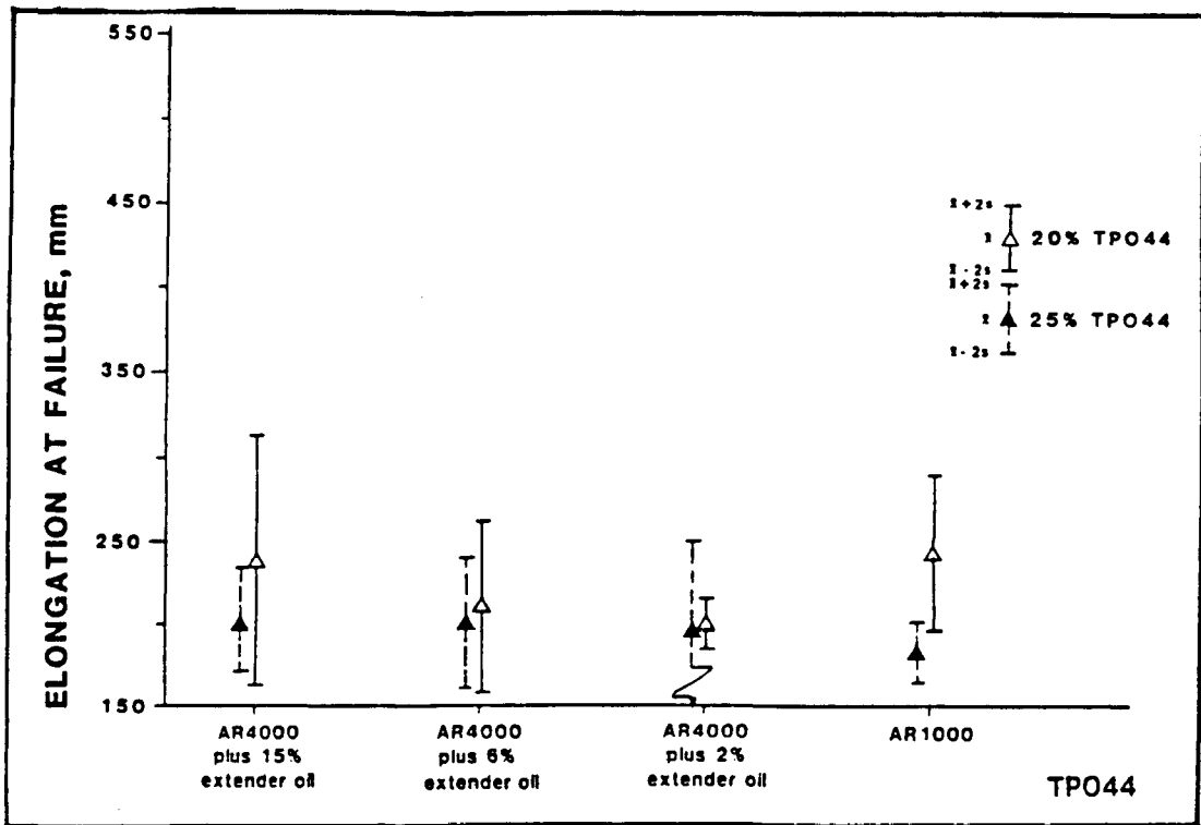
FIGURE D-10 Influence of asphalt cement and oil extender on force ductility elongation at failure at 39.2°F. (D2)
