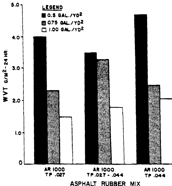
FIGURE F-2 Water vapor transmission rate for various A-R combinations. (F2)
