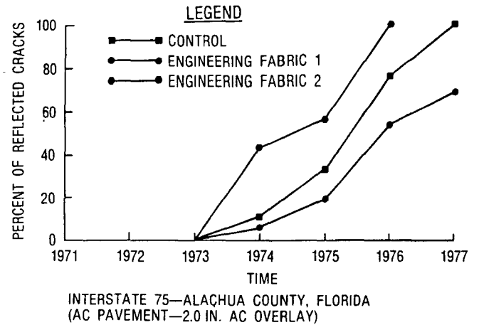
FIGURE K-18 Percent of reflected cracks vs. time, Interstate 75. (K38)
