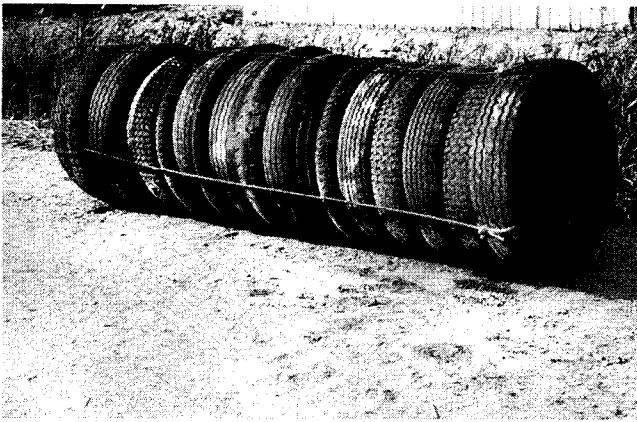
FIGURE 23 Truck-tire culvert from Vermont (113).
