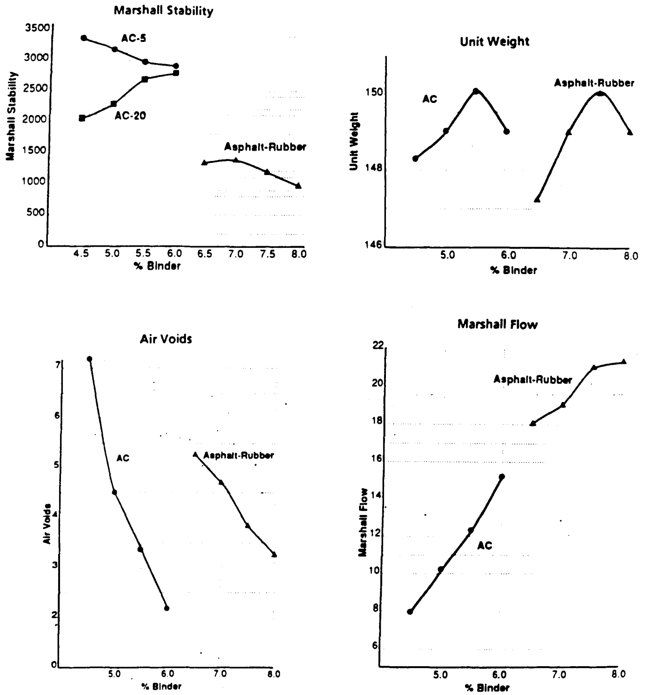
FIGURE N-1 Typical Marshall stability data. (NI)
