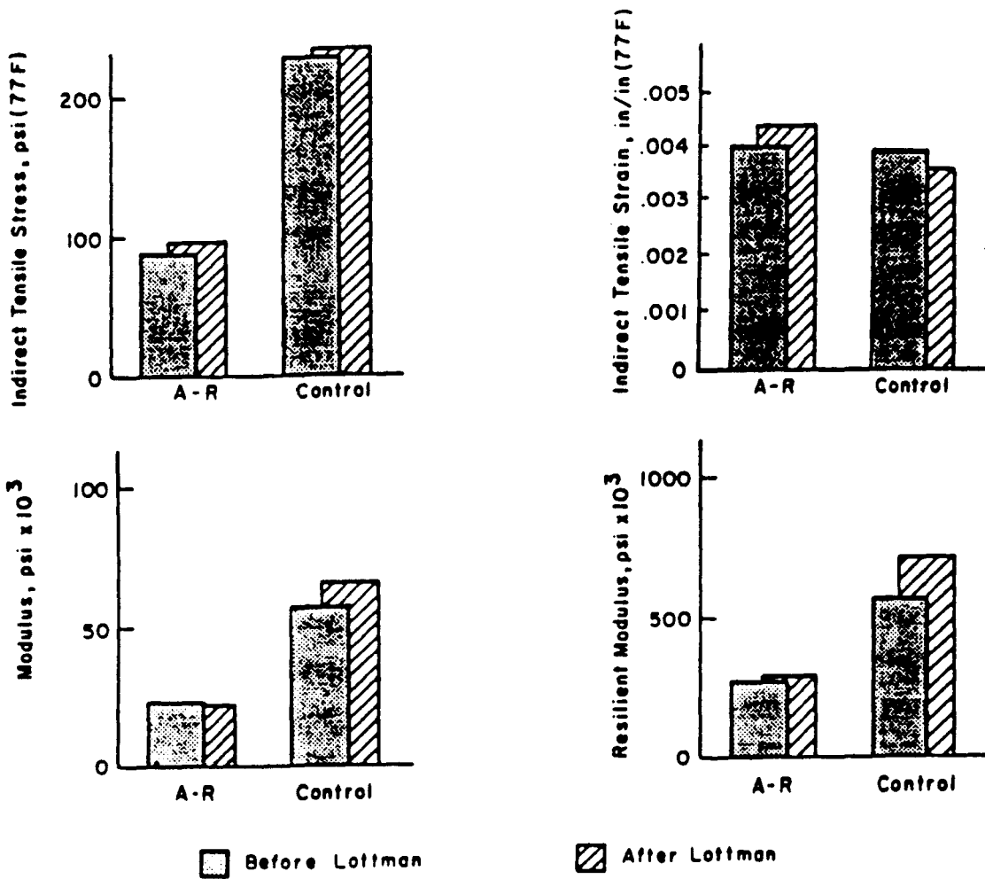
FIGURE N-29 Asphalt-rubber concrete vs. control "adequate" limestone mixes. (N5)
