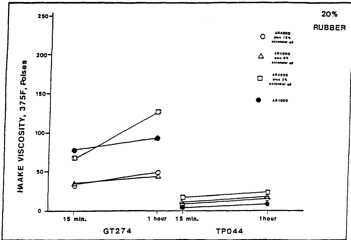
FIGURE D-11 Influence of asphalt cement and oil extender on viscosity at 375°F. (D2)
