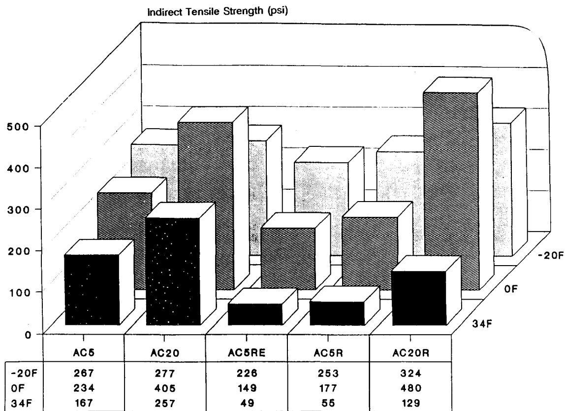
FIGURE N-32 Comparison of average indirect tensile strengths at all temperatures for all mixtures. (NII)
