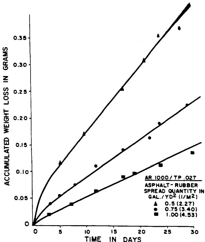
FIGURE F-1 Water vapor transmission accumulated weight loss vs. time for AR 1000/TP.027. (F2)
