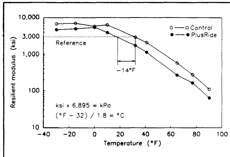
FIGURE N-16 PlusRide: Resilient modulus vs. temperature for evaluating low temperature cracking. (N9)
