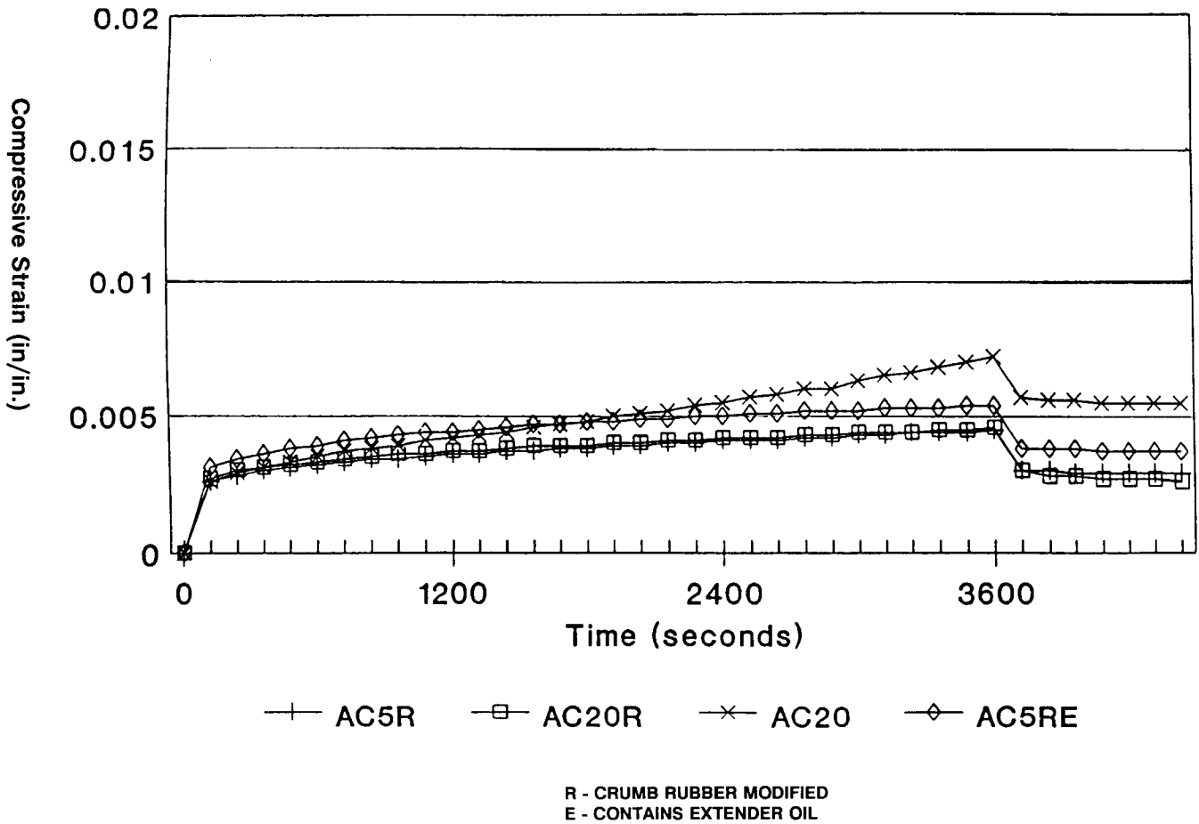
FIGURE N-18 Compressive strain vs. time for static loading conducted at 104°F. (N11)
