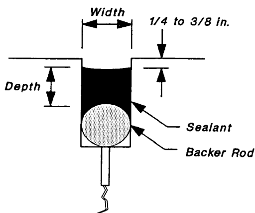
FIGURE 15 Typical poured joint sealant installation (9).
