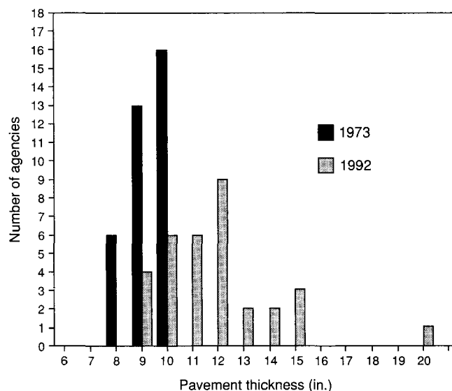
FIGURE 6 Distribution of maximum specified pavement thicknesses.
