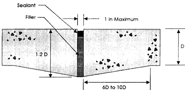
(b) Undoweled - Thickened Edge (Isolation)
