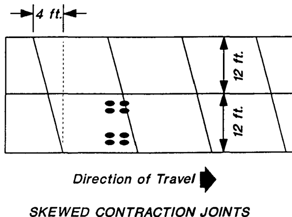
FIGURE 9 Typical skewed transverse joints (9).
