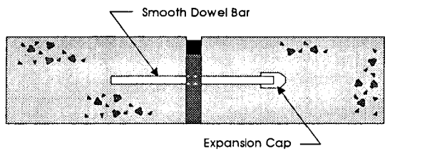
(a) Doweled
