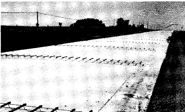
FIGURE 17 Dowel assemblies in place prior to paving (9).
