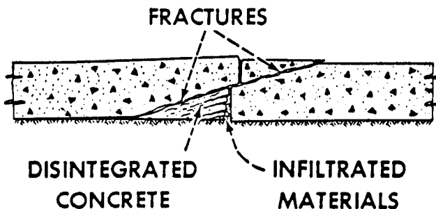
FIGURE 31 Blowup mechanism (after 93).
