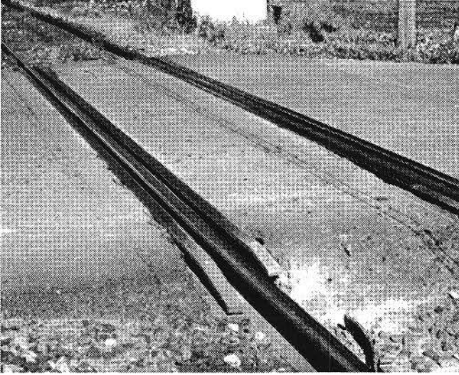
FIGURE 5 Formed-in-place asphalt.
