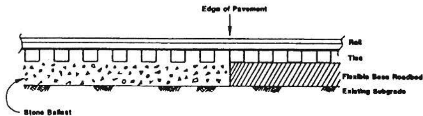
FIGURE 17a Cross section of crossing surface prior to hot-mix asphalt application.
