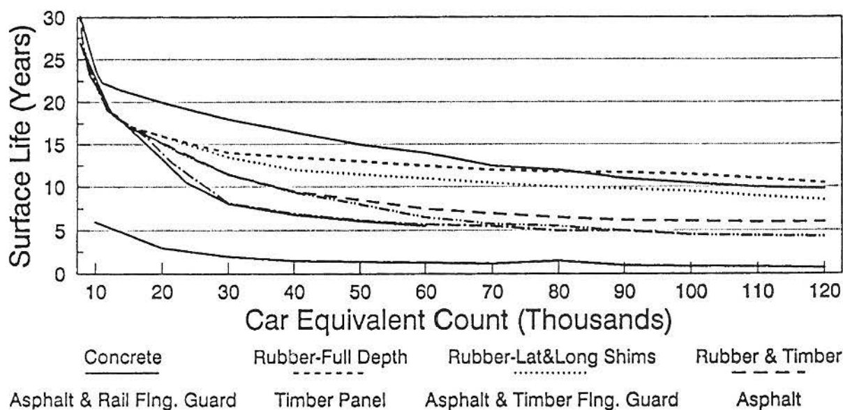
FIGURE 19 Service life of grade crossing surfaces—years versus highway traffic with limited railroad traffic.
