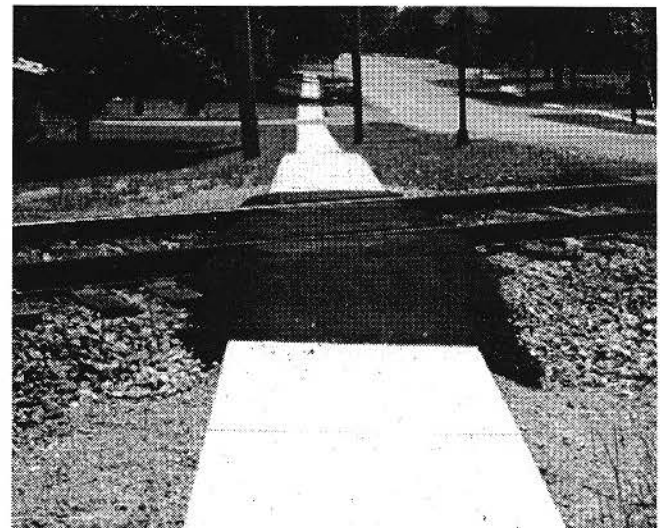
FIGURE 15b Appropriate sidewalk design through track structure.
