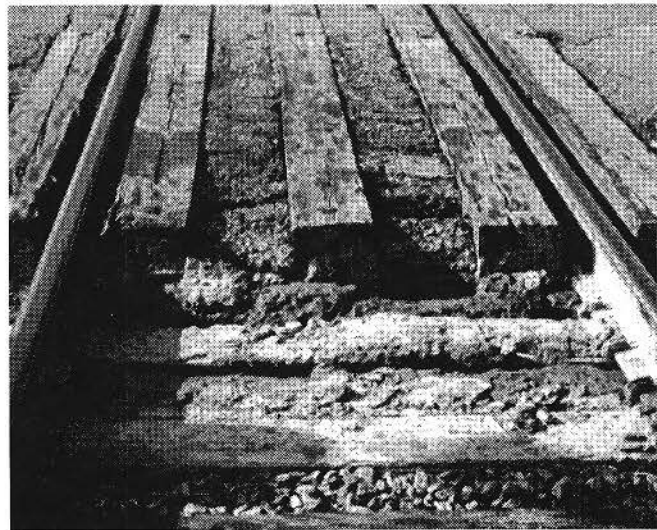
FIGURE 14b A poorly drained crossing surface.
