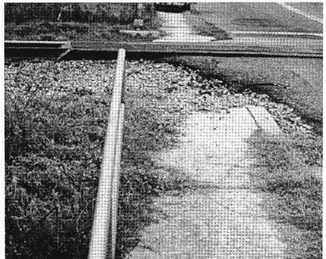
FIGURE 15a Provision not made for sidewalk through track structure.
