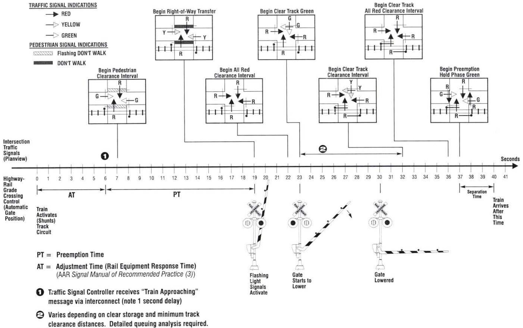
FIGURE 15 Sample advance preemption time line.
