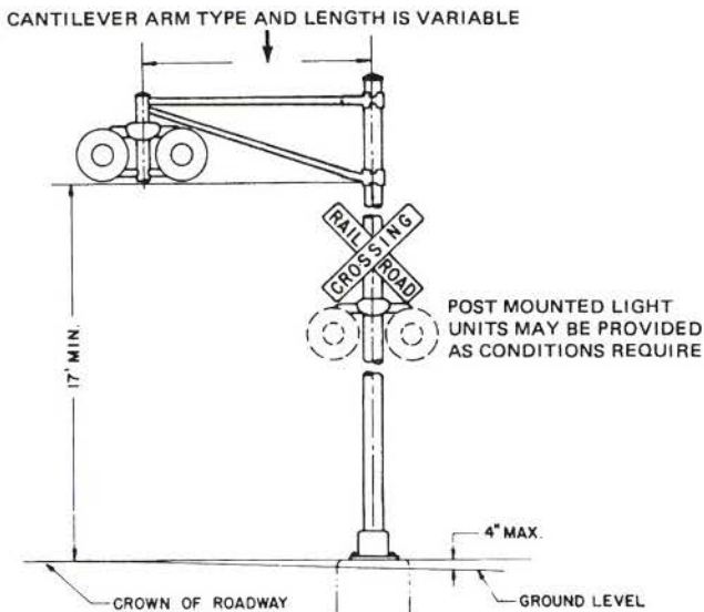
FIGURE 3 Flashing light signals (4).
