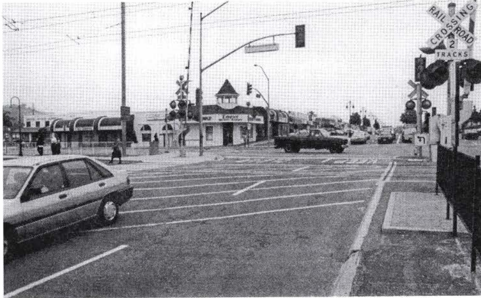
Broadway Highway-Rail Grade Crossing Lemon Gove, California (on the San Diego LRT System)
