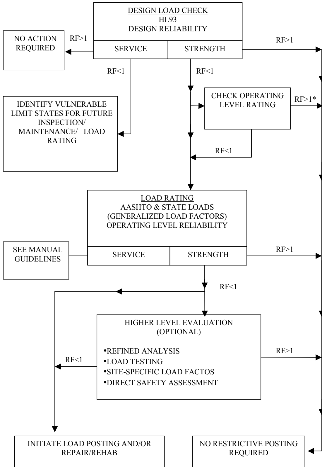
Figure 3-1. LRFR Flow Chart for Non-Permit Loads
