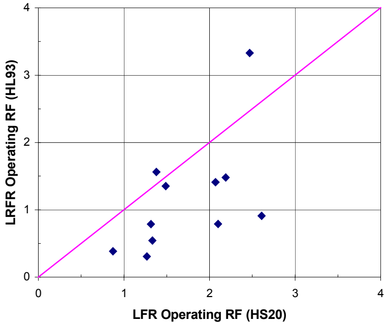
Figure 5-10. Prestressed Concrete I girder Bridges Design Load (Operating)
