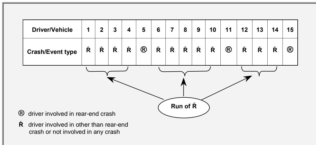
Figure 2. Sequence of crash events required to wait through for the involvement of k = 3 drivers in rear-end crashes.
