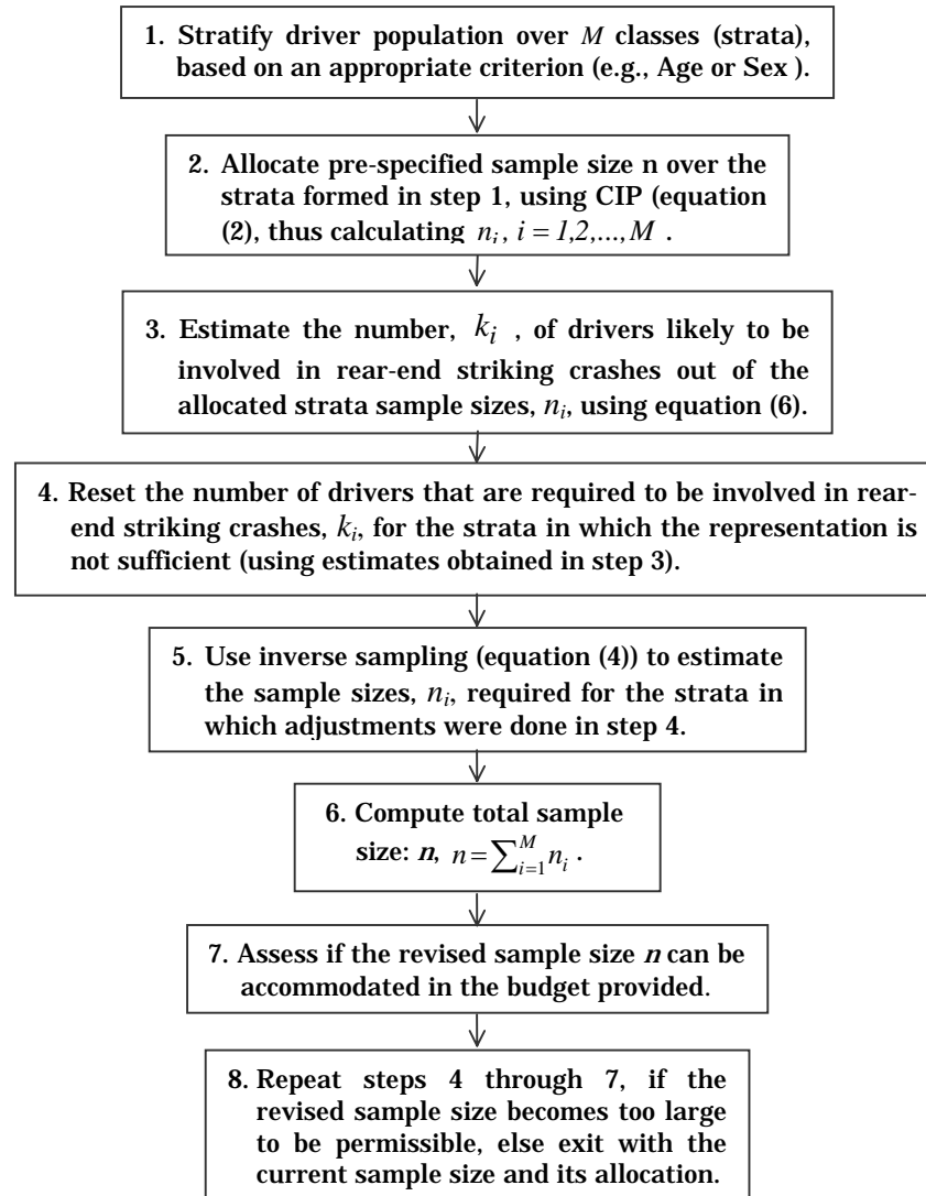
Figure 4. Sampling strategy with restriction on the sample size
