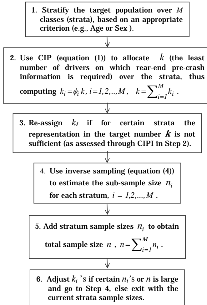
Figure 3. Sampling strategy when the target number, k , of drivers involved in rear-end crashes is to be observed.
