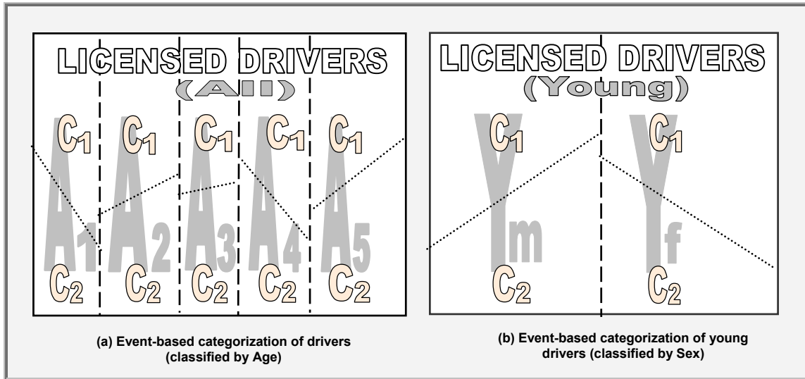
Figure 1. Categorization of drivers (classified by Age and Sex), based on Crash event: Rear end crash involvement or otherwise.
