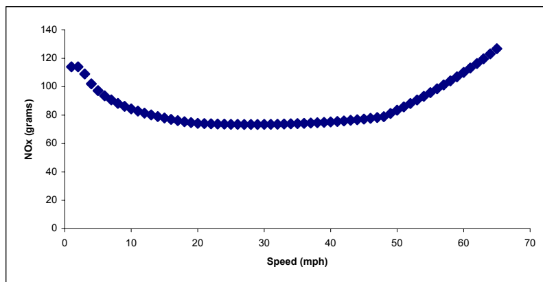
Figure 4.2 Plot of NO x emissions (all vehicle emission factors* vehicle travel activity) against average speed.
