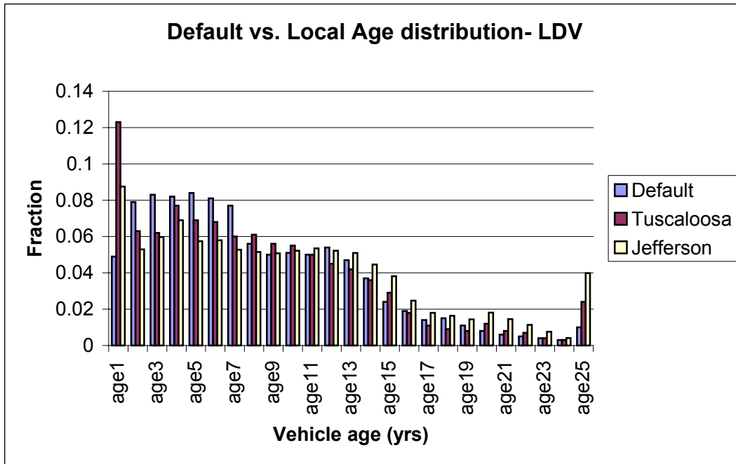
Figure 4.5 Registration distribution data of national default, Tuscaloosa and Jefferson Counties.
