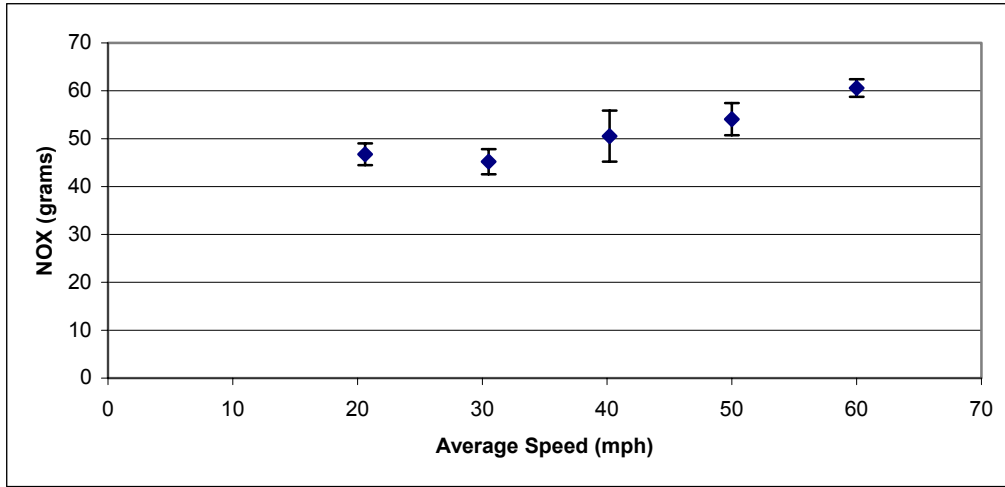
Figure 4.4 Variation in NO x due to trip speed distribution. Error bars are 95% confidence intervals.
