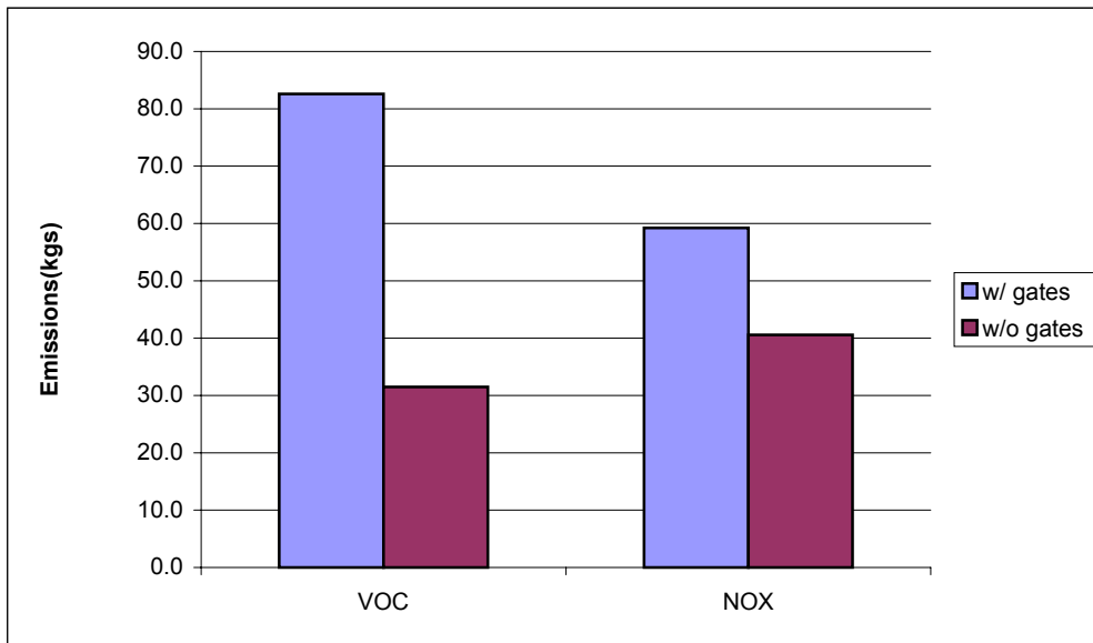
Figure 4.10 Comparison of VOC and NO x emissions between “with gates” and “without gates” scenarios in railroad case study.
