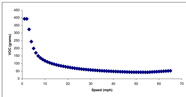
Figure 4.1 Plot of VOC emissions (all vehicle emission factor*vehicle travel activity) against average speed.
