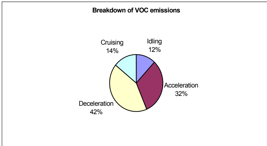
Figure 4.8 Contribution of emissions from different operating phases to the total VOC emissions in the worst-case scenario of single vehicle in signalization case study.
