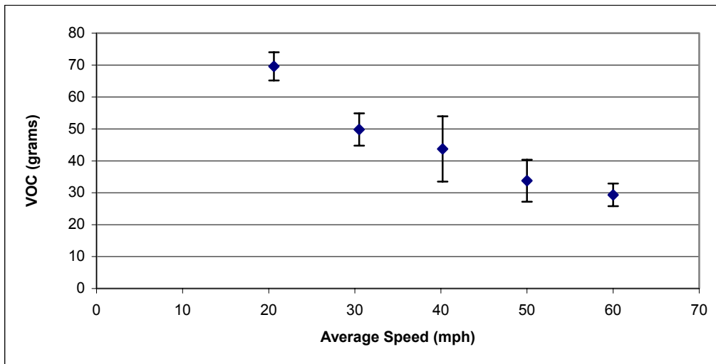
Figure 4.3 Variation in VOCs due to trip speed distribution. Errors bars are 95% confidence intervals.
