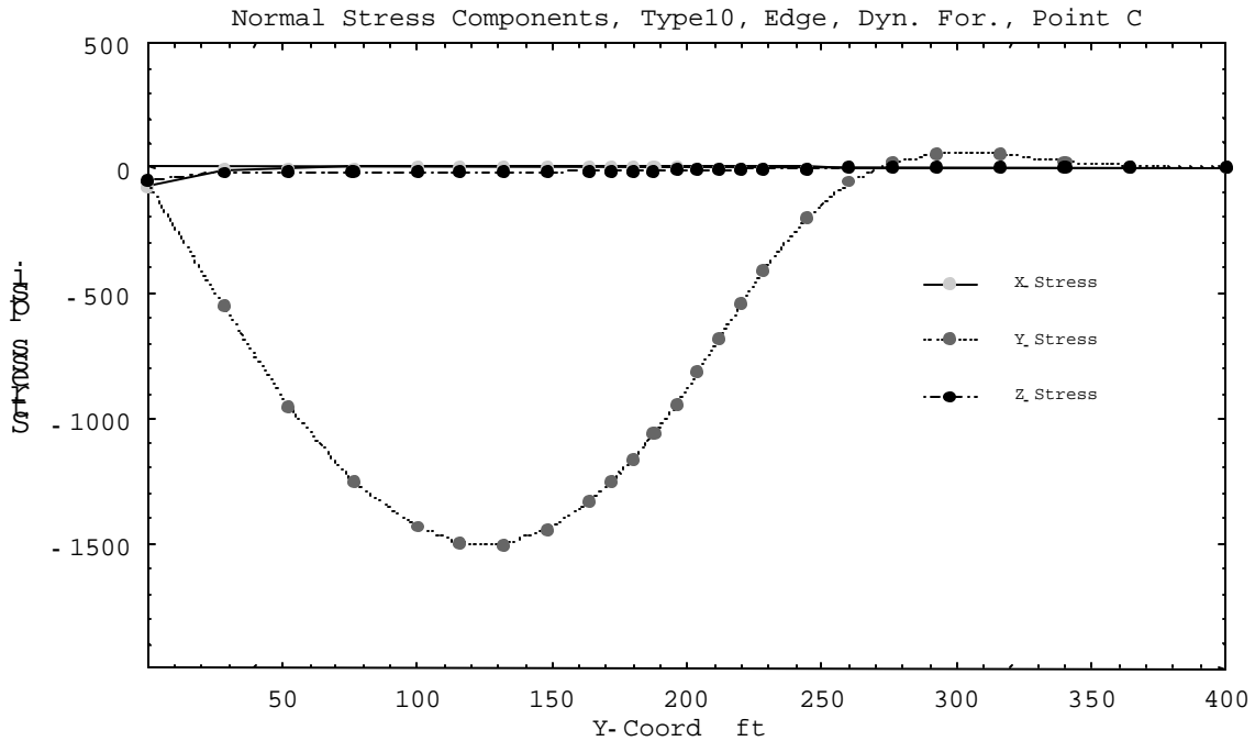
Figure B-11: Normal Stress components along point C of Type 10 Rail (400-ft, Edge Hit, Static, TL5a).
