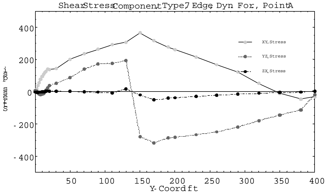
Figure B-4: Shear Stress components along point A of Type 7 Rail (400-ft, Edge Hit, Static, TL5a).
