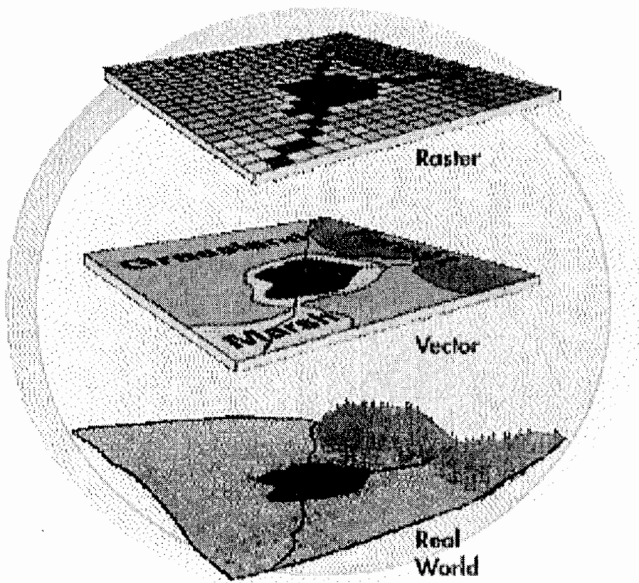
Figure 3. Raster and vector representations of real world data [17].
