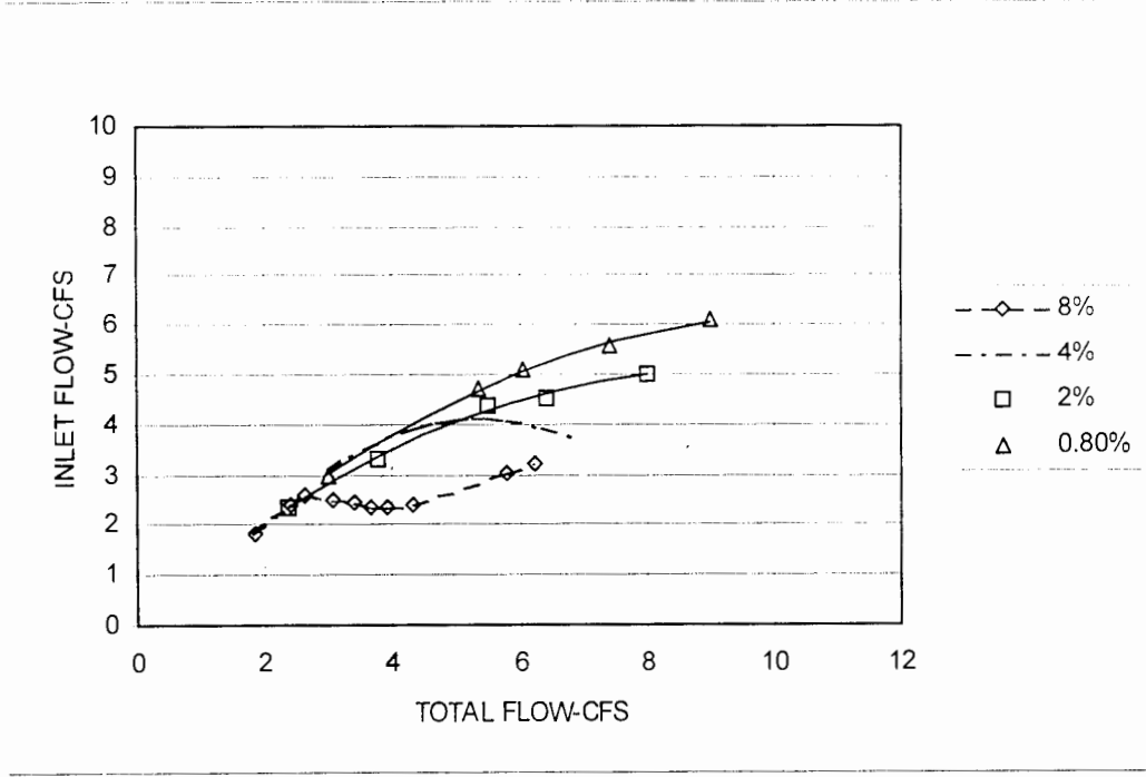
Figure 8: Full size performance curves for inlet Index 213 at 6% cross slope. Parameter is longitudinal slope.
