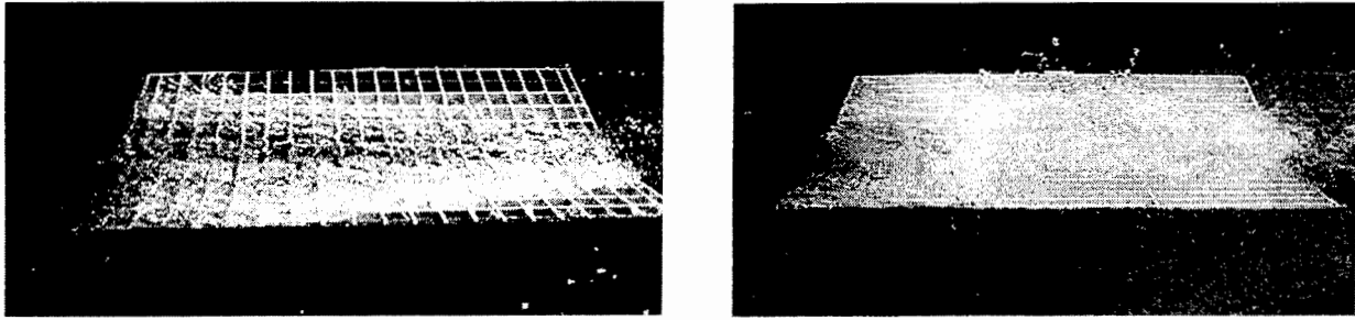
Figure 26: Flow across grating, reticuline grate (left), crossbar grate (right) at longitudinal slope 4% and a total flow of 1 CFS. Note water splash is much higher in the case of the crossbar grate.
