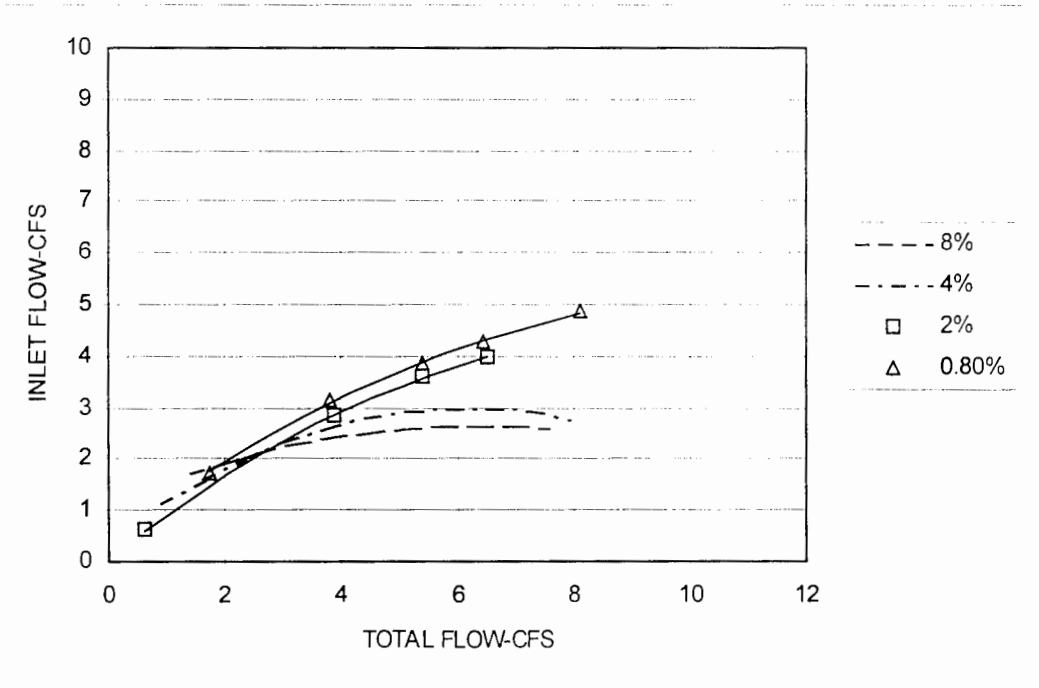
Figure 10: Full size performance curves for inlet Prototype inlet at 4% cross slope. Parameter is longitudinal slope.
