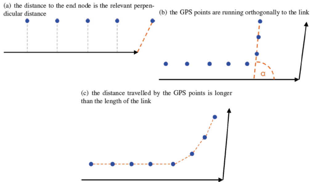
Figure 32. Three Criteria Used to Assess Reaching End of Link (Schuessler and Axhausen, 2009)
