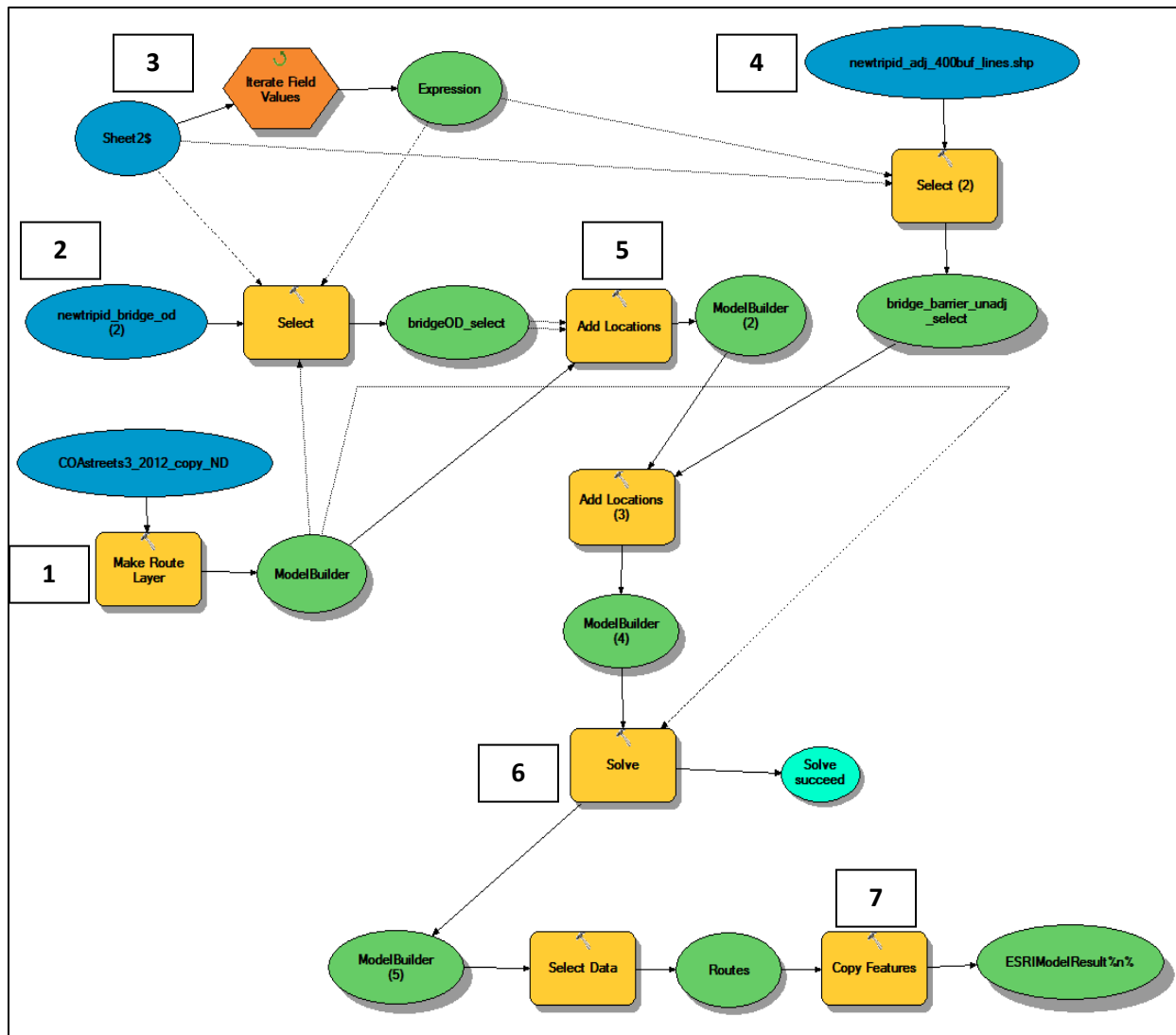
Figure 39. Model for Dalumpines and Scott (2011) Algorithm
