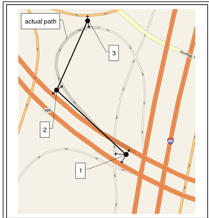
Figure 31. Problems with Matching to the Nearest Road Only (Newsom and Krumm, 2009)
