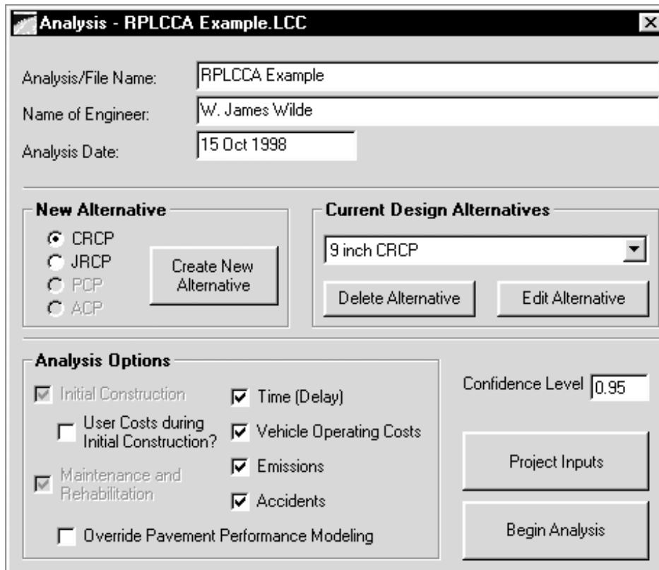
Illustration 9.1. RPLCCA Analysis Window
