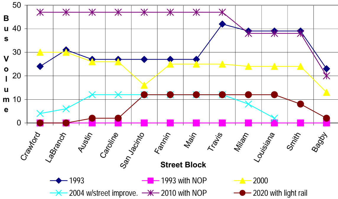
Typical Output for AM Peak Scenarios (Walker Street)
