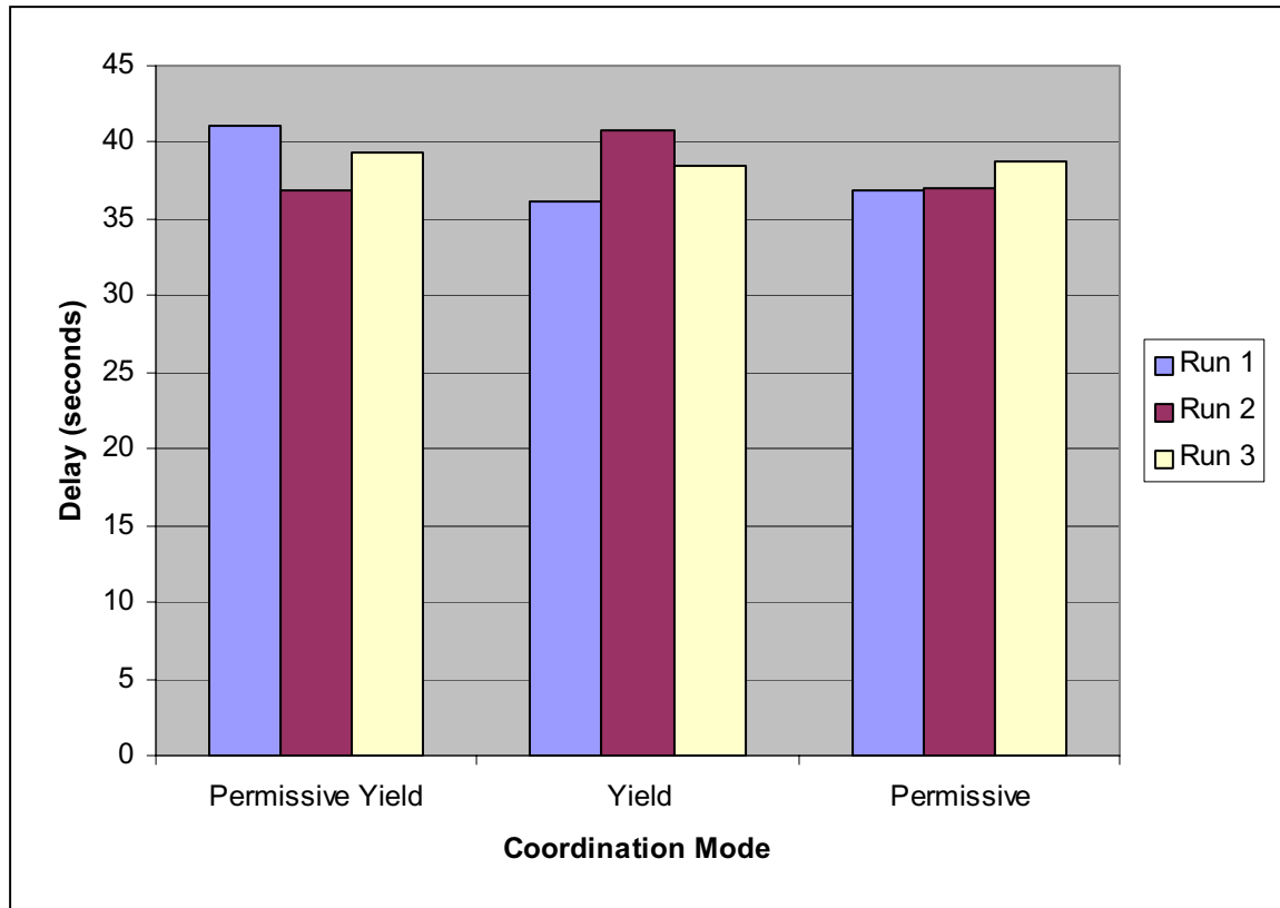
Figure 6 – Total System Delay for Each Coordination Mode
