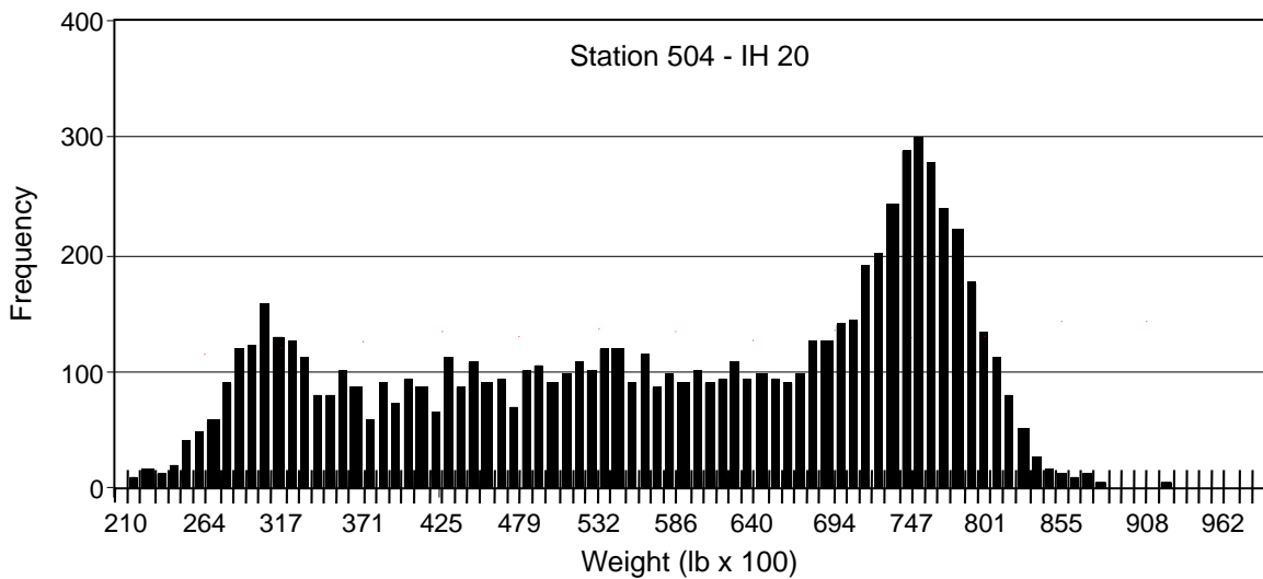
Figure 17. Weight Histogram (Truck 332000) Station 504.
