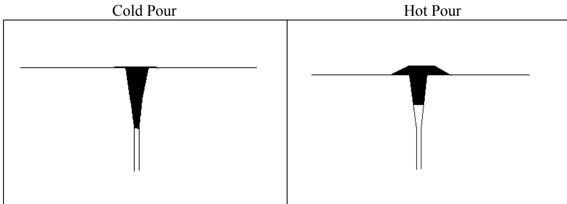
Figure 5.1 Sealing material configurations in the crack
