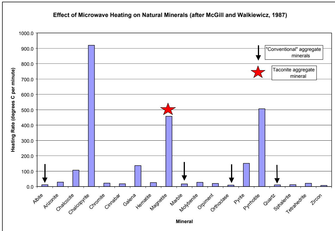
Figure 1.1 Comparison of microwave heating on various minerals (after McGill and Walkiewicz, 1987).
