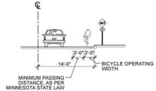
WIDE CURB LANE
