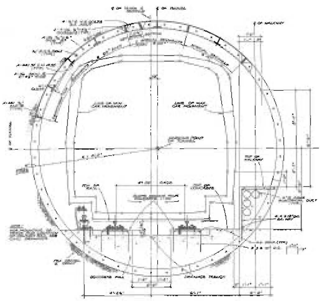
TYPICAL SECTION OF STEEL JOIST PLATE TUNNEL TANGENT TRACK
