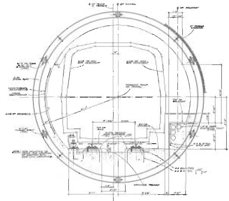
TYPICAL SECTION OF REINFORCED CONCRETE TUNNEL TANGENT TRACK
