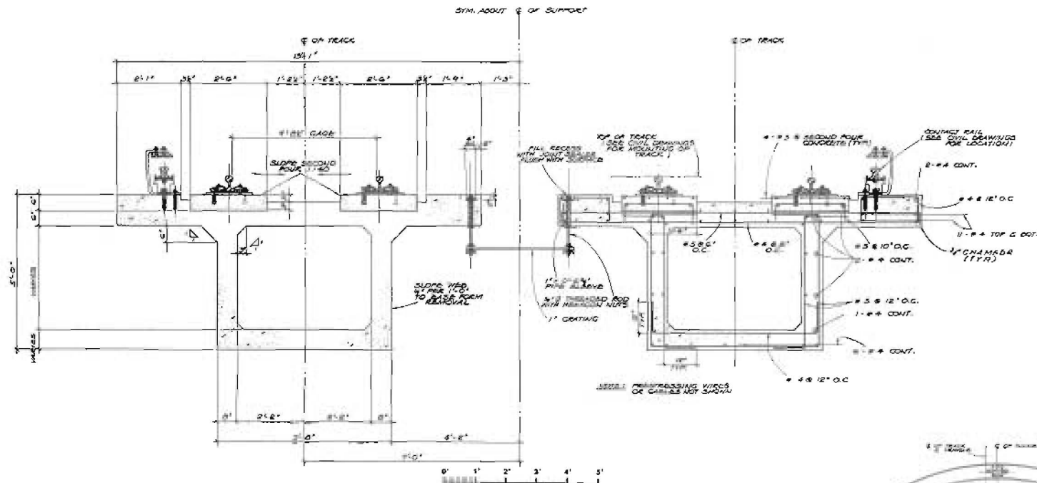
TYPICAL SECTION THROUGH PRESTRESSED AERIAL GIRDERS
