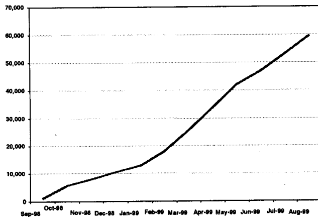
Figure 3-5: Orion VI Hybrid Mileage (5 Buses)
