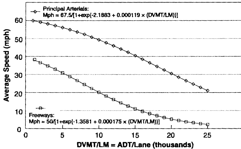
Figure A-10. Average Speed Versus Average Daily Traffic per Lane
