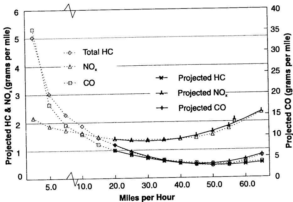
Figure A-13. Emissions as a Function of Average Speed: Low Emissions Scenario, Year 2010
