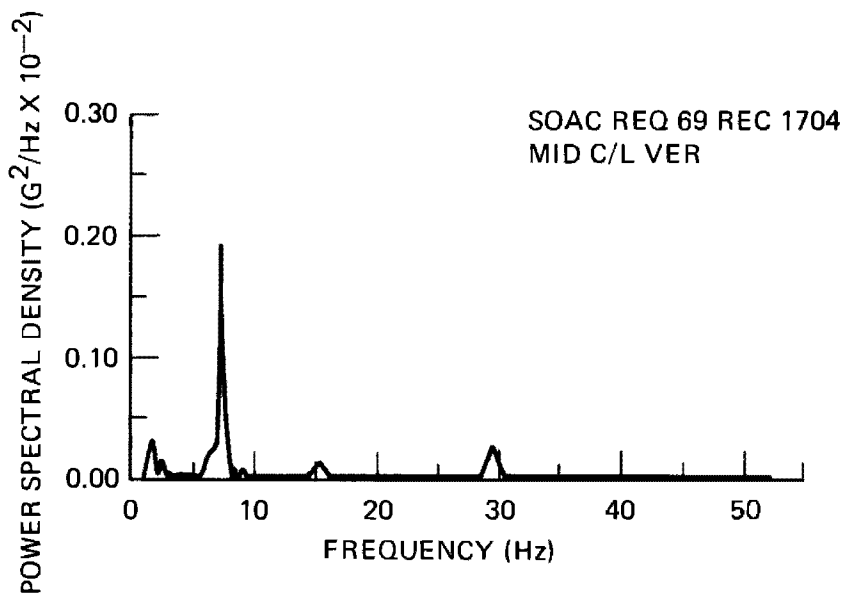
Figure 3-12. Ride Quality Test Baseline Data
