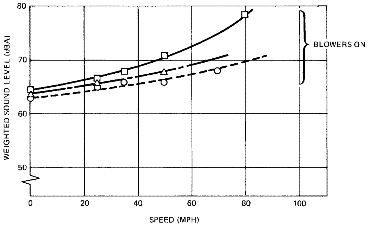
Figure 3-18. Effect of Wheel Configuration on Interior Noise
