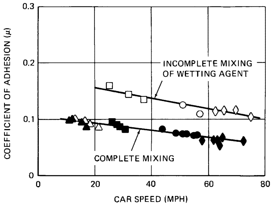
Figure 3-11. Wheel Adhesion
