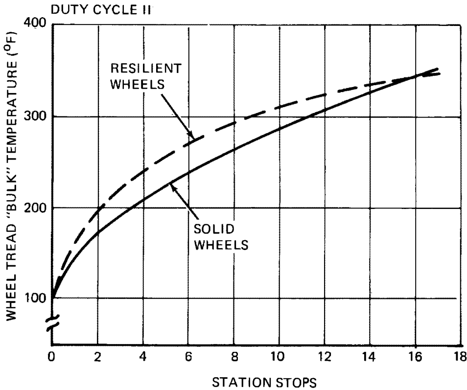
Figure 3-9. Wheel Temperature
