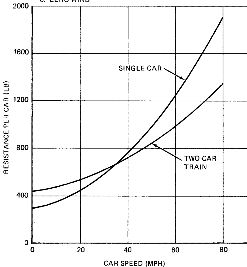
Figure 3-8. Traction Resistance
