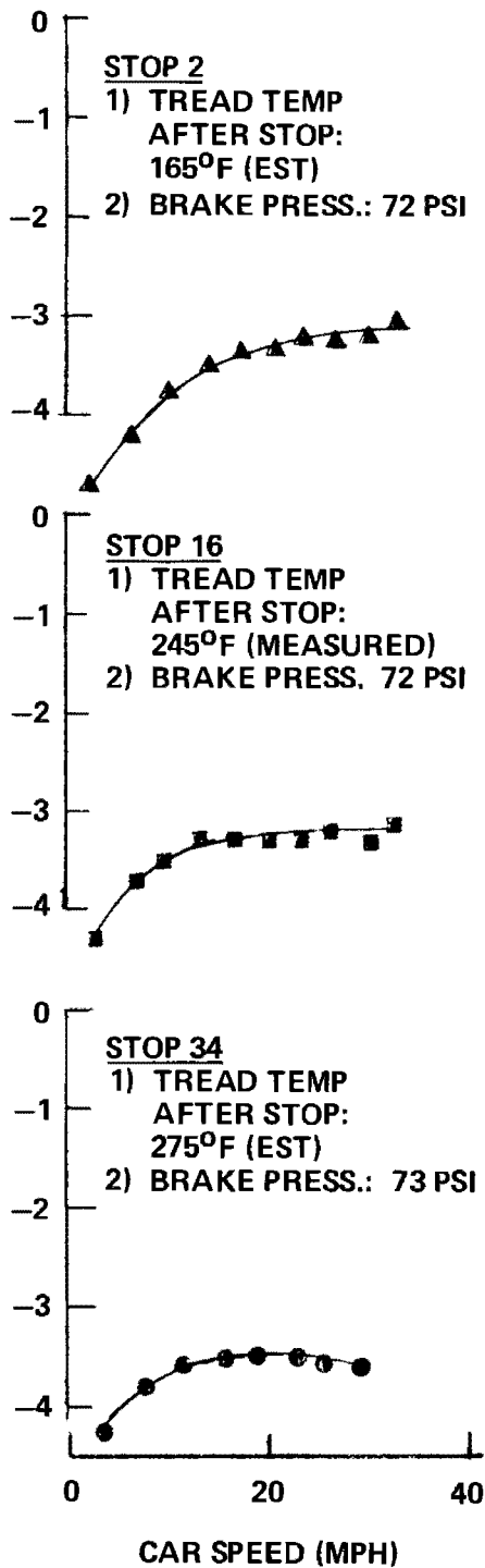
Figure 5-4. Duty Cycle I Friction Braking Deceleration (105,000-Pound Car Braking from 35 MPH)
