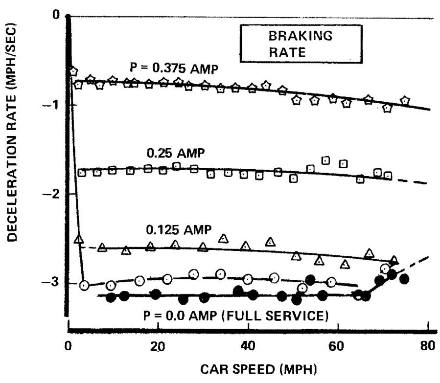
Figure 3-3. Blended Braking Control Characteristics (105,000-Pound Car)
