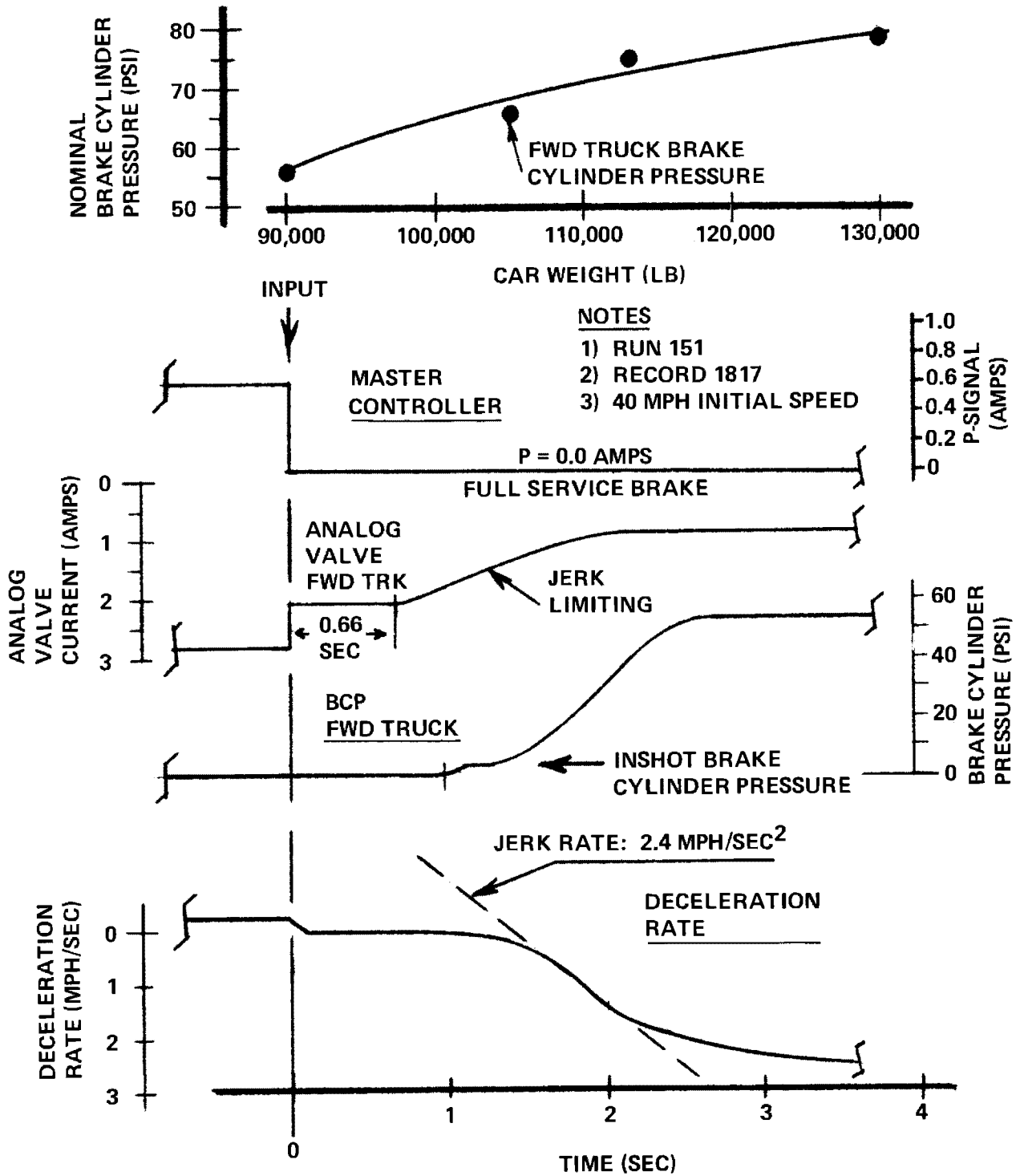
Figure 3-11. Friction Brake Pressure and Application Characteristics
