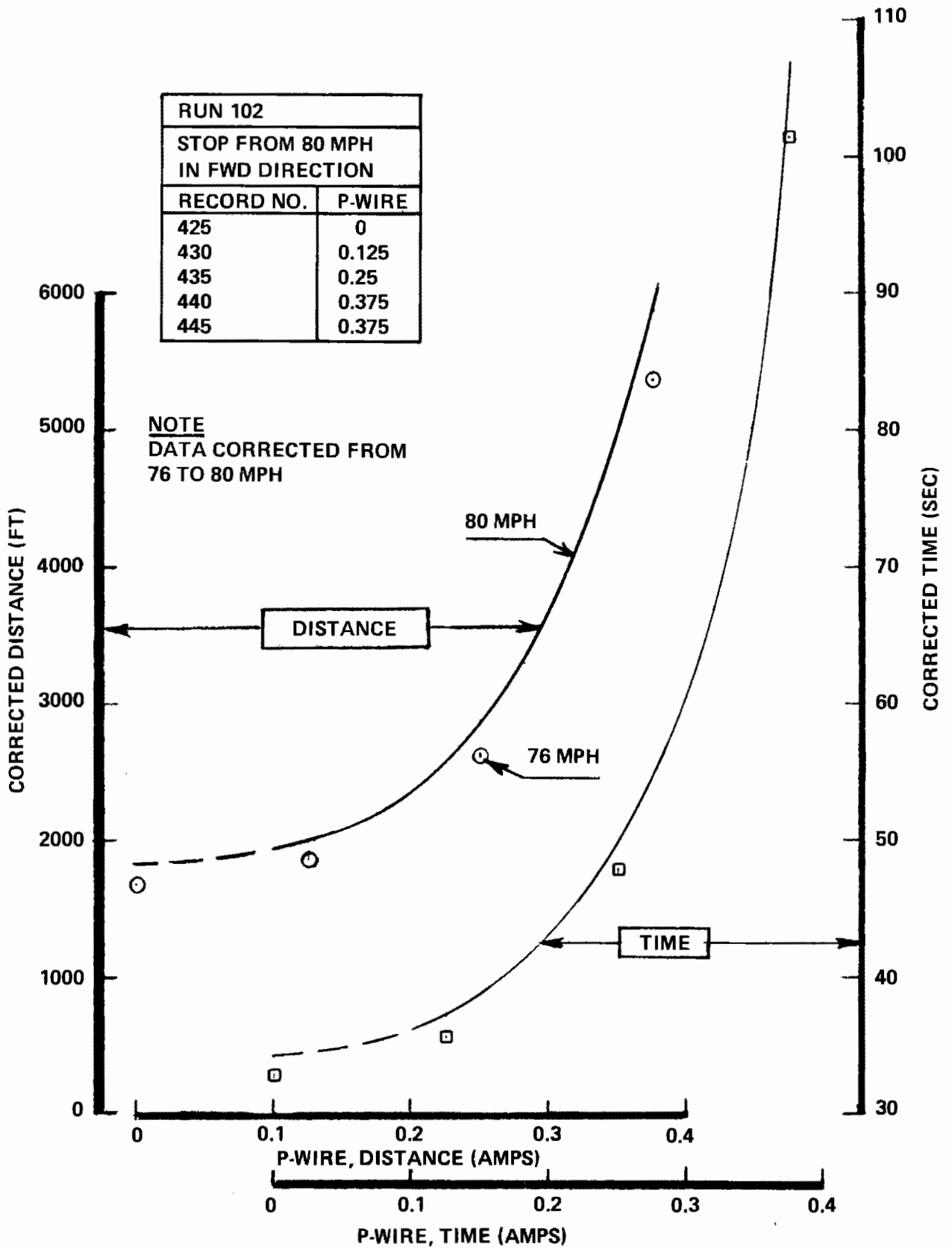
Figure 3-15. Dynamic Braking Stopping Distance
