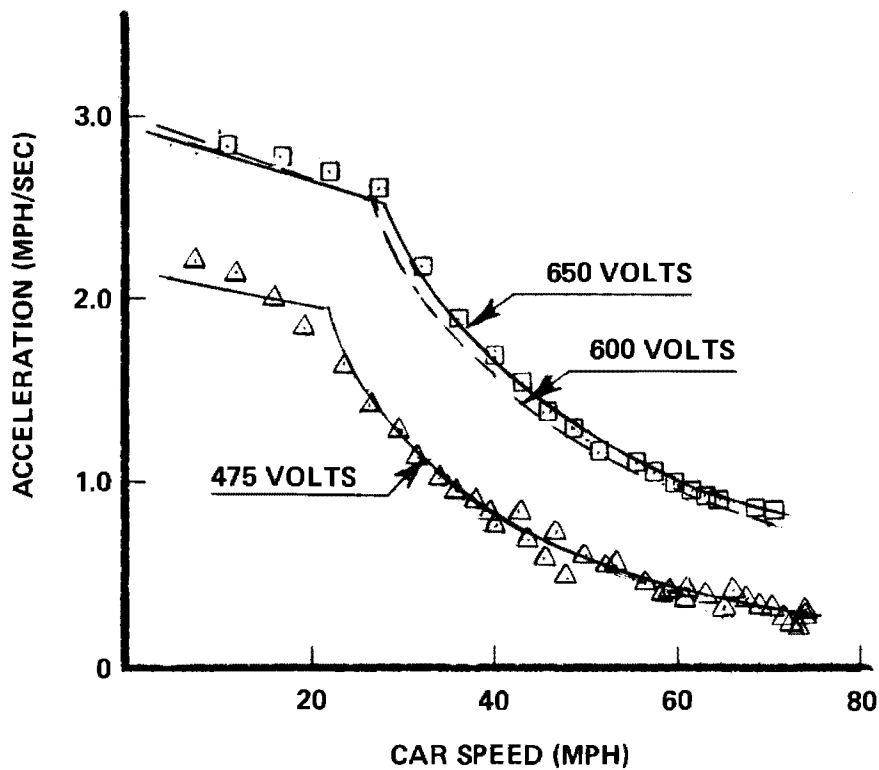
Figure 2-10. Acceleration at Off-Nominal Track Voltage (105,000-Pound Car)
