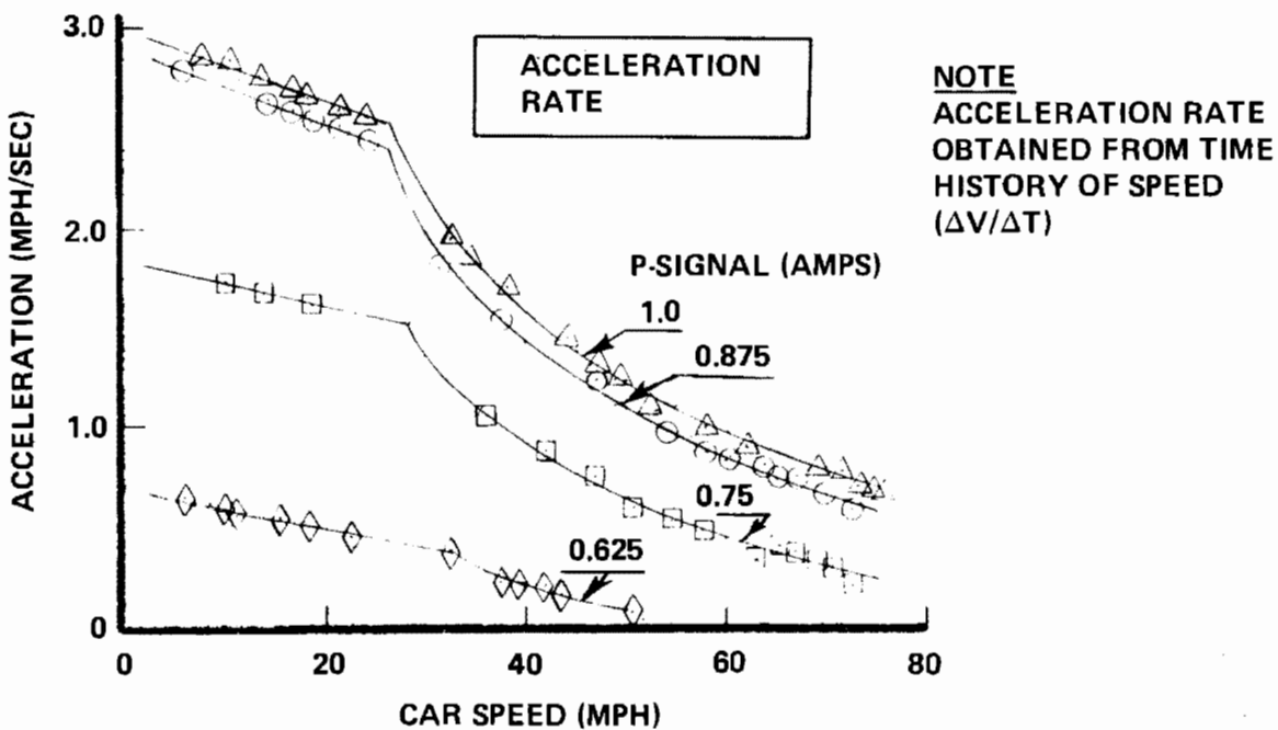
Figure 2-5. Acceleration Control Characteristics (105,000-Pound Car; Nominal 600 Volts)
