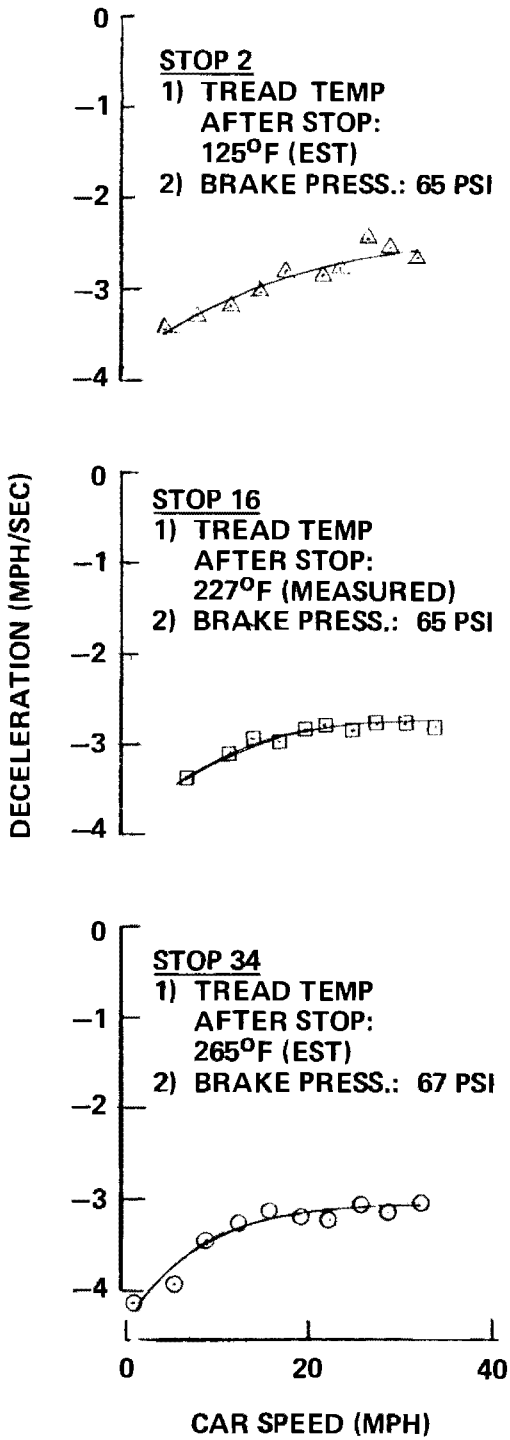
Figure 5-4. Duty Cycle I Friction Braking Deceleration (105,000-Pound Car Braking from 35 MPH)
