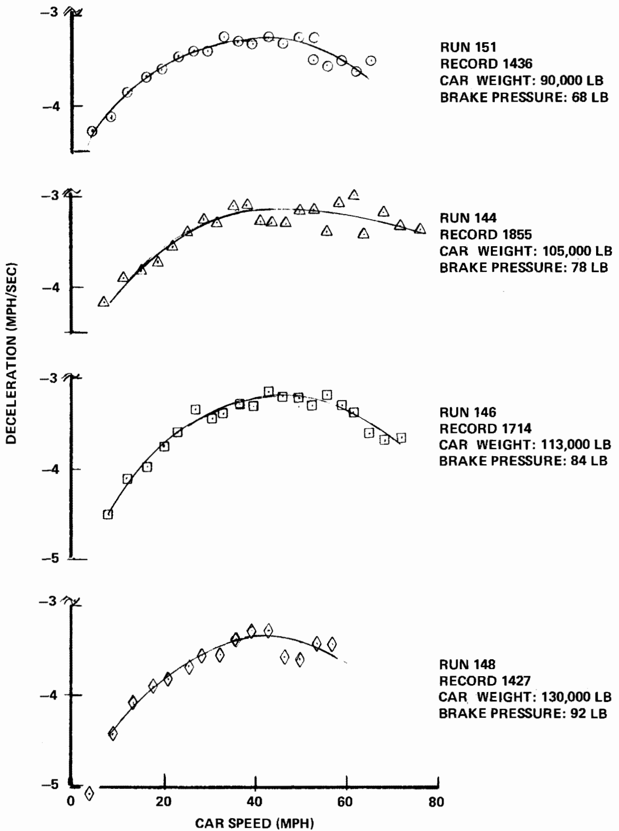
Figure 3-16. Emergency-Friction-Braking Load Weight Compensation
