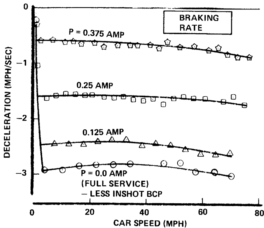
Figure 3-14. Dynamic Braking Only Control Characteristics (105,000-Pound Car)
