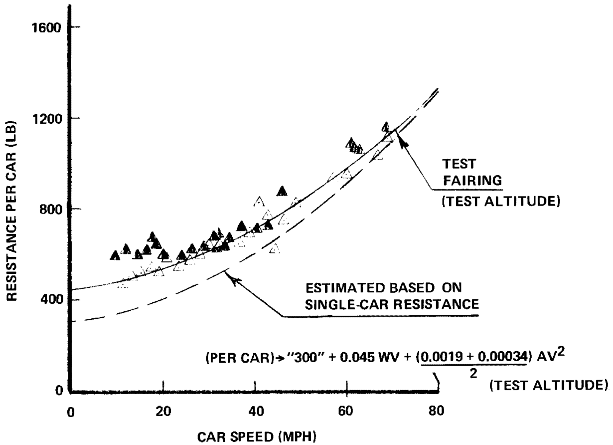
Figure 4-2. Traction Resistance (105,000-Pound Two-Car Train)
