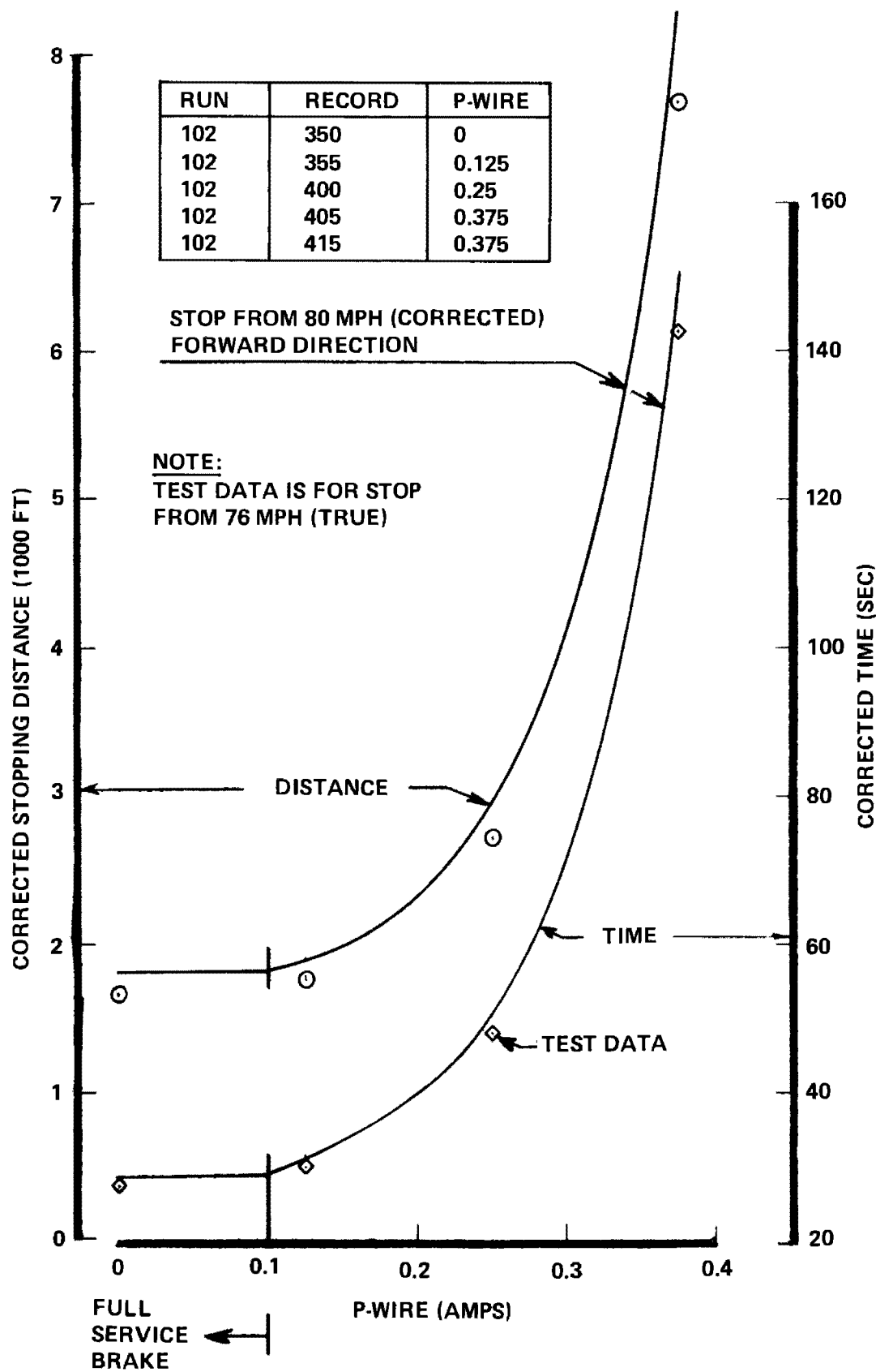
Figure 3-10. Friction Braking Stopping Distance (105,000-Pound Car)
