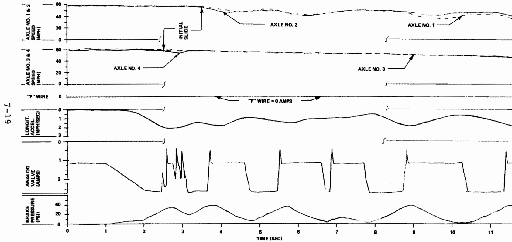
Figure 7-4. Deceleration of 90,000-Pound High-Density Car with Friction Brakes Only on Wetted Rails
