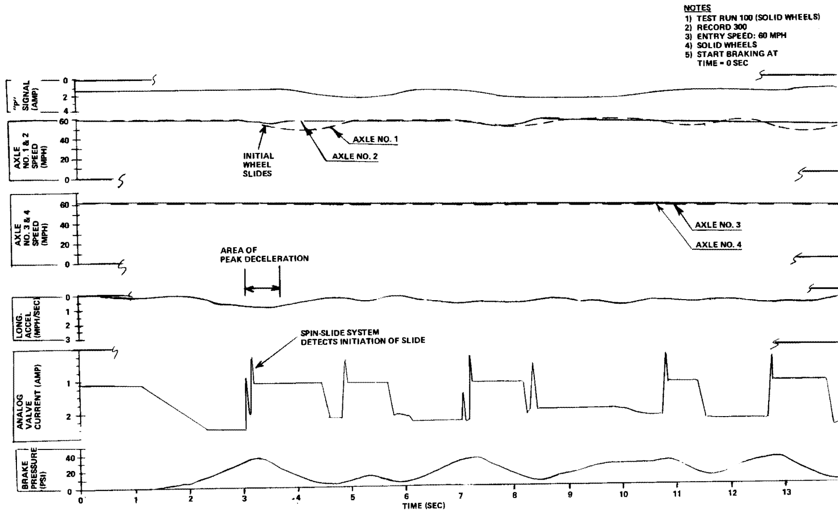
Figure 8-1. Adhesion of 90,000-Pound Car on Wetted Rails During Deceleration with Friction Brakes Only (Friction Braking on Aft Truck Cut Out for Adhesion Tests)
