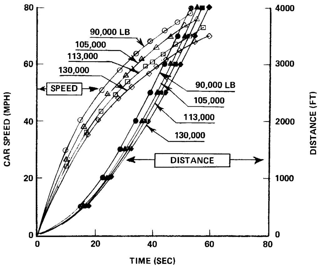
Figure 2-9. Time-, Distance-, and Speed-to-Accelerate Car Weight Effects
