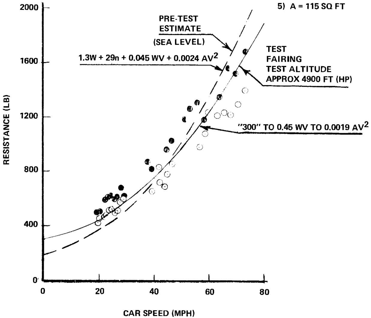
Figure 4-1. Traction Resistance (105,000-Pound Single Car)
