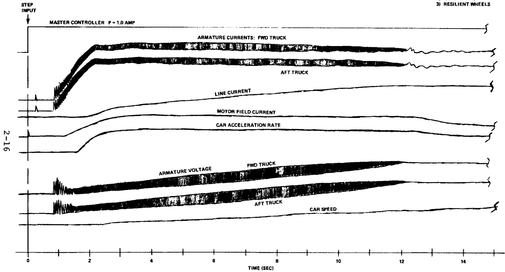
Figure 2-4. Time History of Typical Initial Acceleration (105,000-Pound Car; 600 Volts)
