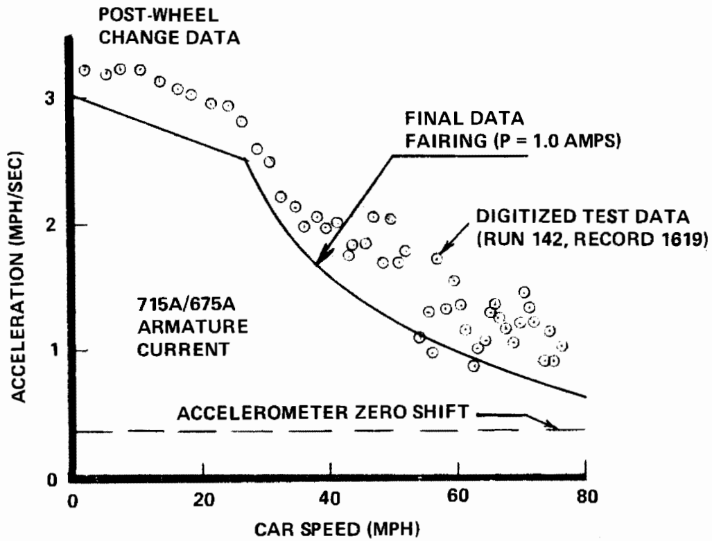
Figure 2-1. Performance Level and Data Reduction Problem Areas (105,000-Pound Car; Nominal 600 Volts)
