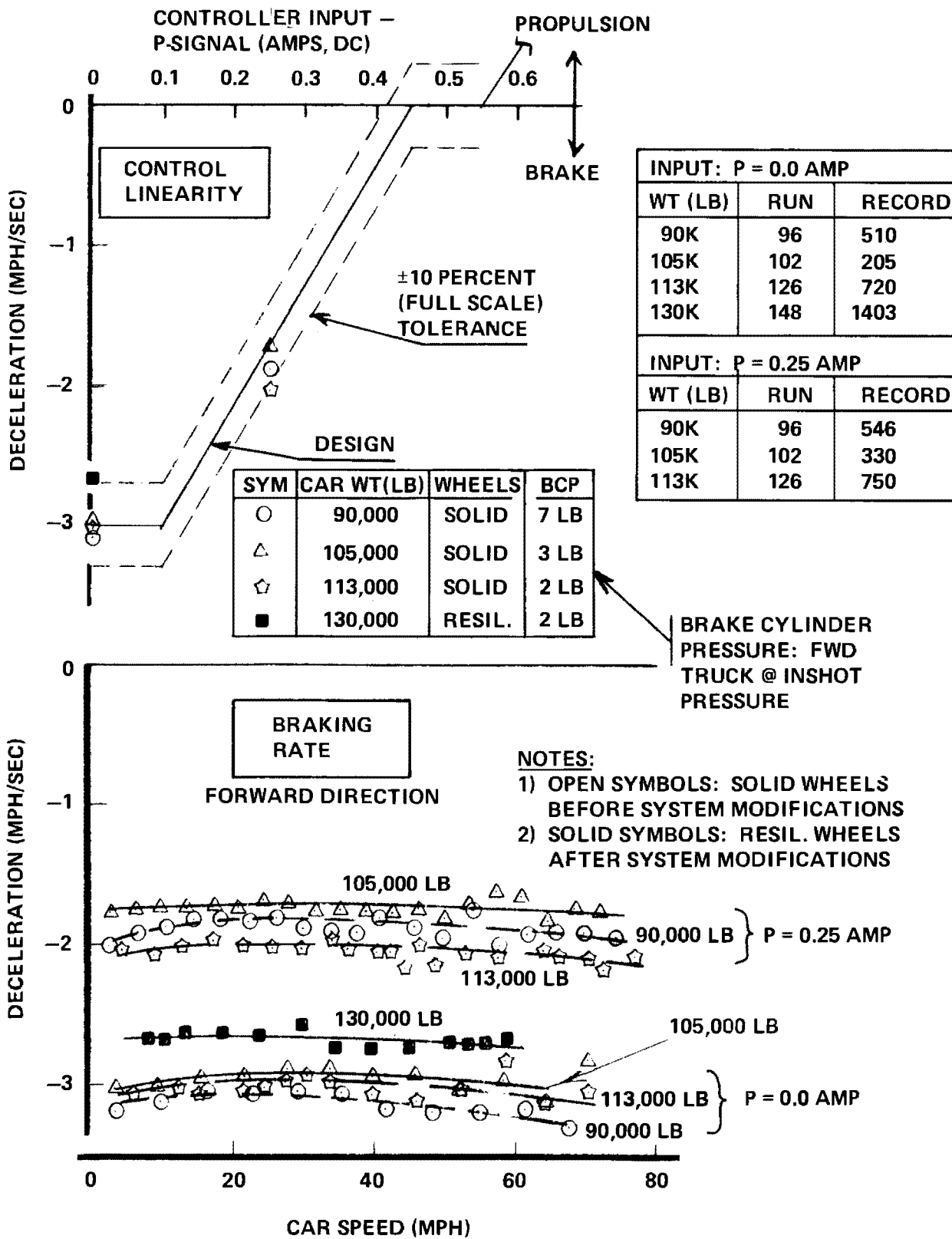
Figure 3-6. Blended Braking Load Weight Compensation
