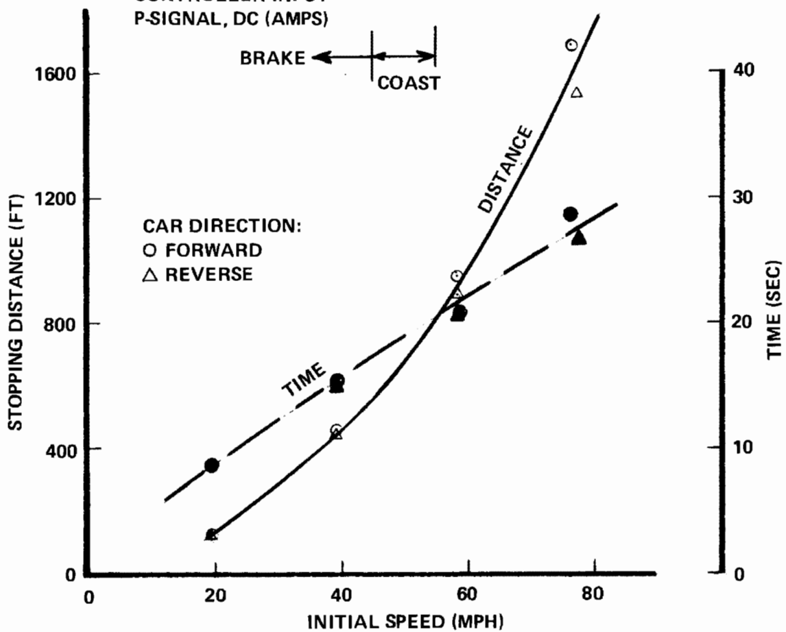
Figure 3-4. Blended Braking Stopping Distance (105,000-Pound Car)
