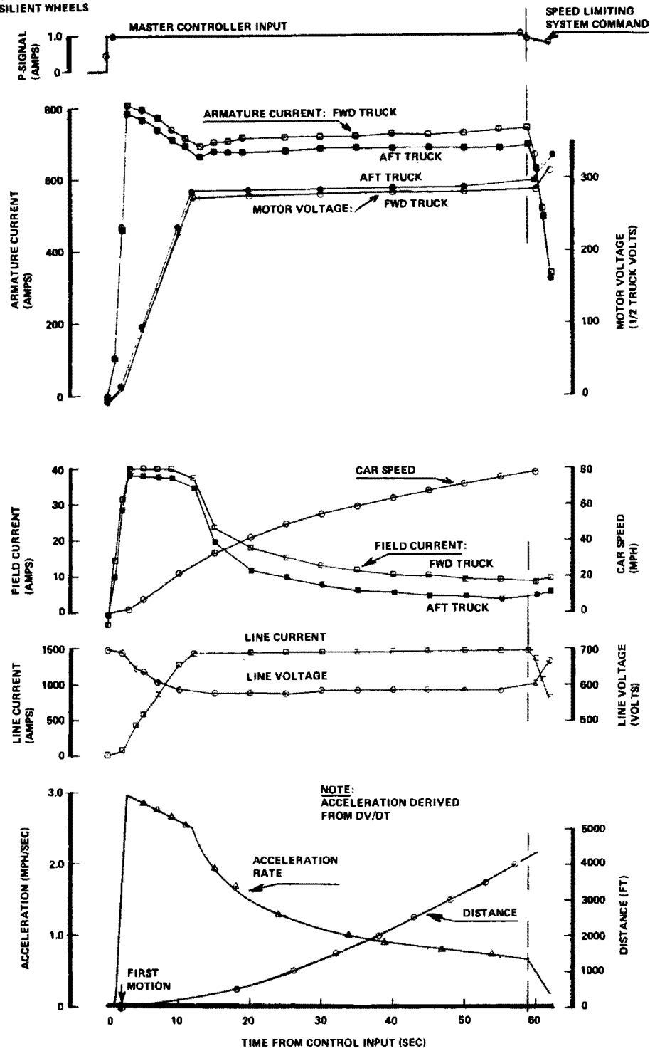
Figure 2-3. Typical Maximum Acceleration Digitized Data (105,000-Pound Car; Nominal 600 Volts)
