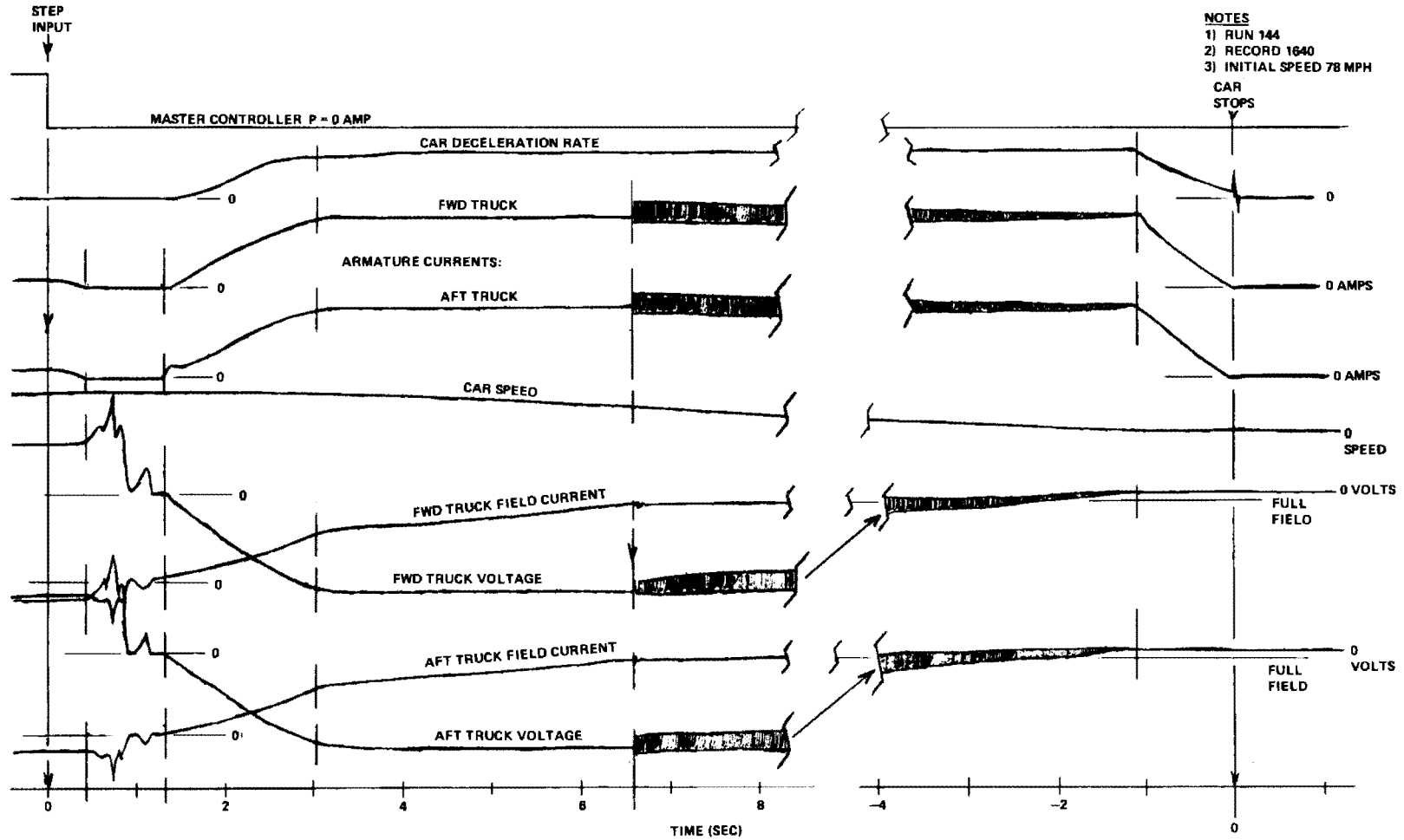
Figure 3-2. Time History of Typical Blended Braking
