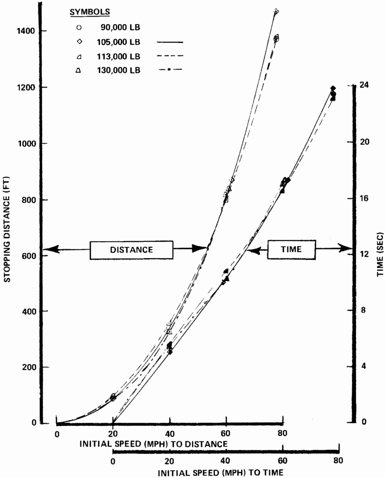
Figure 3-17. Emergency Braking Stopping Distance
