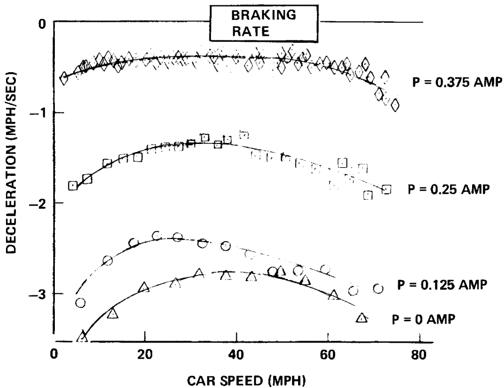
Figure 3-9. Friction Braking Only Control Characteristics (105,000-Pound Car)
