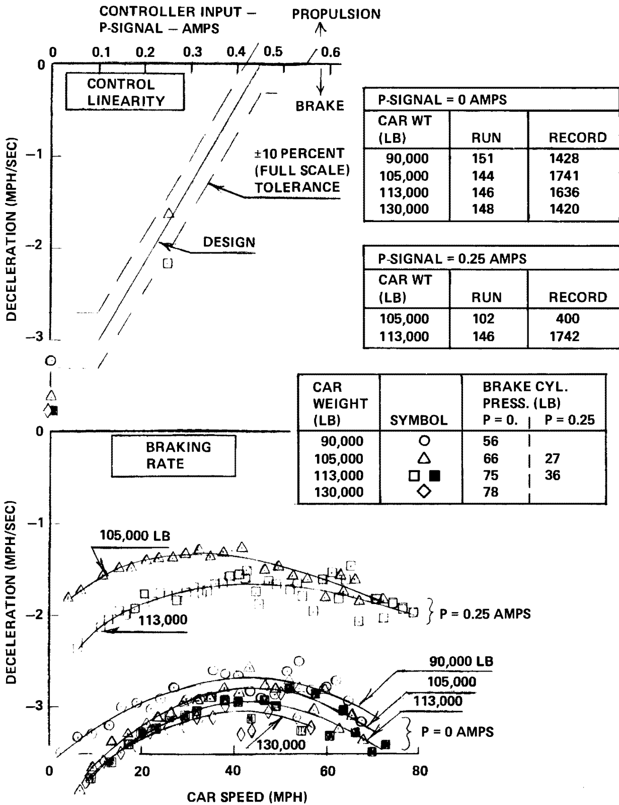
Figure 3-12. Friction-Braking-Only Load Weight Compensation
