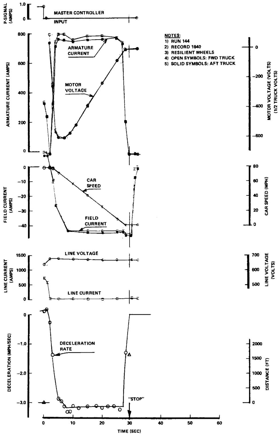
Figure 3-1. Typical Blended Deceleration Digitized Data (105,000-Pound Car).
