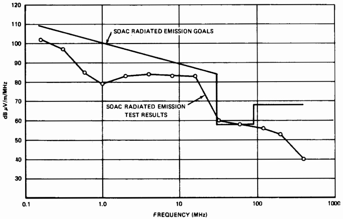
Figure 3-1. Electromagnetic Field Test Data
