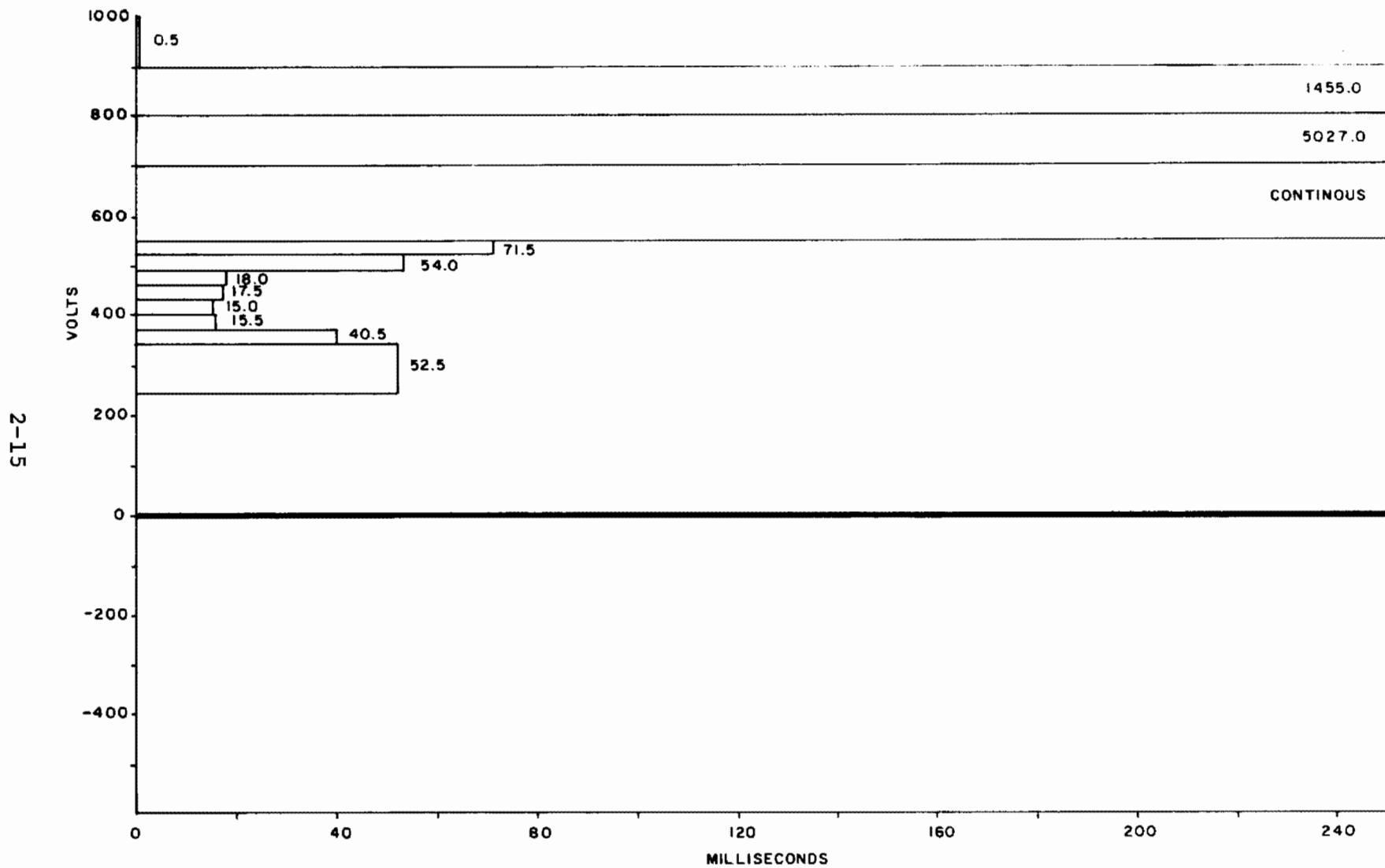
Figure 2-14. Transient Events, Maximum Amplitude (Observed) Duration Distribution (All Conditions; Instrumentation on Board; 5481.0-Second Test Duration)
