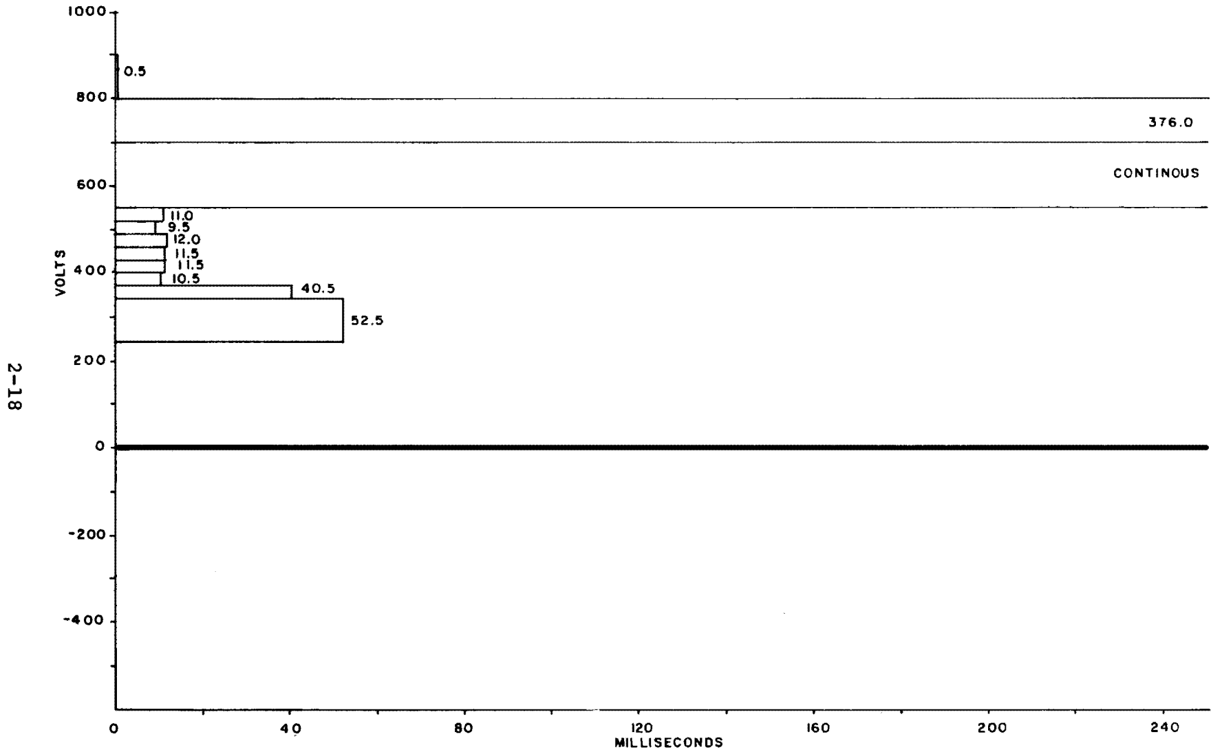
Figure 2-17. Transient Events, Maximum Amplitude (Observed) Duration Distribution (Morning Run; Instrumented Car Pulling; 1729.5-Second Test Duration)
