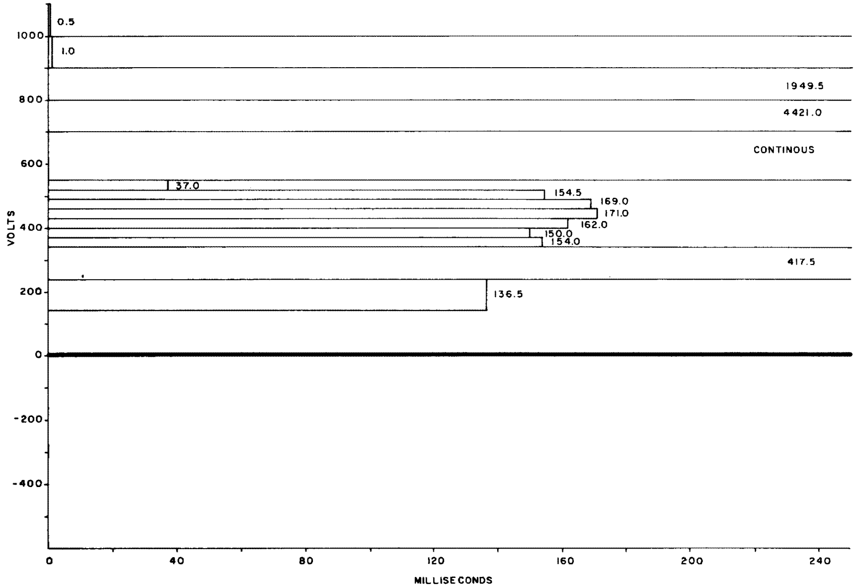
Figure 2-15. Transient Events, Maximum Amplitude (Observed) Duration Distribution (All Conditions; Instrumentation Trackside; 1050.0-Second Test Duration)
