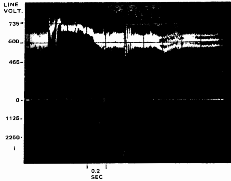
Figure 2-10. Train Passing South Rail Gap (Trackside Measurement)
