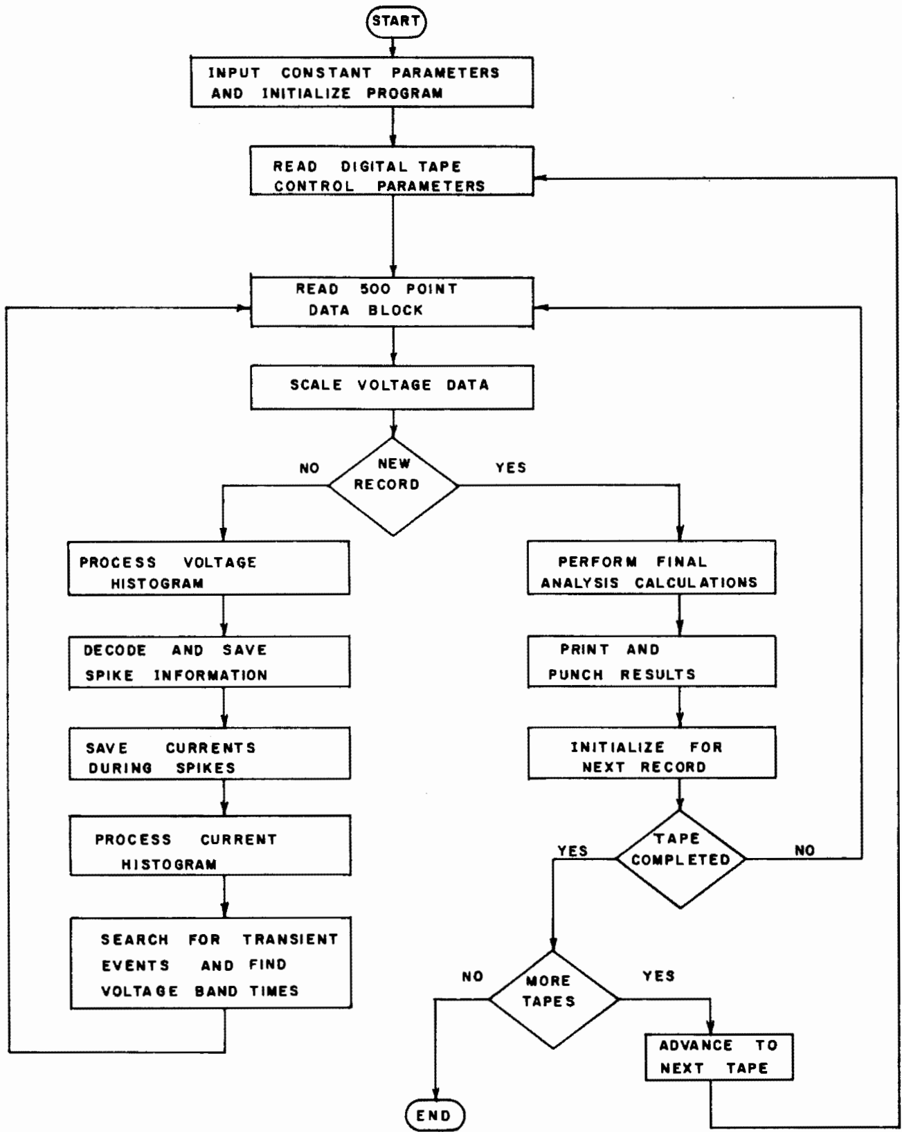
Figure A-12. General Flow Chart for "SUBWAY 1" Program (Main Computer Analysis Program)
