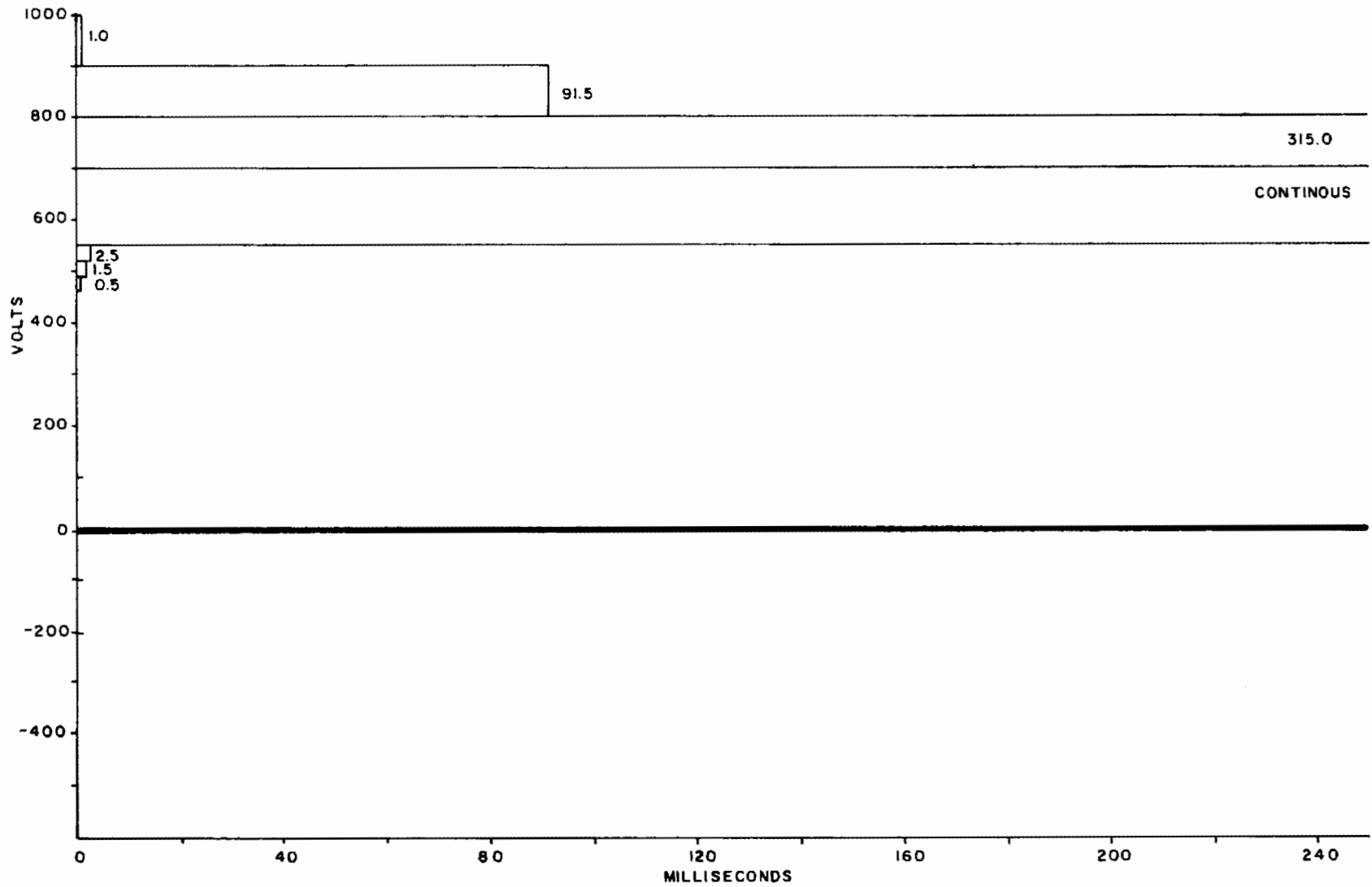
Figure 2-20. Transient Events, Maximum Amplitude (Observed) Duration Distribution (Afternoon Trackside Run; Car Out of Area; 280.5-Second Test Duration)
