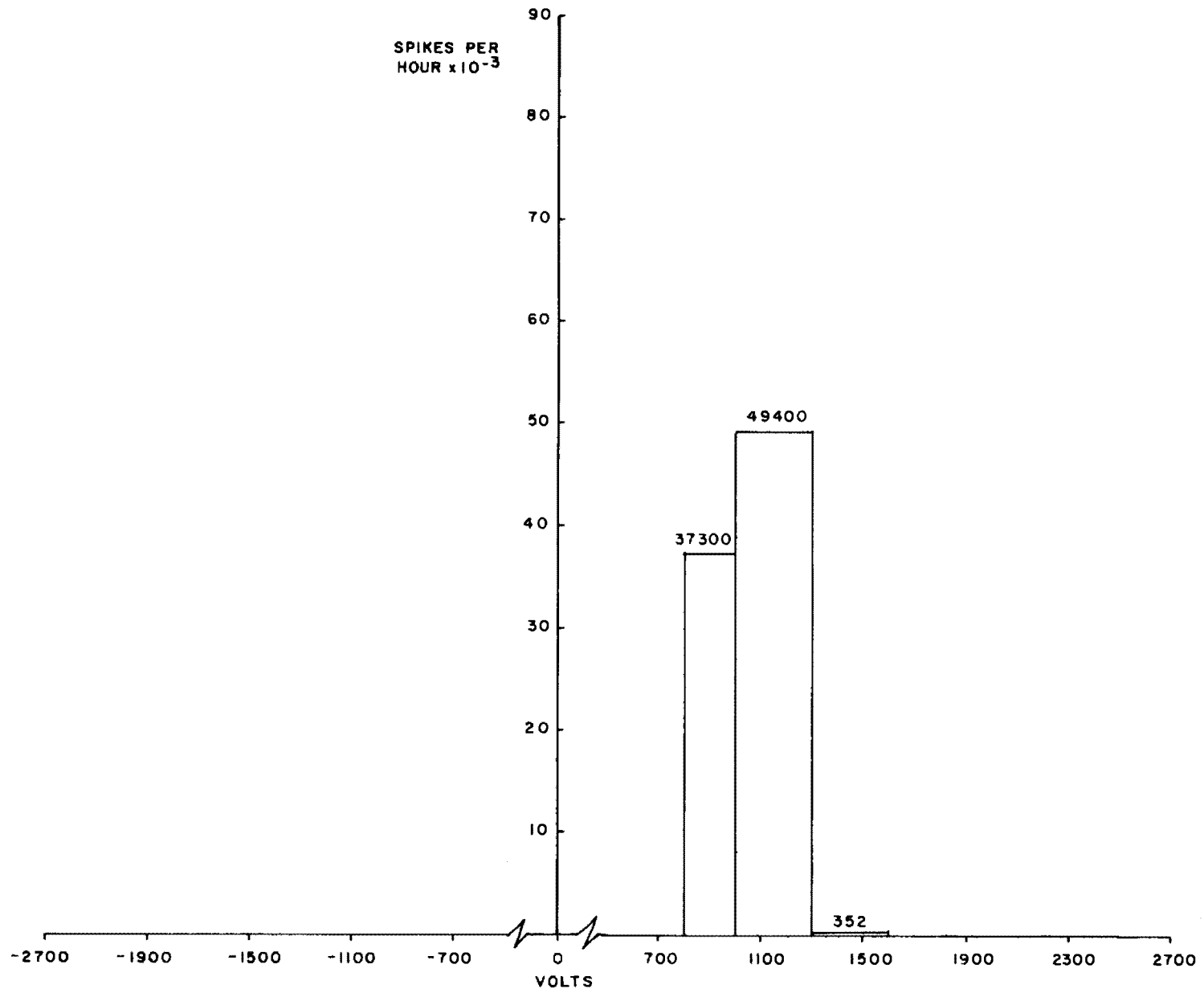
Figure 2-21. Spike Voltage (Observed) Distribution (Morning Total Envelope; 5481.0-Second Test Duration)
