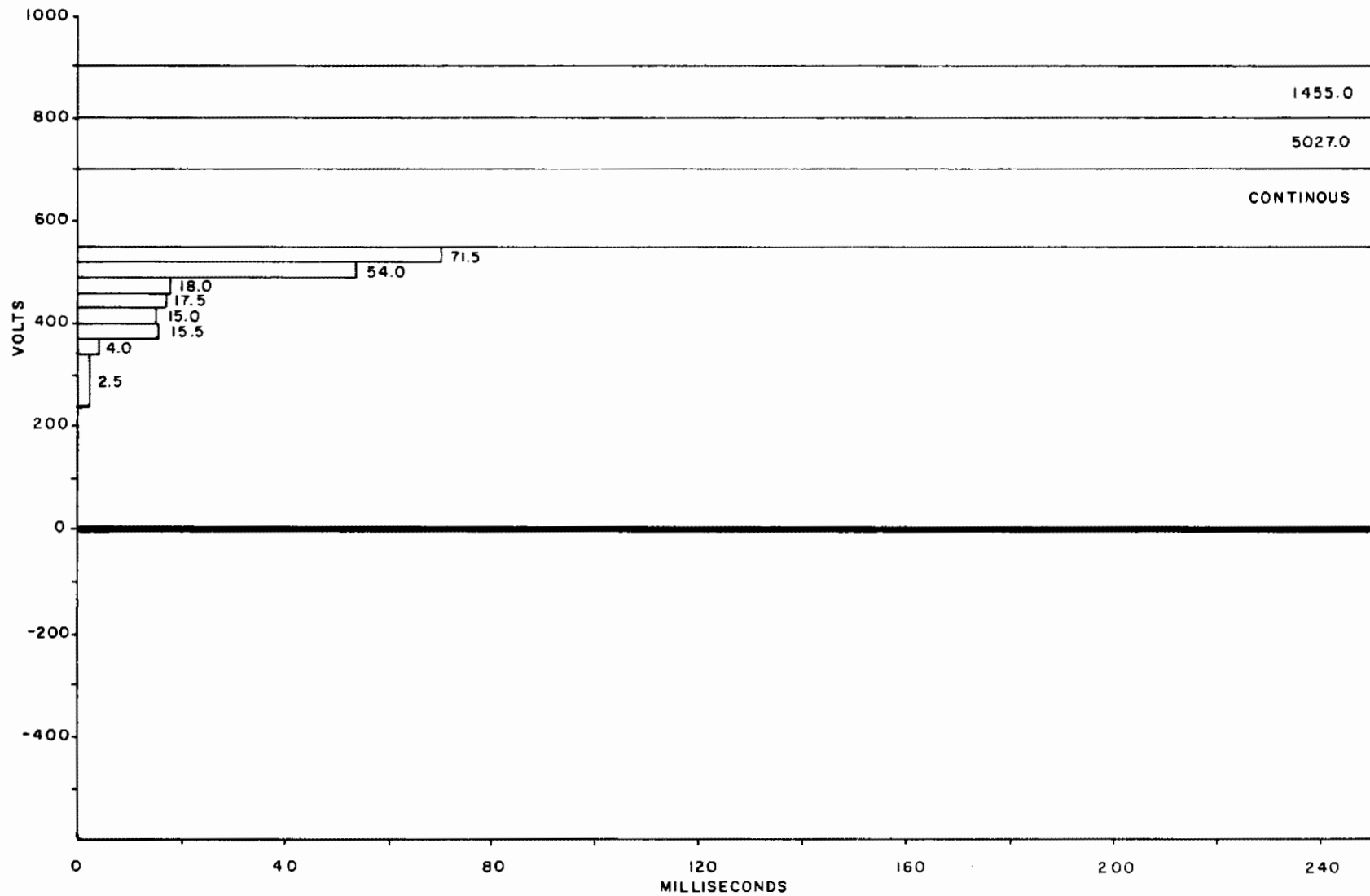
Figure 2-16. Transient Events, Maximum Amplitude (Observed) Duration Distribution (Morning Run; Both Cars Energized; 2384.5-Second Test Duration)
