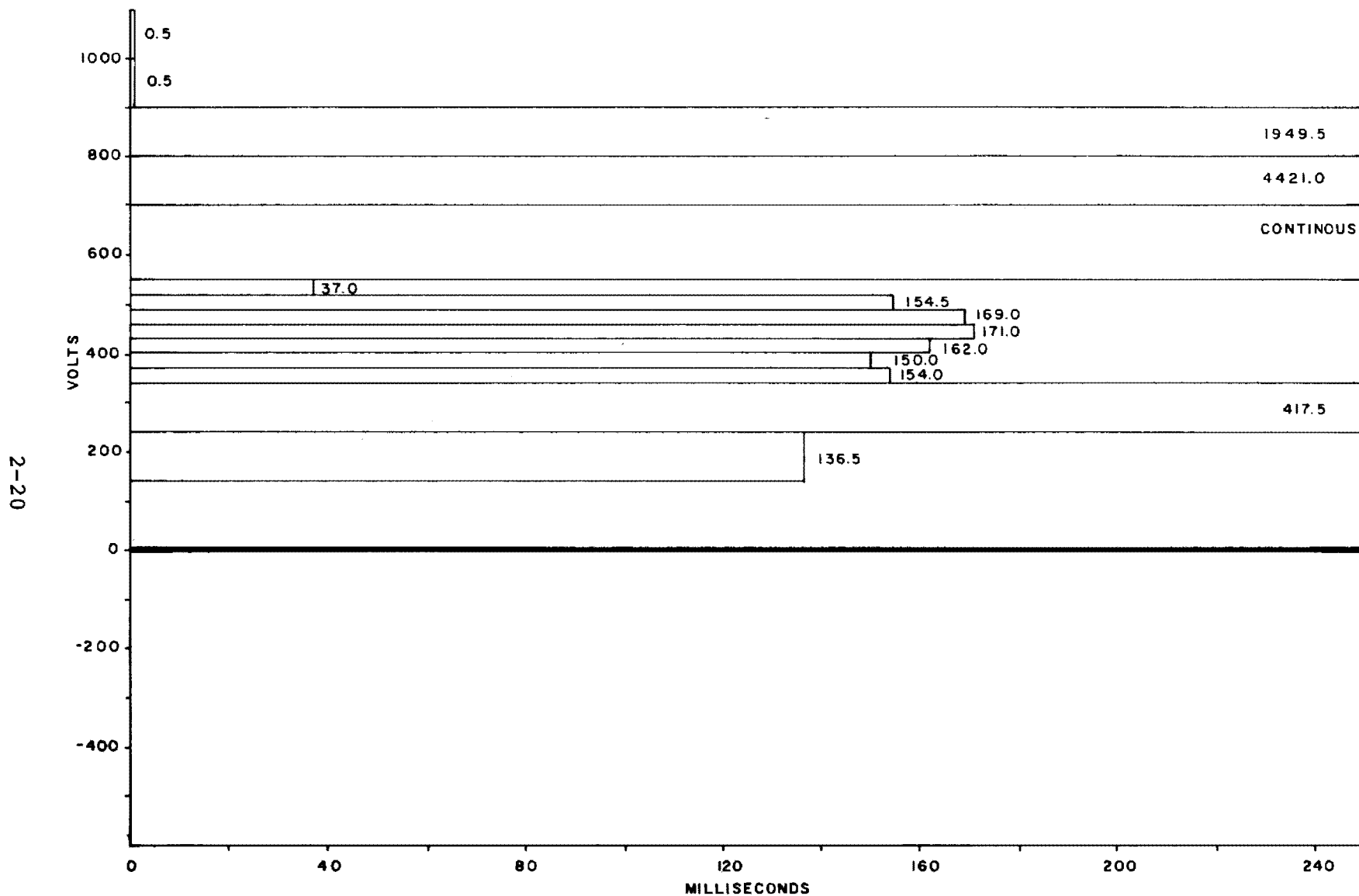
Figure 2-19. Transient Events, Maximum Amplitude (Observed) Duration Distribution (Afternoon Trackside Run; Car in Area or Passing Test Site; 769.5-Second Test Duration)
