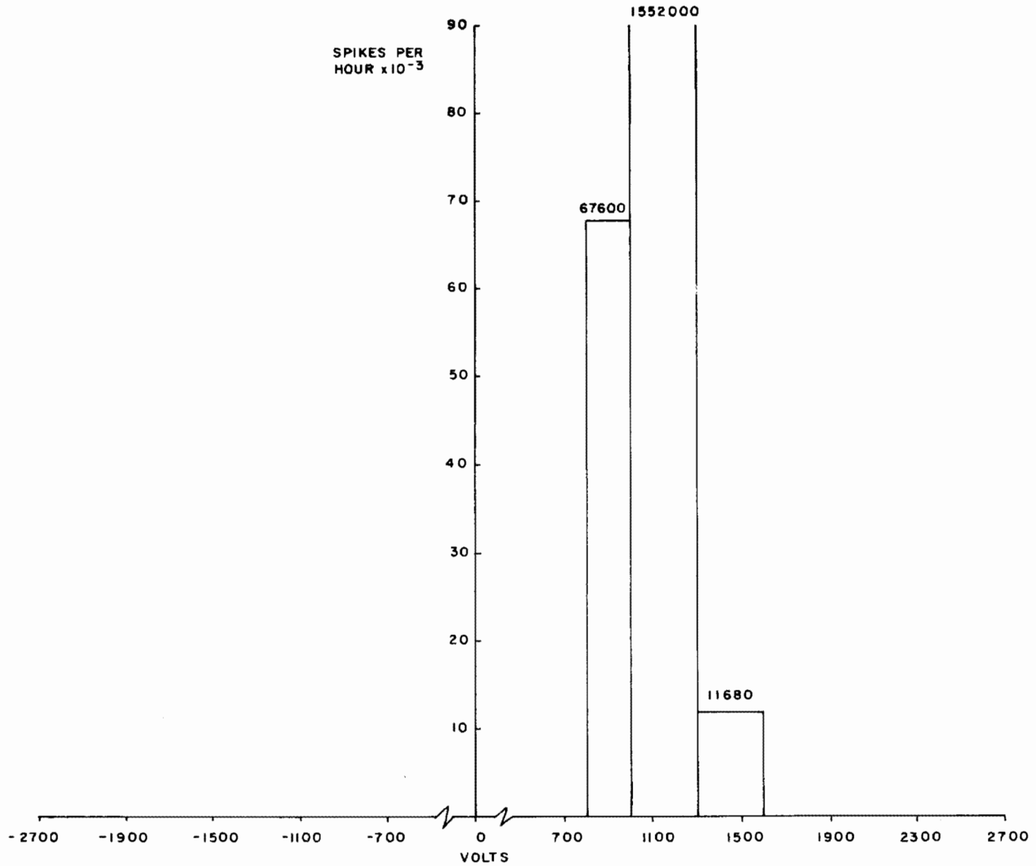
Figure 2-27. Spike Voltage (Observed) Distribution (Trackside; Car Out of Area; 280.5-Second Test Duration)
