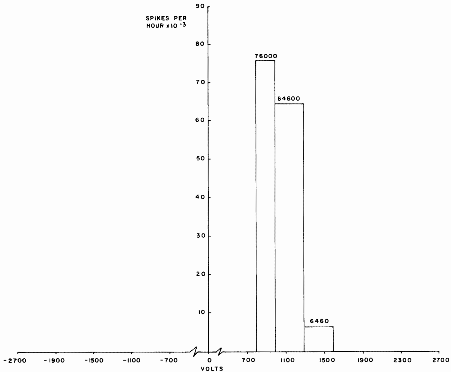
Figure 2-22. Spike Voltage (Observed) Distribution (Afternoon Total Envelope; Trackside Results; 1050.0-Second Test Duration)
