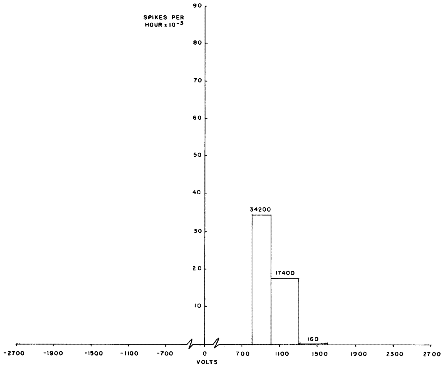
Figure 2-23. Spike Voltage (Observed) Distribution (Both Cars Pulling; 2384.5-Second Test Duration)
