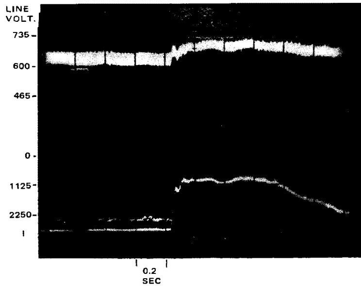
Figure 2-8. Minor Decrease of Power (Instrumented Car Pulling)
