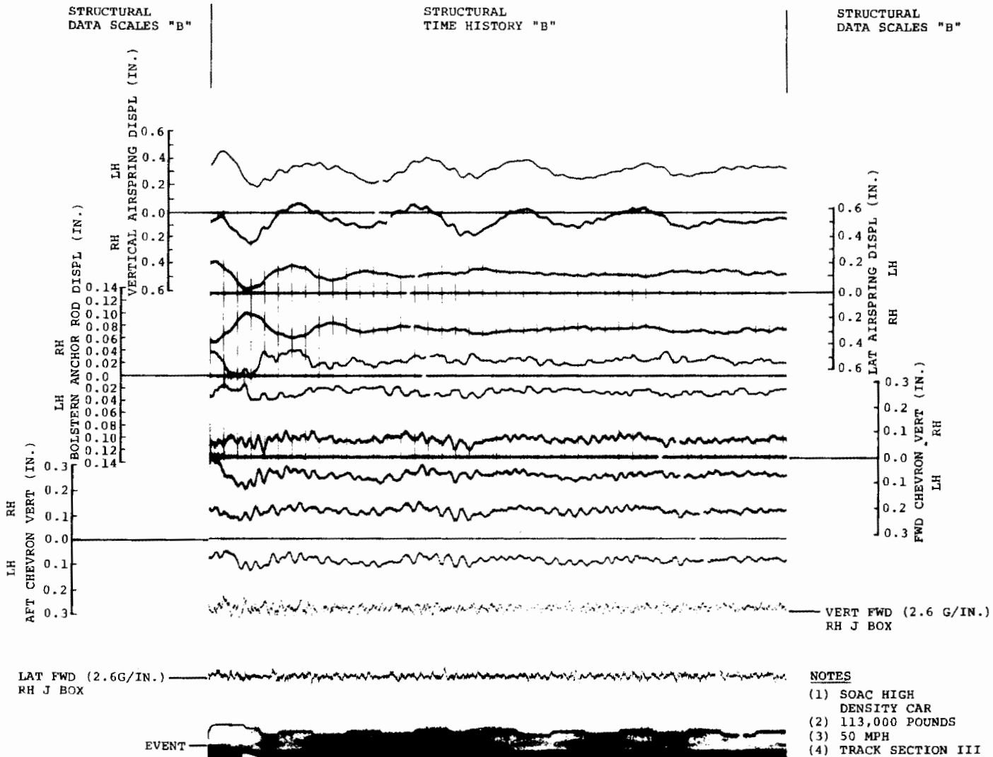
Figure 1-2. Sample Data Record (Sheet 2 of 2)
