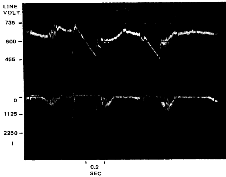
Figure 2-1. North Rail Gap Transient
