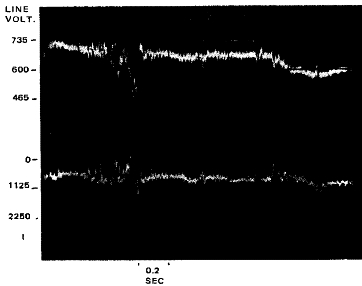
Figure 2-2. Representative Transients in North Turn
