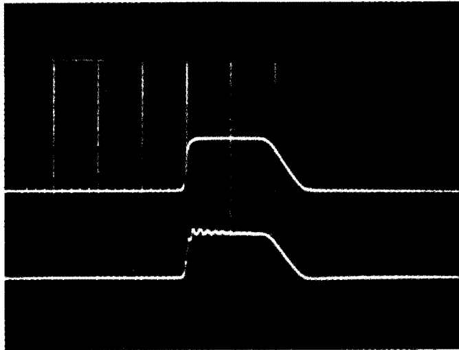
Figure A-4. Spike Probe and Cable Response
