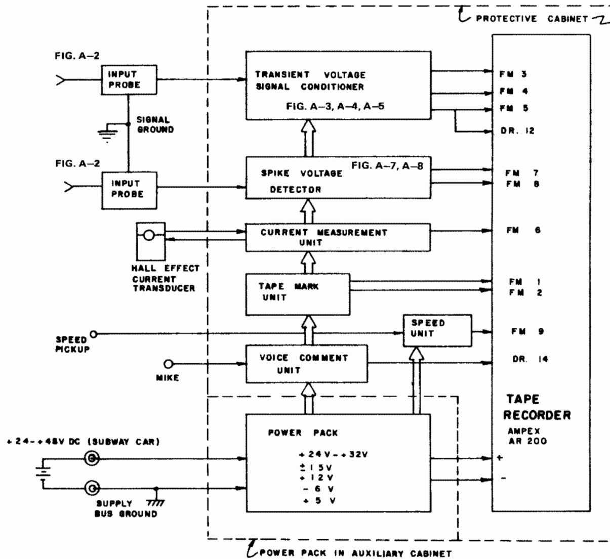
Figure A-1. General Block Diagram for Rapid Transient Recording System Voltage Transients and Spikes
