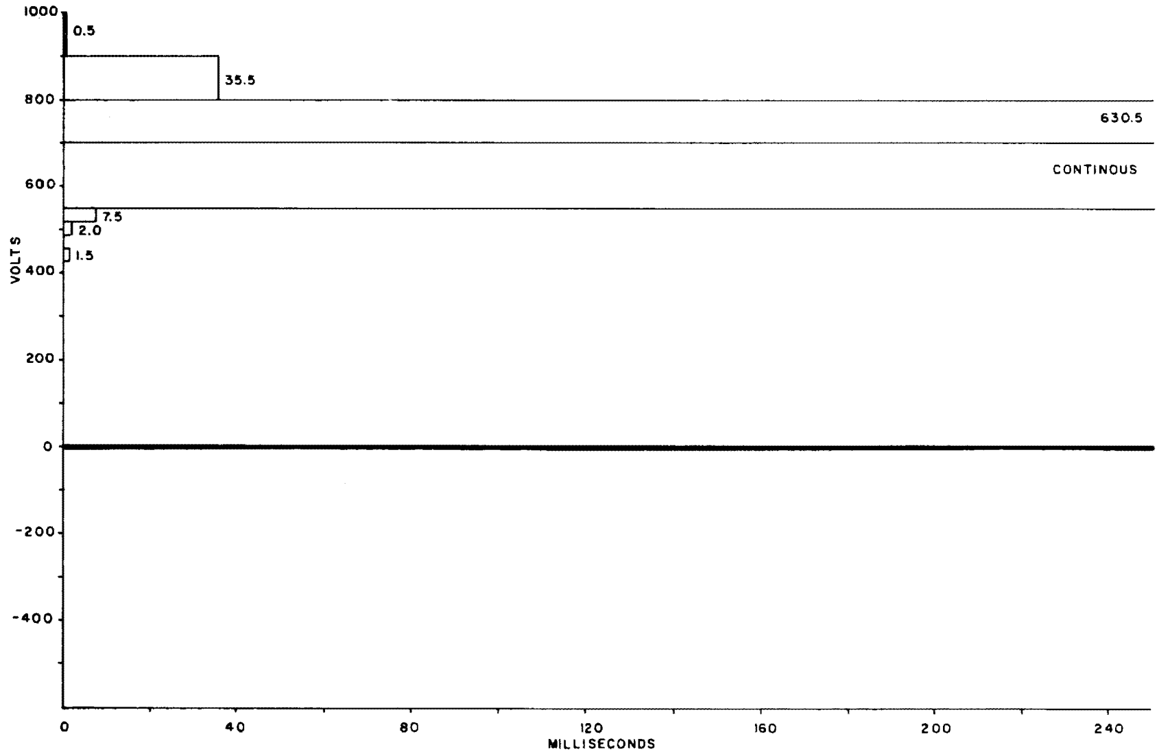
Figure 2-18. Transient Events, Maximum Amplitude (Observed) Duration Distribution (Morning Run; Instrumented Car Being Pulled; 1367.0-Second Test Duration)
