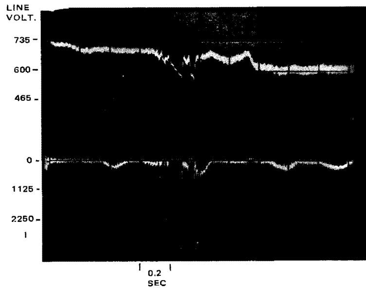
Figure 2-7. Representative Transients (Instrumented Car Being Pulled)
