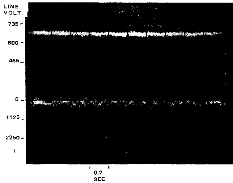
Figure 2-3. Noise Near Locomotive Generator
