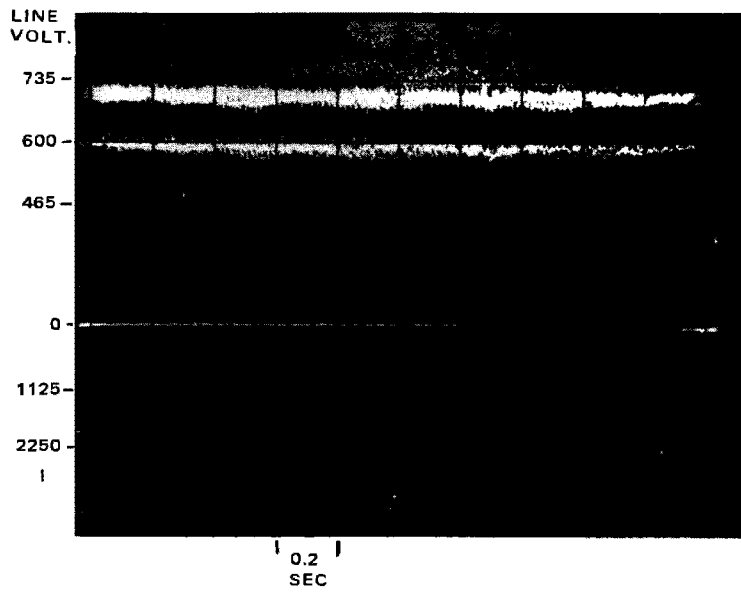
Figure 2-13. Train Located Outside Instrumented Track Section (Trackside Measurement)
