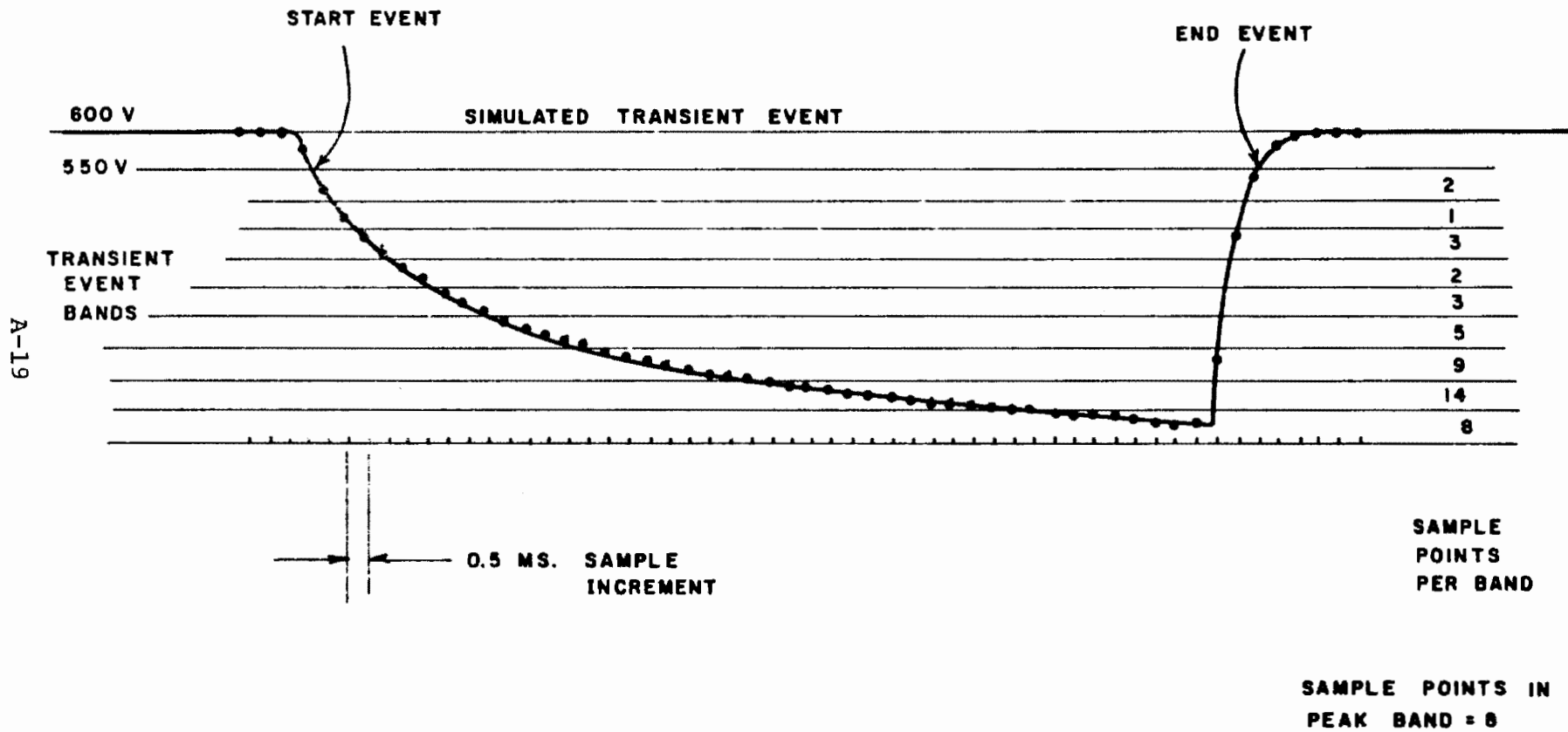
Figure A-14. Application of the Transient Algorithm to a Simulated Transient Event
