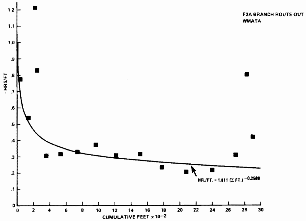
Figure 5-5. Rate of Advance vs Cumulative Tunnel Length
