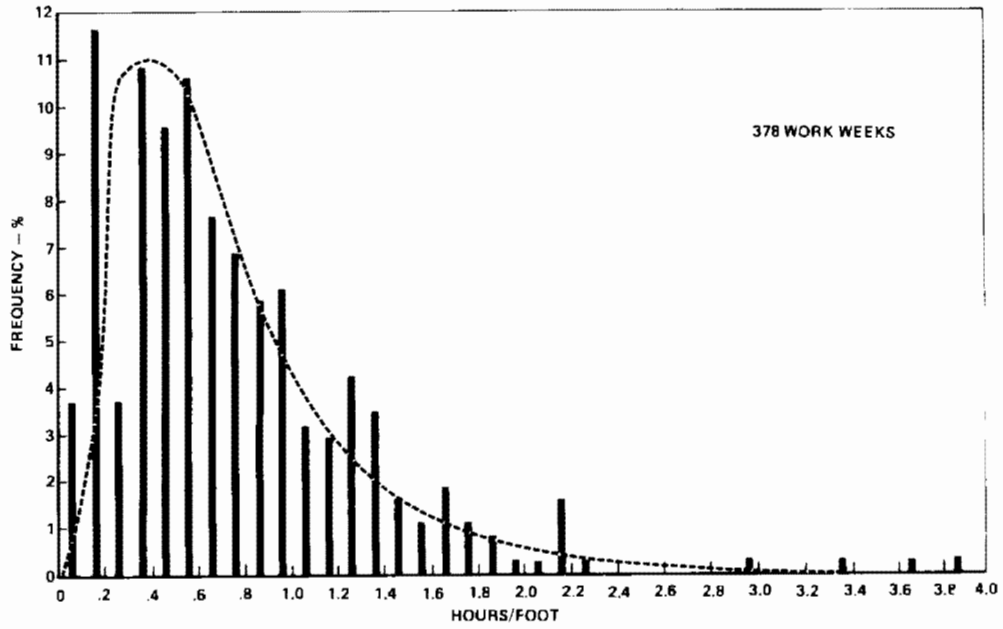
Figure 5-10. Distribution of Weekly Average Rates of Advance
