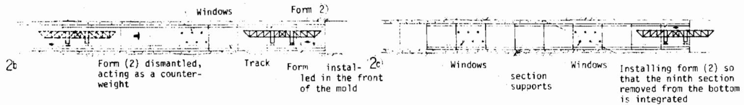
FIGURE B-4. FILTERING RHYTHM AND MOVEMENT SEQUENCE OF THE MOLD SECTIONS
