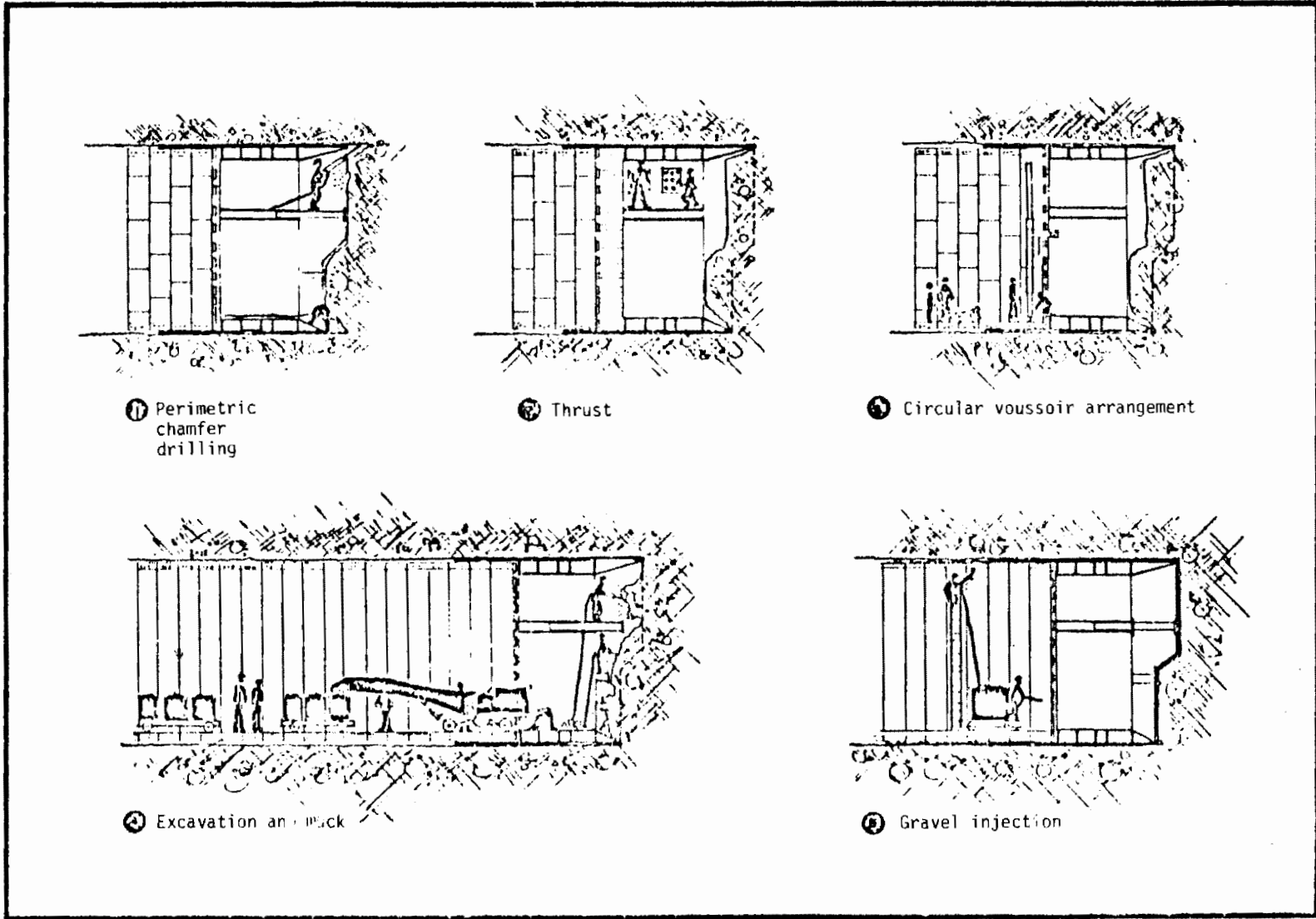
FIGURE B-3. CENTRAL INTERCEPT
