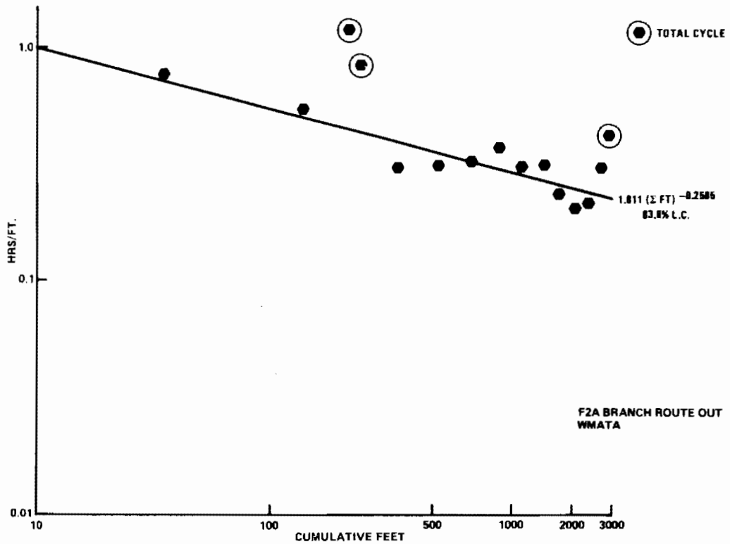
Figure 5-5. Rate of Advance vs Cumulative Tunnel Length
