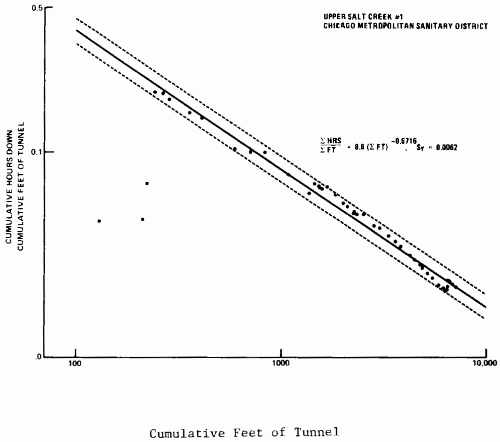
Figure 6-3. Excavating Cutting Wheel Downtime for USC No. 1
